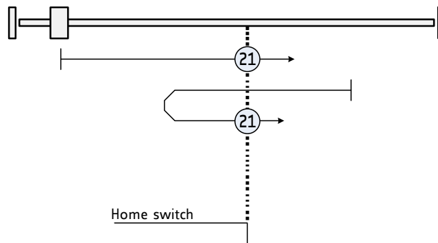
Figure 18: Homing Method 21
