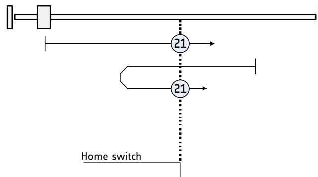
Figure 9: Homing Method 21
