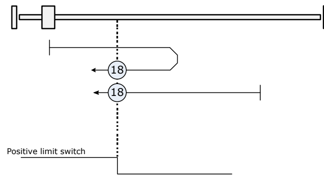
Figure 7: Homing Method 18
