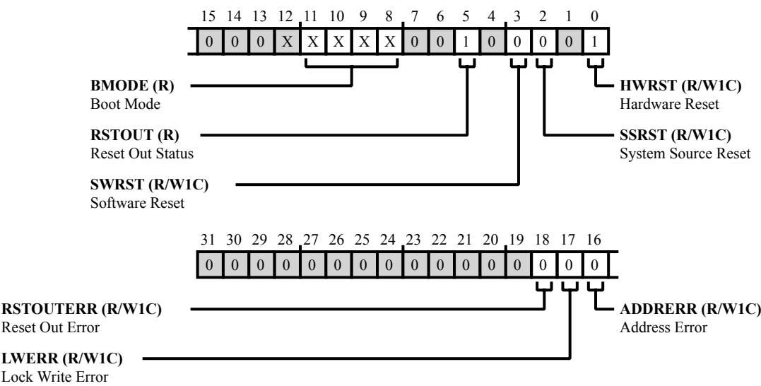
Figure 41-10: RCU_STAT Register Diagram
