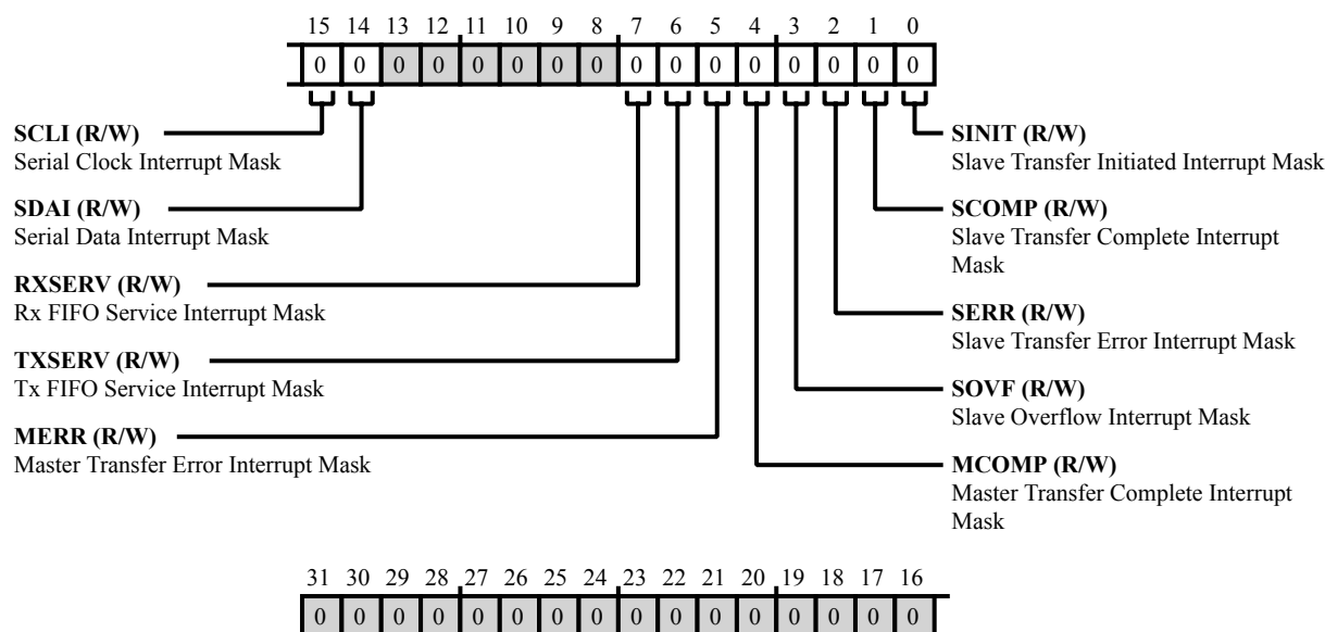
Figure 26-18: TWI_IMSK Register Diagram
