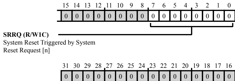
Figure 41-9: RCU_SRRQSTAT Register Diagram
