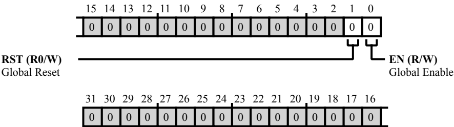
Figure 45-6: SWU_GCTL Register Diagram
