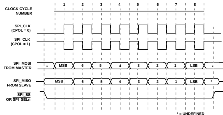
Figure 28-2: SPI Transfer Protocol for CPHA=0
