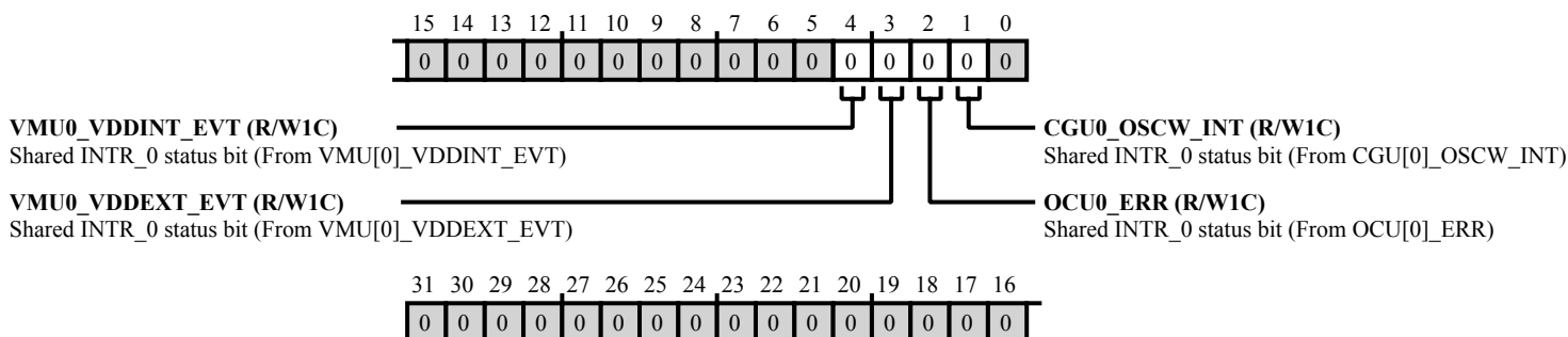
Figure 43-14: SYSBLK_SISTAT0 Register Diagram
