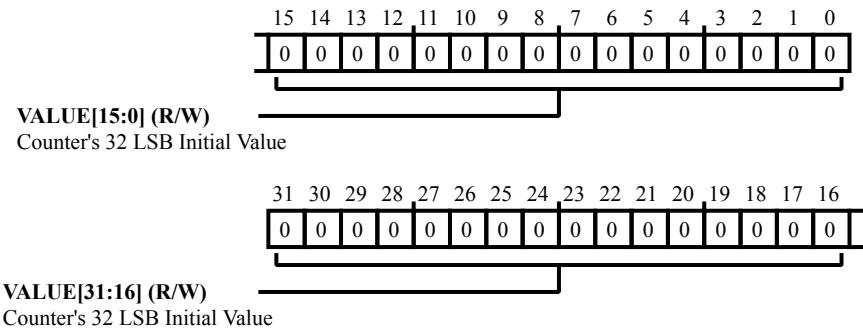
Figure 6-18: CGU_TSVALUE0 Register Diagram
