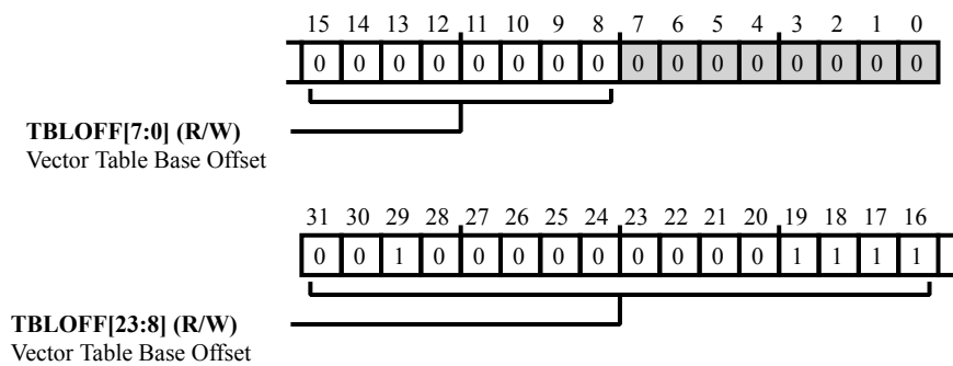
Figure 43-9: SYSBLK_M0_VTOR Register Diagram
