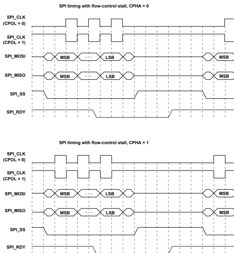
Figure 28-6: SPI Flow Control Timing in Master Mode.
