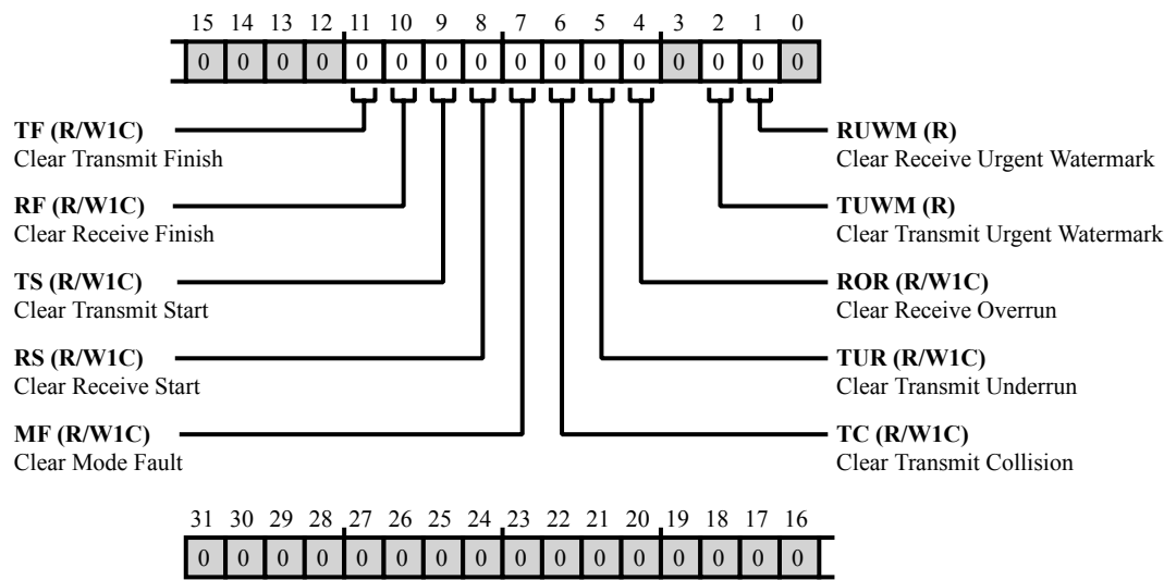
Figure 28-17: SPI_ILAT_CLR Register Diagram
