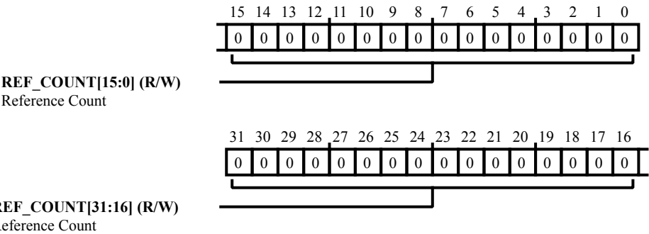
Figure 7-9: OCU_REFCNT Register Diagram
