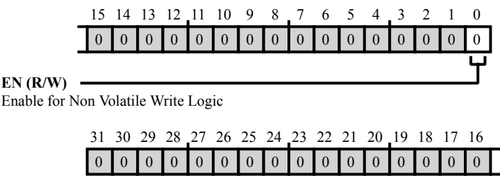
Figure 43-38: PADS_NVWR_RSTCTL Register Diagram
