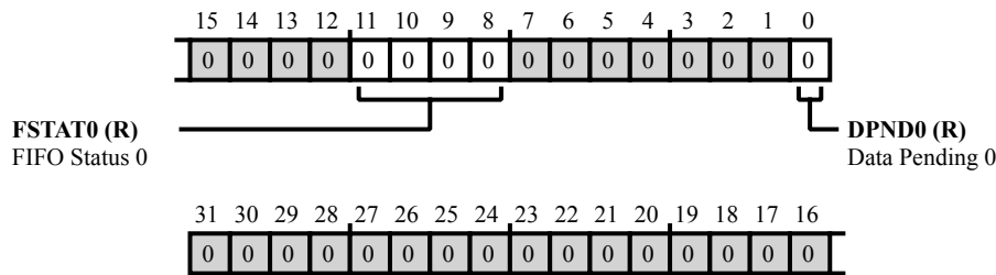
Figure 31-20: DACC_STAT Register Diagram
