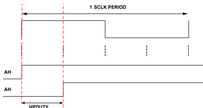
Figure 24-20: Heightened-Precision Steps in a Single SCLK Period
