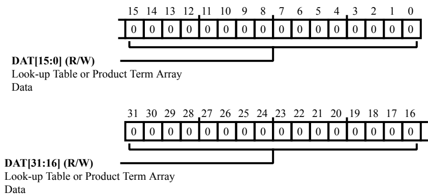
Figure 37-12: LBA0_BLK[n]_FN2 Register Diagram
