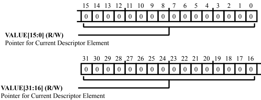
Figure 17-12: DMA_DSCPTR_CUR Register Diagram
