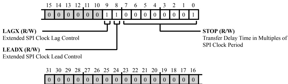
Figure 28-15: SPI_DLY Register Diagram
