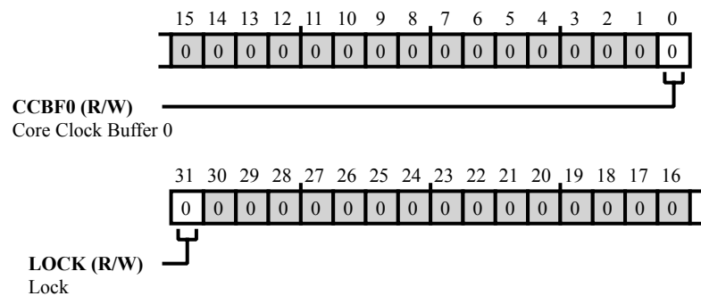
Figure 6-4: CGU_CCBF_DIS Register Diagram
