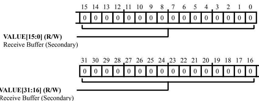
Figure 29-35: SPORT_RXSEC_A Register Diagram
