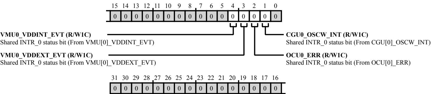
Figure 43-60: SYSBLK_SISTAT0 Register Diagram
