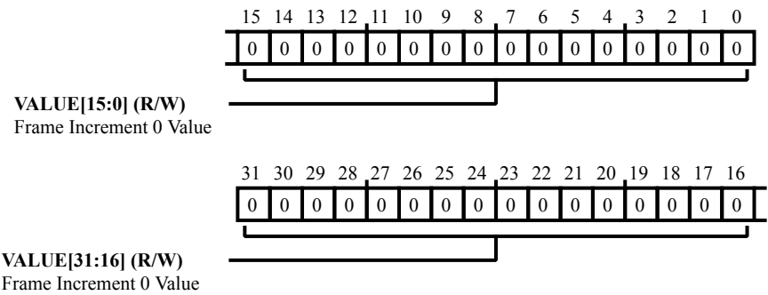
Figure 30-57: ADCC_FRINC0 Register Diagram
