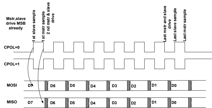
Figure 28-11: SPI Transfer Protocol in Fast Mode for SPI_CTL.CPHA = 0
