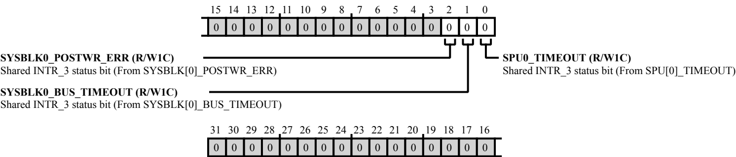
Figure 43-26: SYSBLK_SISTAT3 Register Diagram
