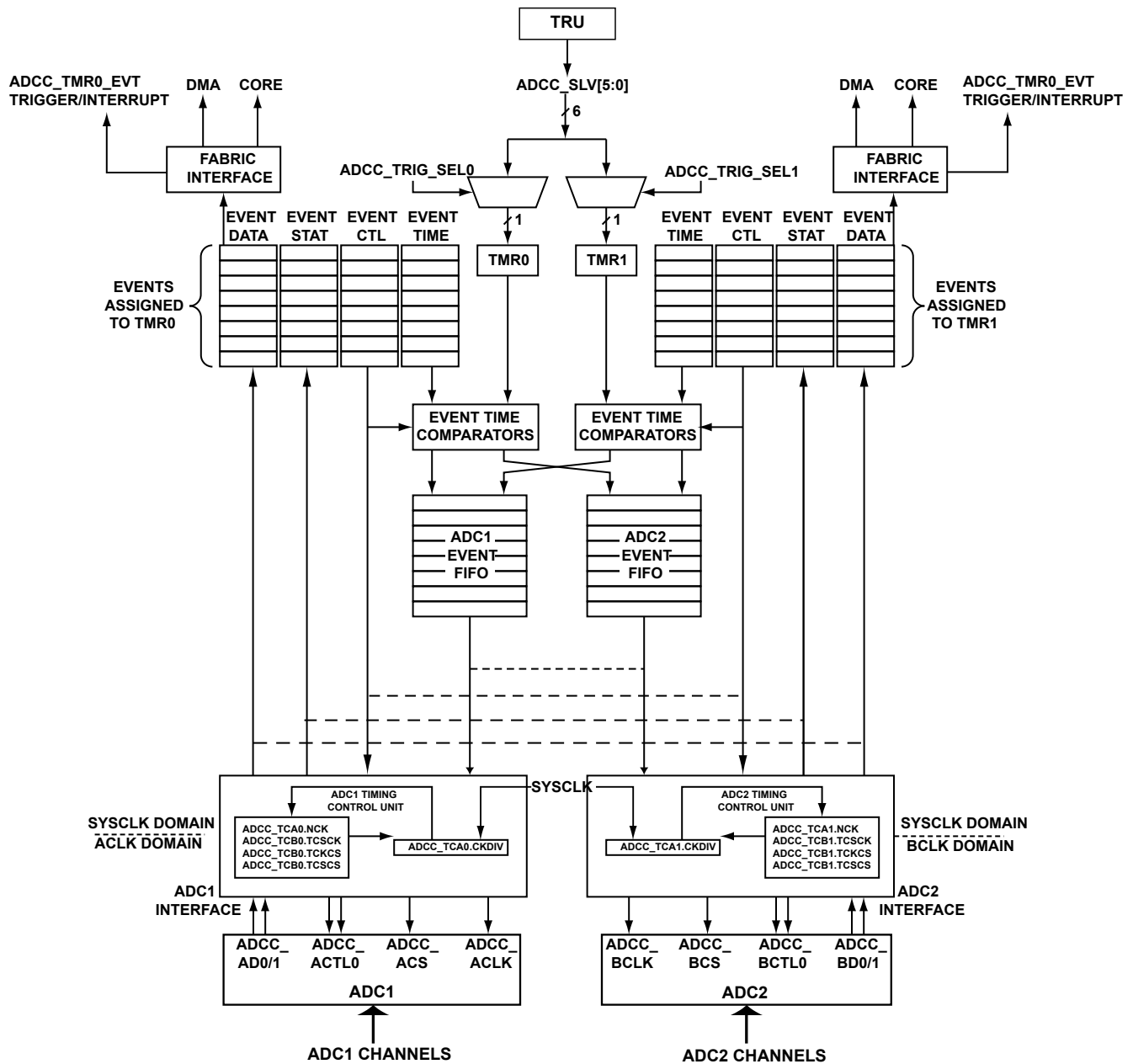
Figure 30-5: ADCC1 Block Diagram
