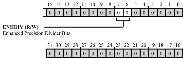
Figure 24-79: PWM_DH0_HP Register Diagram
