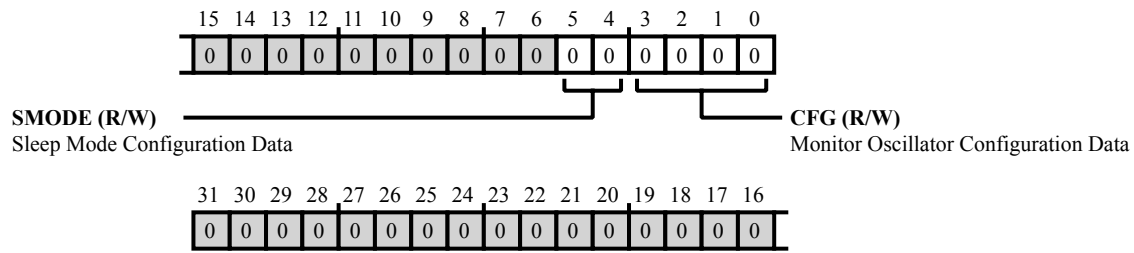
Figure 43-37: PADS_MONOSC_CFG Register Diagram
