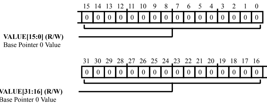
Figure 30-25: ADCC_BPTR0 Register Diagram
