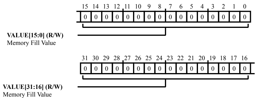
Figure 16-9: CRC_FILLVAL Register Diagram
