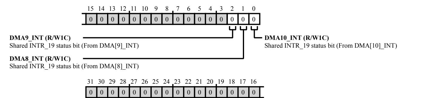
Figure 43-22: SYSBLK_SISTAT19 Register Diagram
