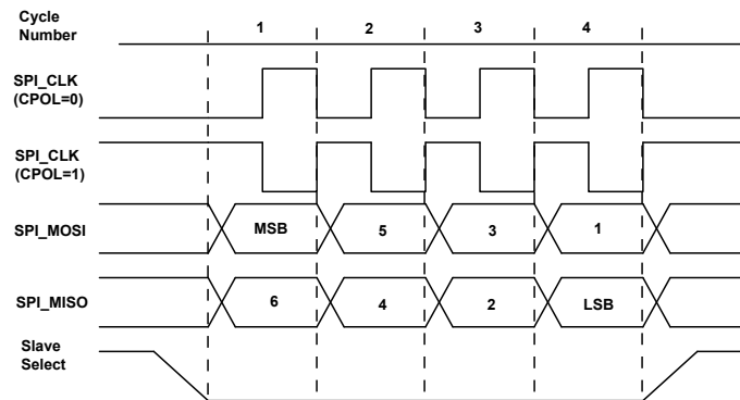
Figure 28-8: Dual I/O Mode Transfer Protocol for CPHA=0 , SOSI=1 , 8-Bit Transfer, LSBF=0 .
