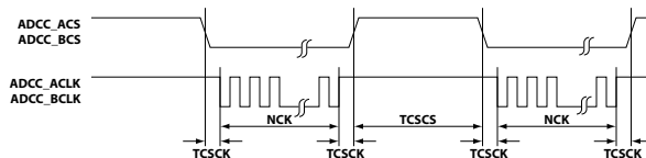
Figure 30-6: ADCC Clock Signal and Chip Select Signal Description
