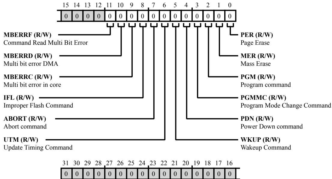
Figure 14-12: FLC_IMSK Register Diagram
