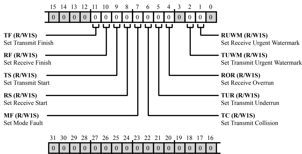
Figure 28-20: SPI_IMSK_SET Register Diagram
