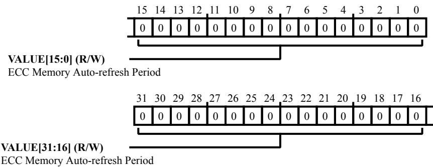
Figure 38-11: MBOX_PORT1_RFRPER Register Diagram
