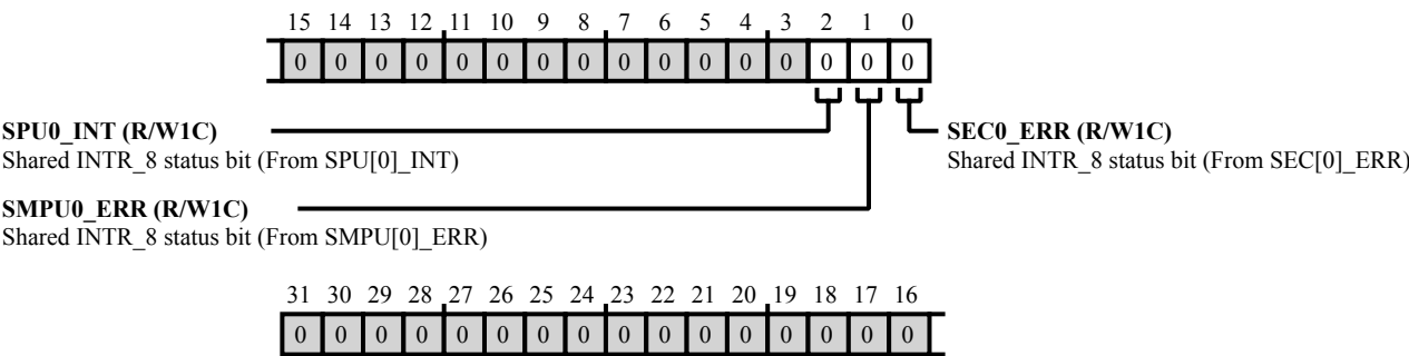
Figure 43-76: SYSBLK_SISTAT8 Register Diagram
