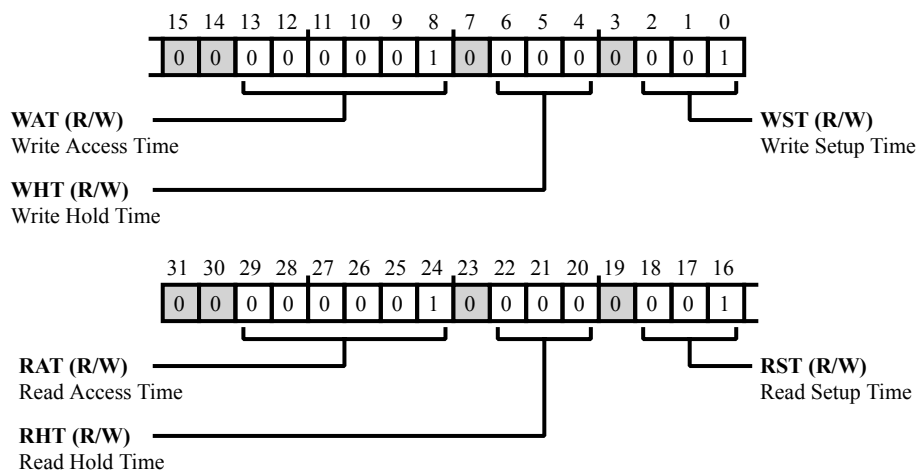
Figure 13-15: SMC_B0TIM Register Diagram
