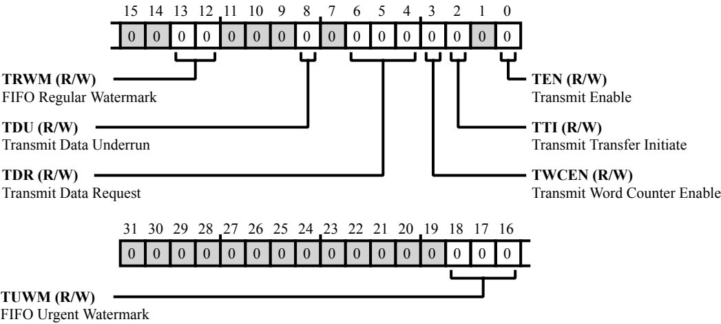
Figure 28-30: SPI_TXCTL Register Diagram
