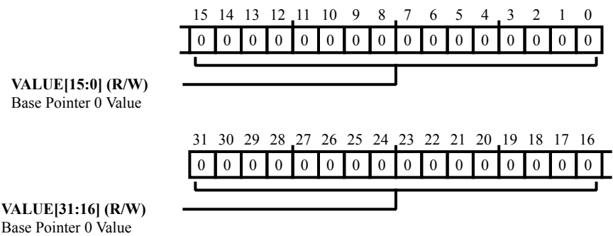
Figure 31-6: DACC_BPTR0 Register Diagram
