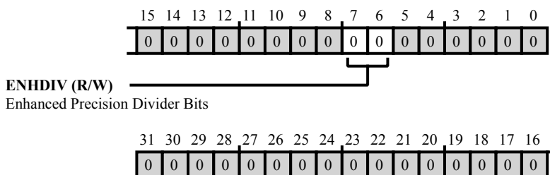
Figure 24-39: PWM_AL0_HP Register Diagram
