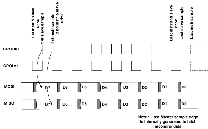
Figure 28-12: SPI Transfer Protocol in Fast Mode for SPI_CTL.CPHA = 1
