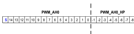
Figure 24-21: Duty Cycle Notation for Heightened-Precision Edge Placement
