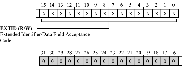
Figure 27-38: CAN_MB[nn]_ID0 Register Diagram
