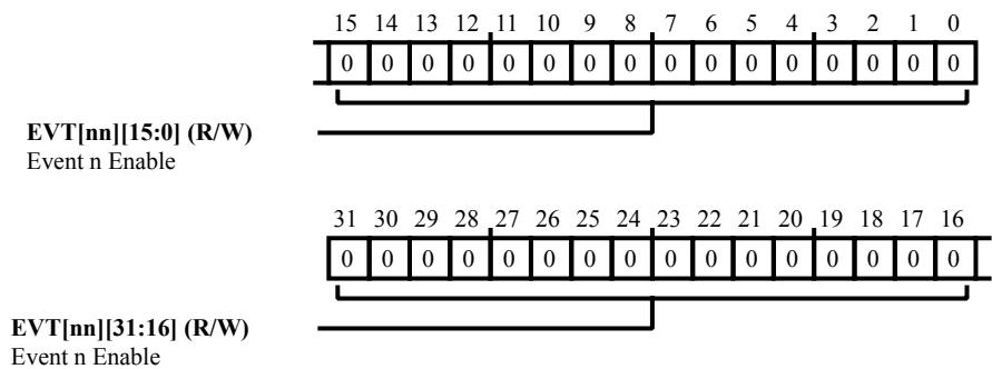
Figure 30-51: ADCC_EVTEN_SET Register Diagram
