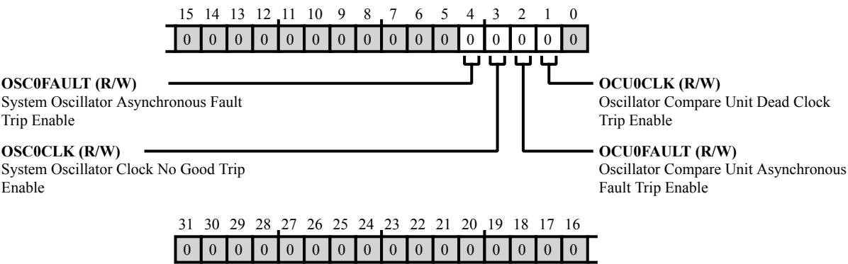
Figure 43-46: PADS_VMU_TRIPEN Register Diagram
