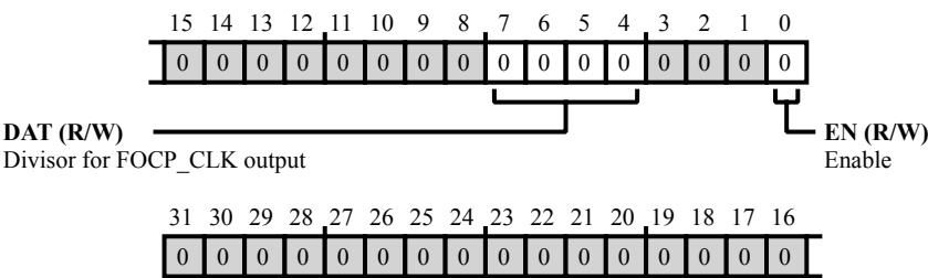
Figure 43-36: PADS_FOCP_DIV Register Diagram
