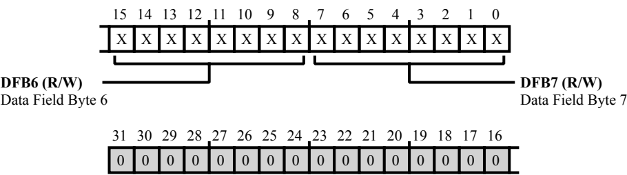
Figure 27-34: CAN_MB[nn]_DATA0 Register Diagram
