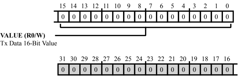
Figure 26-28: TWI_TXDATA16 Register Diagram
