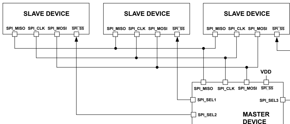
Figure 28-7: Single-Master, Multiple-Slave Configuration
