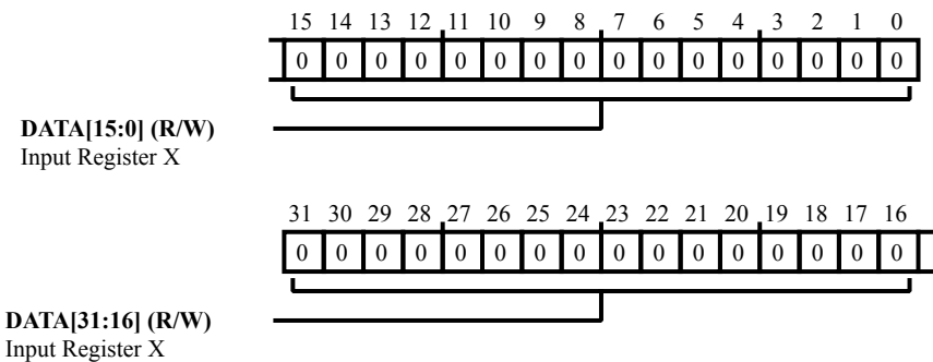
Figure 35-6: MATH_ATAN2F_X Register Diagram
