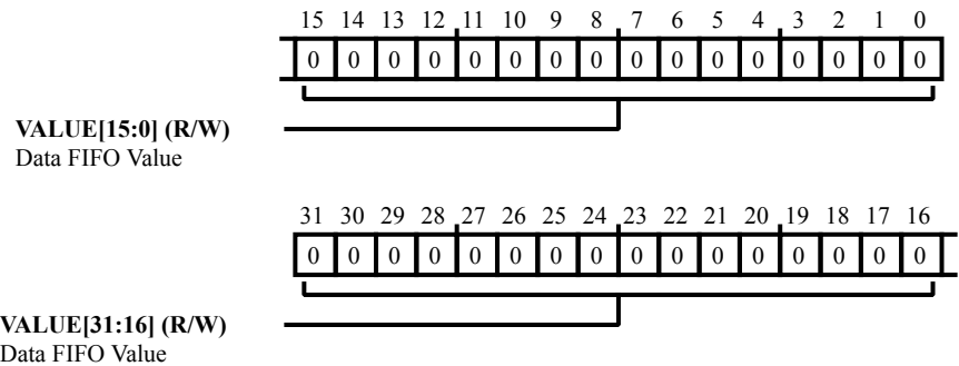
Figure 16-8: CRC_DFIFO Register Diagram
