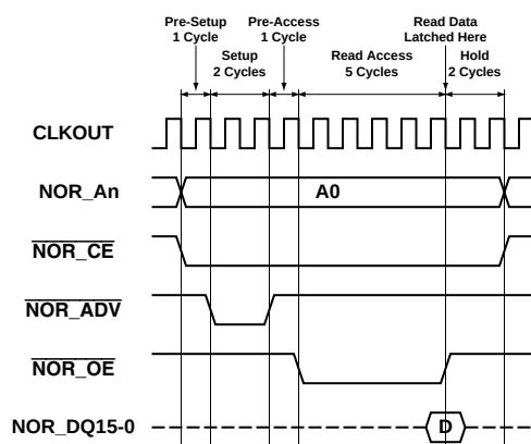
Figure 13-7: Asynchronous Flash Read with Pre-Setup and Pre-Access Cycles
