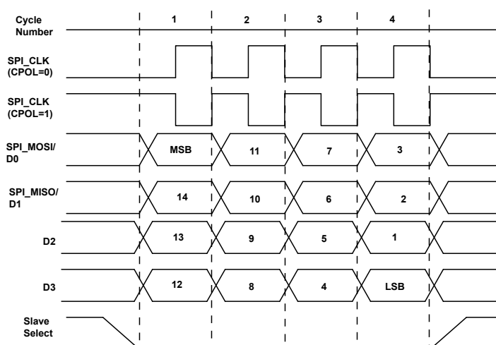
Figure 28-10: Quad Mode Timing for CPHA=0 , SOSI=1 , 16-Bit Transfer, LSBF=0 .
