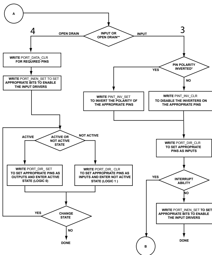
Figure 18-5: GPIO Programming Model Flow (Part 2)
