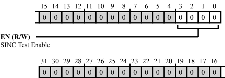
Figure 43-13: SYSBLK_SINC_TEST Register Diagram
