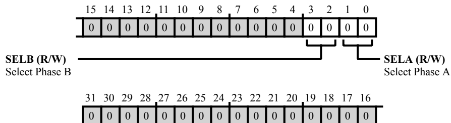
Figure 43-12: SYSBLK_ROT_UPDN_CFG Register Diagram
