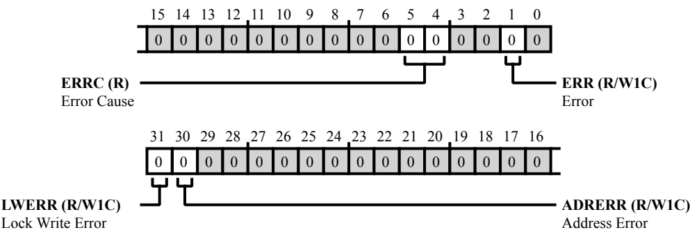
Figure 10-15: SEC_GSTAT Register Diagram
