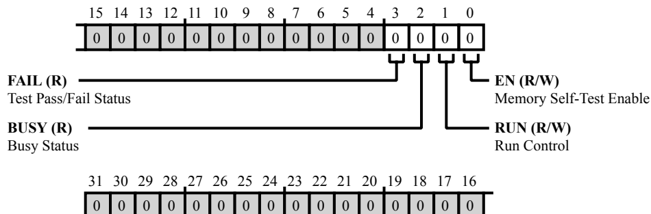
Figure 43-10: SYSBLK_MEMST_CTL Register Diagram
