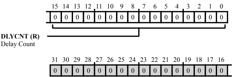
Figure 30-48: ADCC_EVSTAT[nn] Register Diagram
