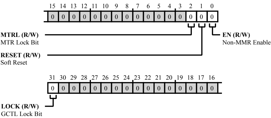
Figure 11-4: TRU_GCTL Register Diagram
