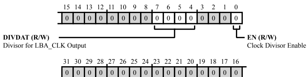
Figure 37-19: LBA0_CLK_CTL Register Diagram
