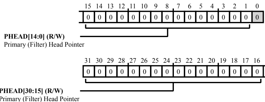
Figure 34-22: SINC_PHEAD1 Register Diagram
