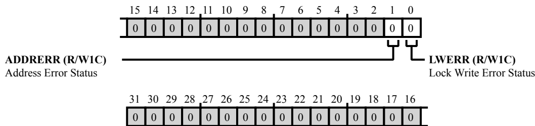
Figure 11-7: TRU_STAT Register Diagram
