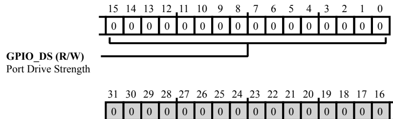
Figure 43-40: PADS_PORT[n]_DS Register Diagram
