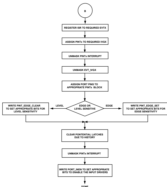
Figure 18-6: GPIO Programming Model Flow (Part 3)
