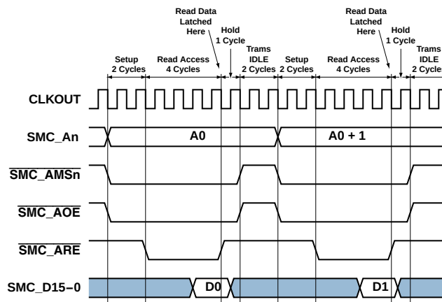
Figure 13-3: Asynchronous SRAM Read with IDLE Transition
