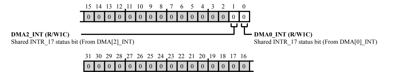
Figure 43-20: SYSBLK_SISTAT17 Register Diagram
