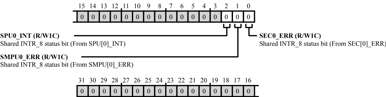
Figure 43-30: SYSBLK_SISTAT8 Register Diagram
