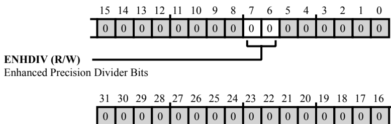
Figure 24-52: PWM_BLO_HP Register Diagram
