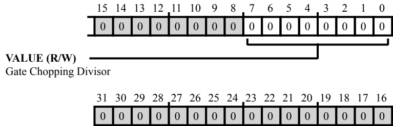
Figure 24-67: PWM_CHOPCFG Register Diagram
