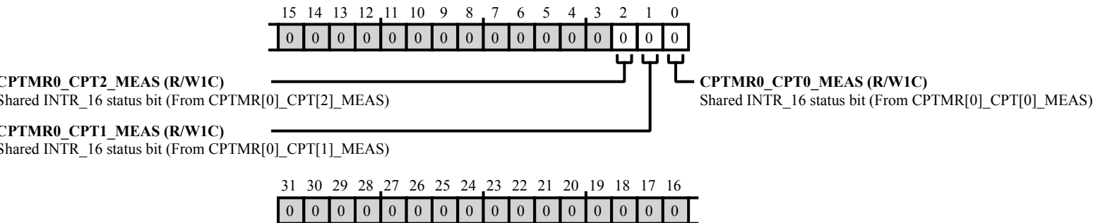
Figure 43-19: SYSBLK_SISTAT16 Register Diagram
