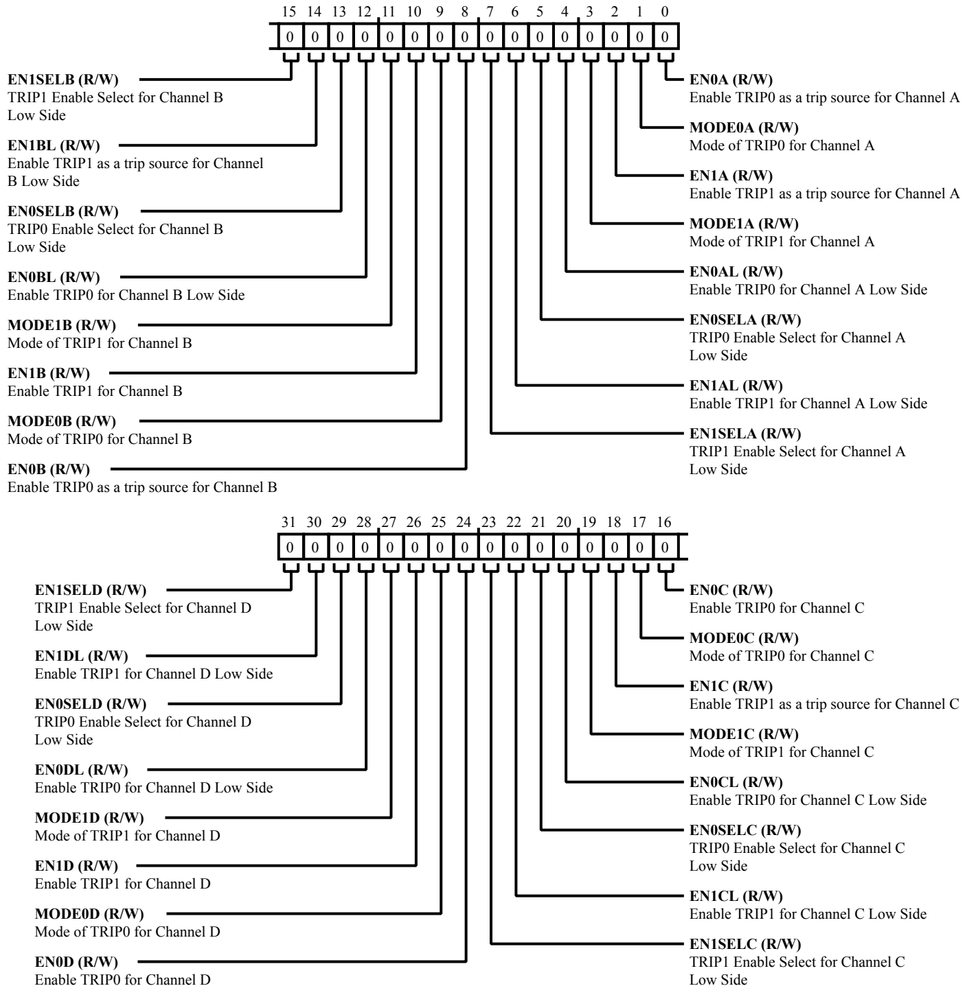
Figure 24-104: PWM_TRIPCFG Register Diagram
