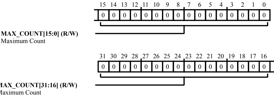
Figure 7-7: OCU_MAXCNT Register Diagram
