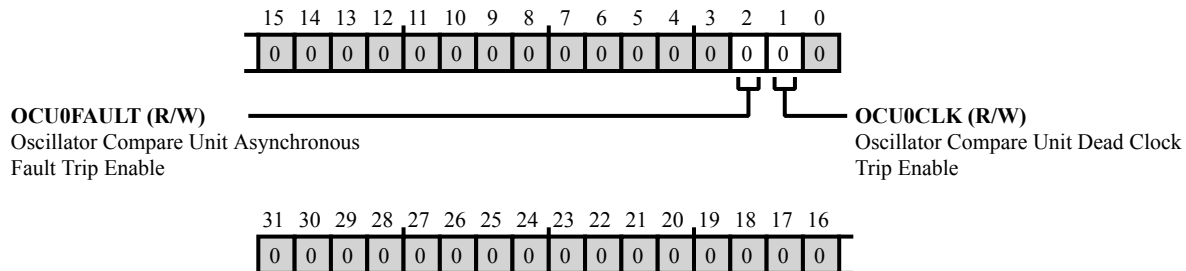
Figure 43-49: SYSBLK_CLKNG_TRIPEN Register Diagram
