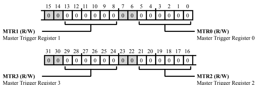
Figure 11-5: TRU_MTR Register Diagram
