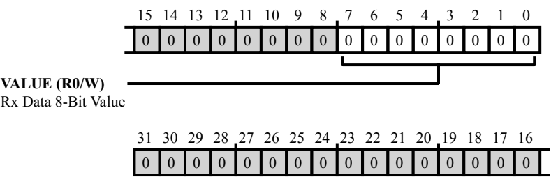
Figure 26-24: TWI_RXDATA8 Register Diagram
