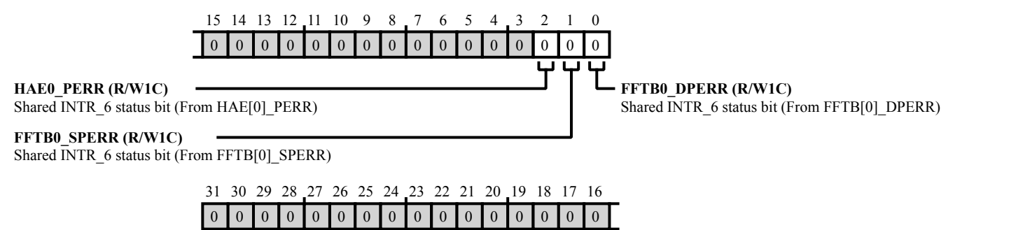
Figure 43-28: SYSBLK_SISTAT6 Register Diagram
