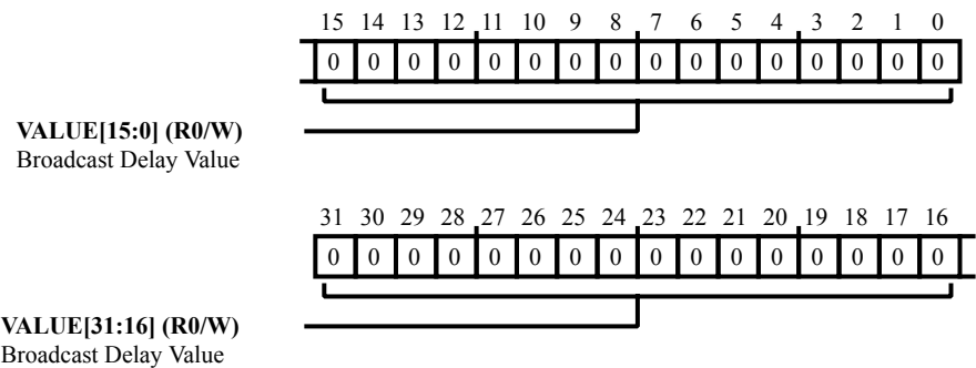
Figure 19-10: TIMER_BCAST_DLY Register Diagram
