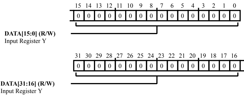
Figure 35-7: MATH_ATAN2F_Y Register Diagram
