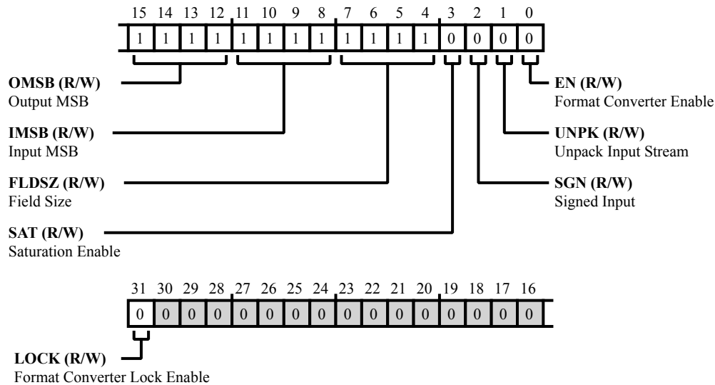
Figure 40-6: FFTB_FMTCTL Register Diagram
