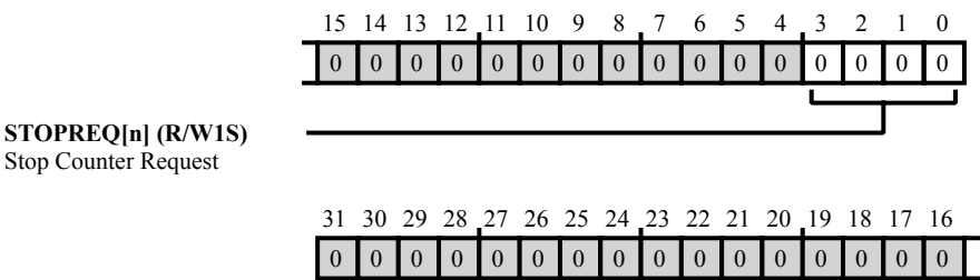
Figure 12-16: TTU_STOP Register Diagram
