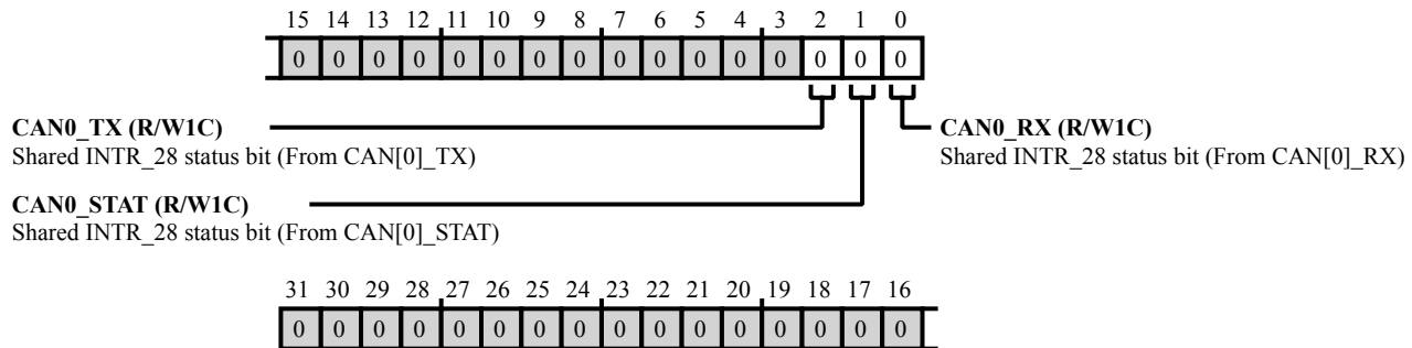
Figure 43-25: SYSBLK_SISTAT28 Register Diagram
