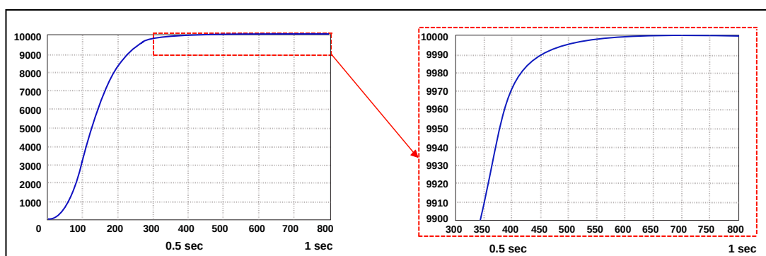
Figure 33-5: Fundamental and Harmonic Values - Settling Times
