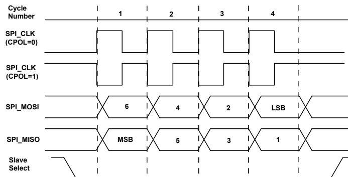
Figure 28-9: Dual I/O Mode Transfer Protocol for CPHA=1 , SOSI=0 , 8-Bit Transfer, LSBF=0 .
