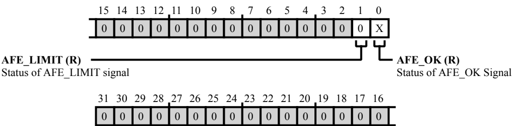
Figure 43-32: SYSBLK_SYSSTAT Register Diagram
