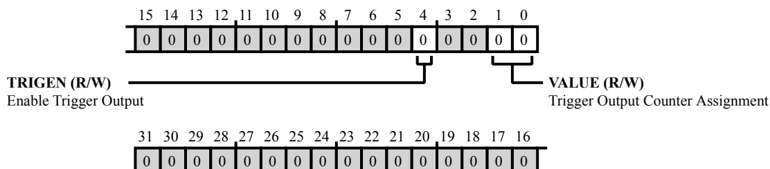
Figure 12-11: TTU_DGRP[m] Register Diagram
