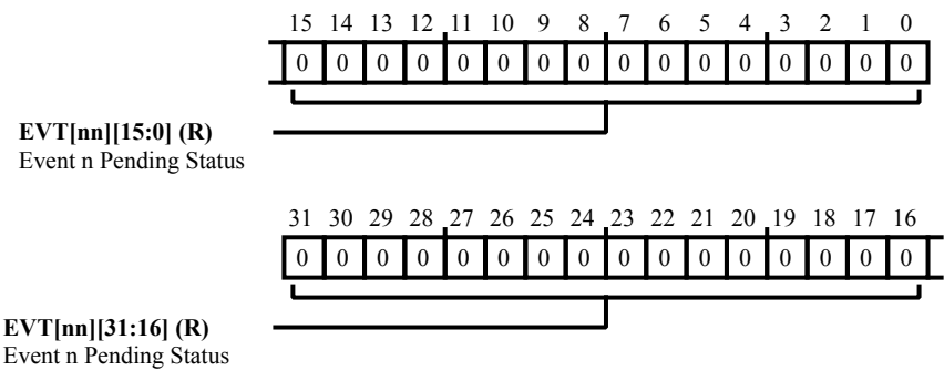
Figure 30-41: ADCC_EPND Register Diagram
