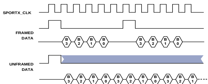
Figure 29-6: Framed versus Unframed Data Stream
