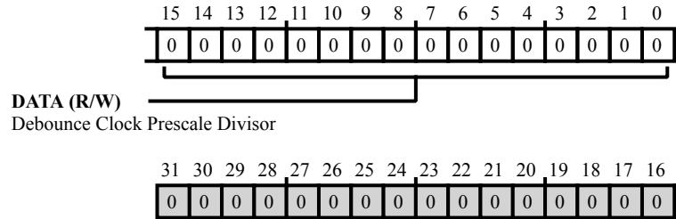
Figure 43-35: PADS_DBC_PRESCALE Register Diagram
