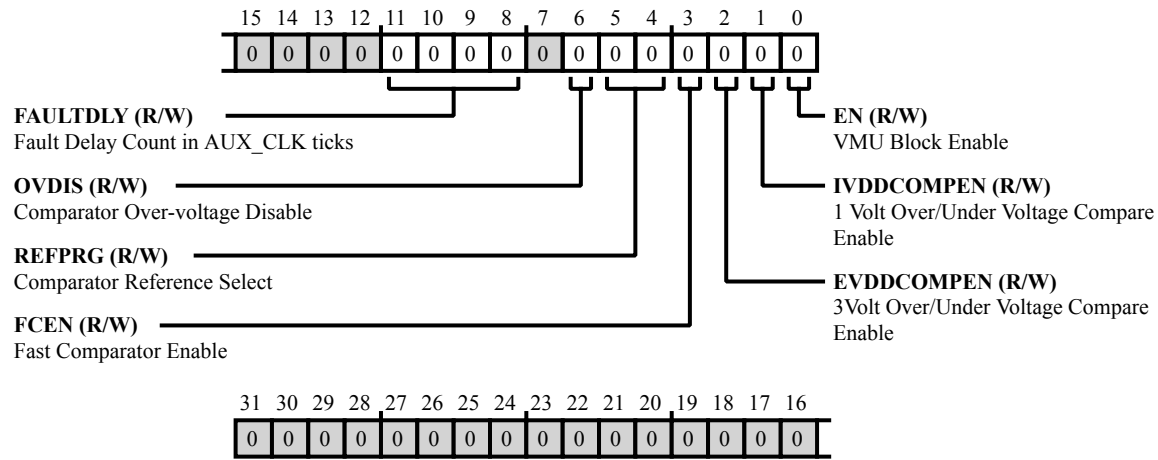
Figure 43-90: PADS_VMU_CTL Register Diagram
