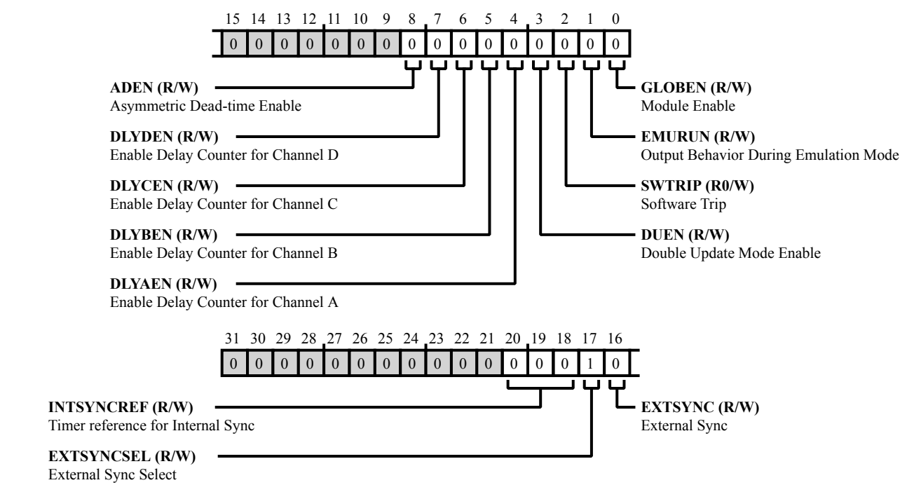
Figure 24-76: PWM_CTL Register Diagram
