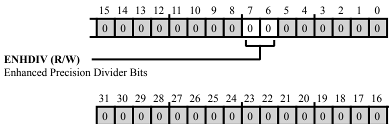
Figure 24-48: PWM_BH1_HP Register Diagram
