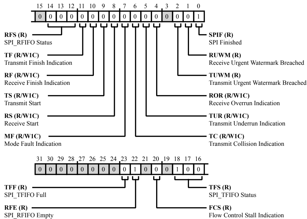
Figure 28-26: SPI_STAT Register Diagram
