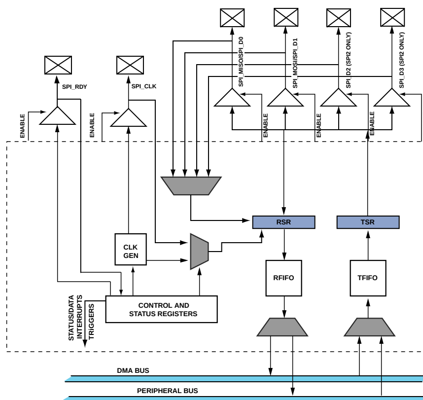
Figure 28-1: SPI Controller Block Diagram, Quad Mode
