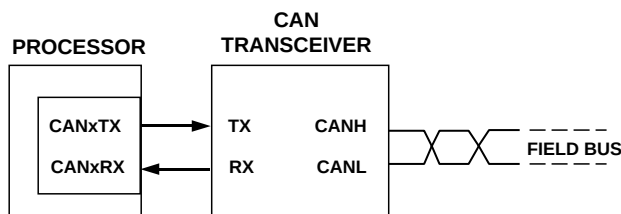
Figure 27-1: Representation of CAN Transceiver Interconnection
