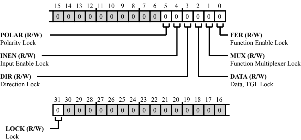
Figure 18-20: PORT_LOCK Register Diagram
