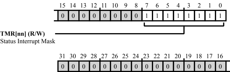
Figure 19-20: TIMER_STAT_IMSK Register Diagram
