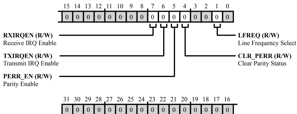
Figure 33-8: HAE_CFG0 Register Diagram
