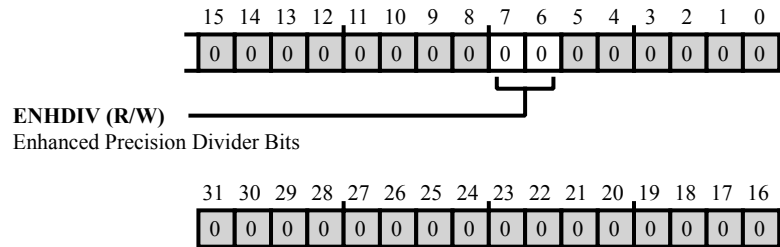
Figure 24-41: PWM_AL1_HP Register Diagram
