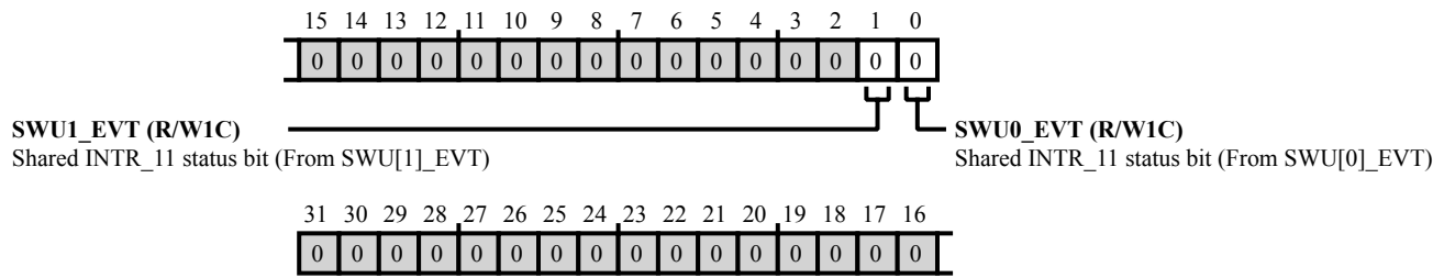
Figure 43-16: SYSBLK_SISTAT11 Register Diagram
