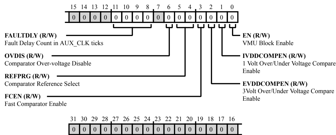
Figure 43-44: PADS_VMU_CTL Register Diagram
