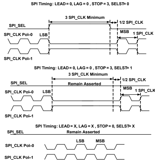
Figure 28-5: SPI Timing with SPI_DLY.STOP Programming (Independent of SPI_CTL.CPHA Setting)
