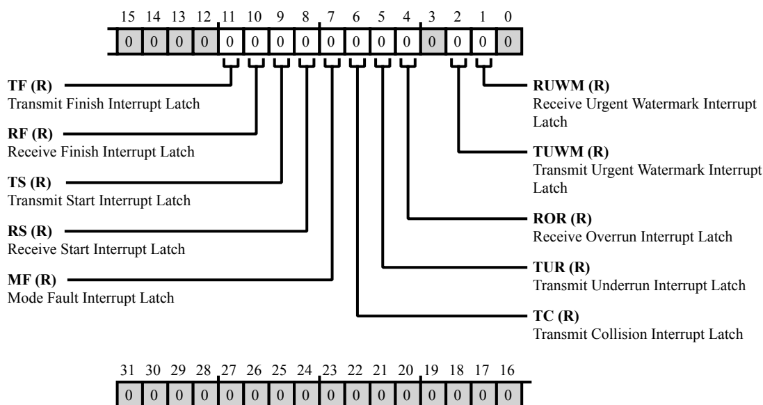
Figure 28-16: SPI_ILAT Register Diagram
