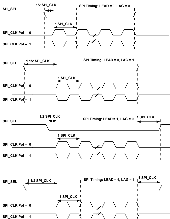
Figure 28-4: SPI Timing with Lead and Lag Programming (Independent of SPI\_CTL.CPHA Setting)
