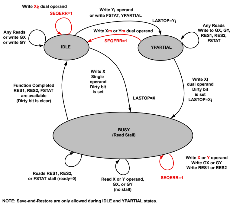
Figure 35-3: MATH Unit Register Operation Sequence
