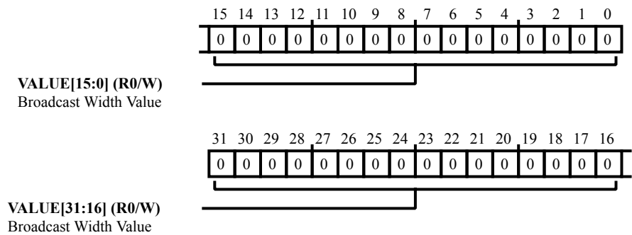
Figure 19-12: TIMER_BCAST_WID Register Diagram
