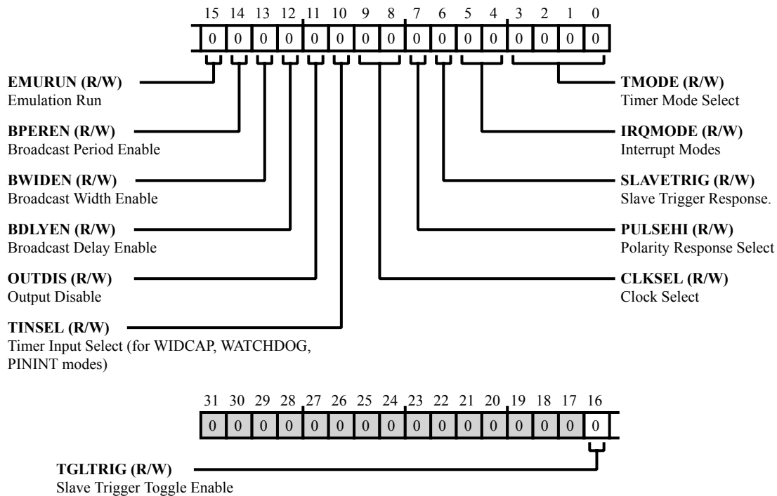
Figure 19-24: TIMER_TMR[n]_CFG Register Diagram
