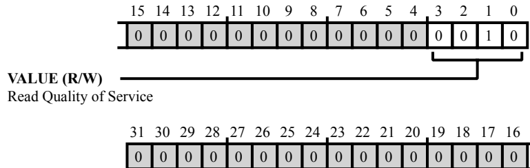
Figure 5-7: SCB_M4_RQOS Register Diagram
