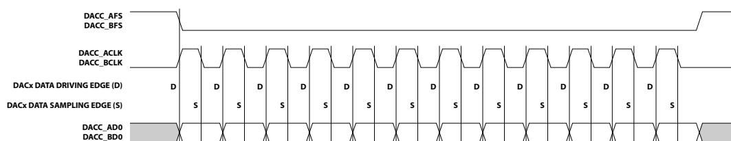
Figure 31-1: DACC Signals
