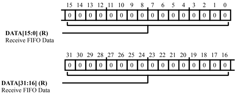
Figure 28-21: SPI_RFIFO Register Diagram
