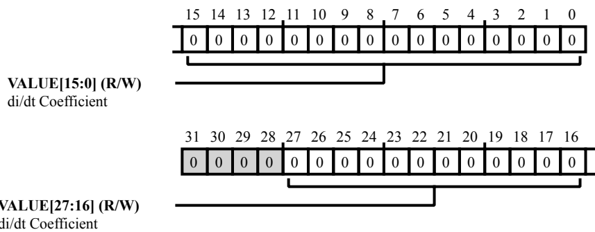
Figure 33-13: HAE_DIDT_COEF Register Diagram
