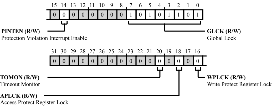
Figure 8-6: SPU_CTL Register Diagram
