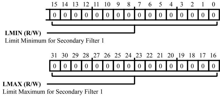
Figure 34-14: SINC_LIMIT1 Register Diagram
