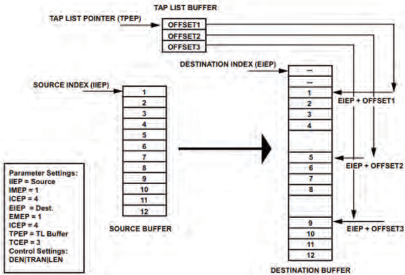
Figure 4-7. Scatter DMA (Writes)
