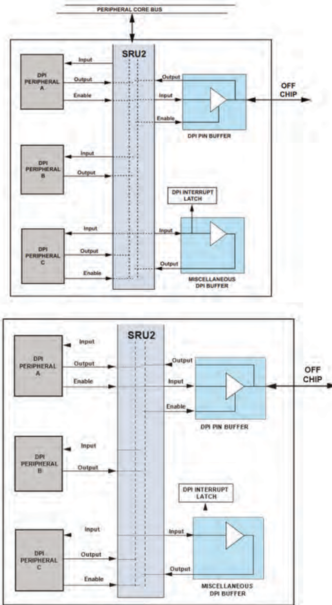
Figure 8-2. DPI Functional Block Diagram
