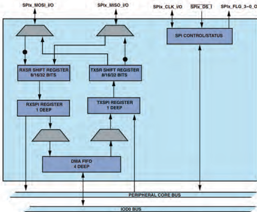
Figure 14-1. SPI Block Diagram
