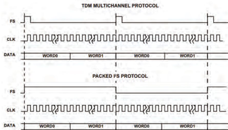
Figure 9-6. Packed I 2 S vs. TDM Multichannel Protocols
