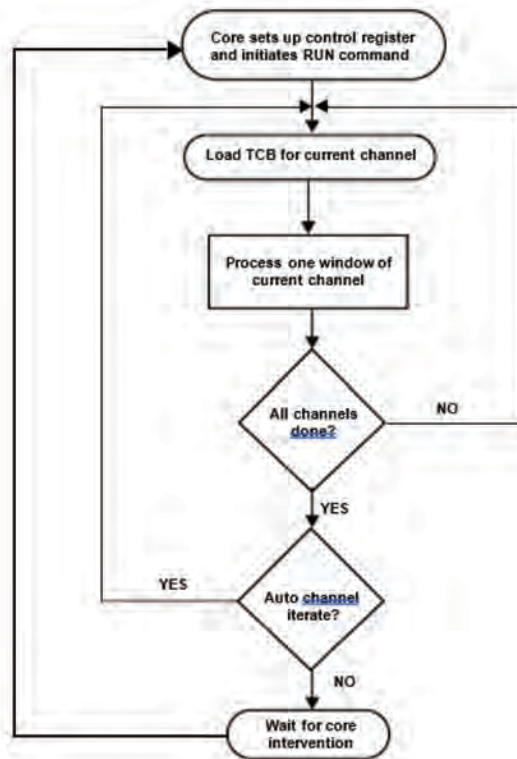
Figure 6-8. Wait for Core Intervention \geq Idle (If CAI Bit = 0)
