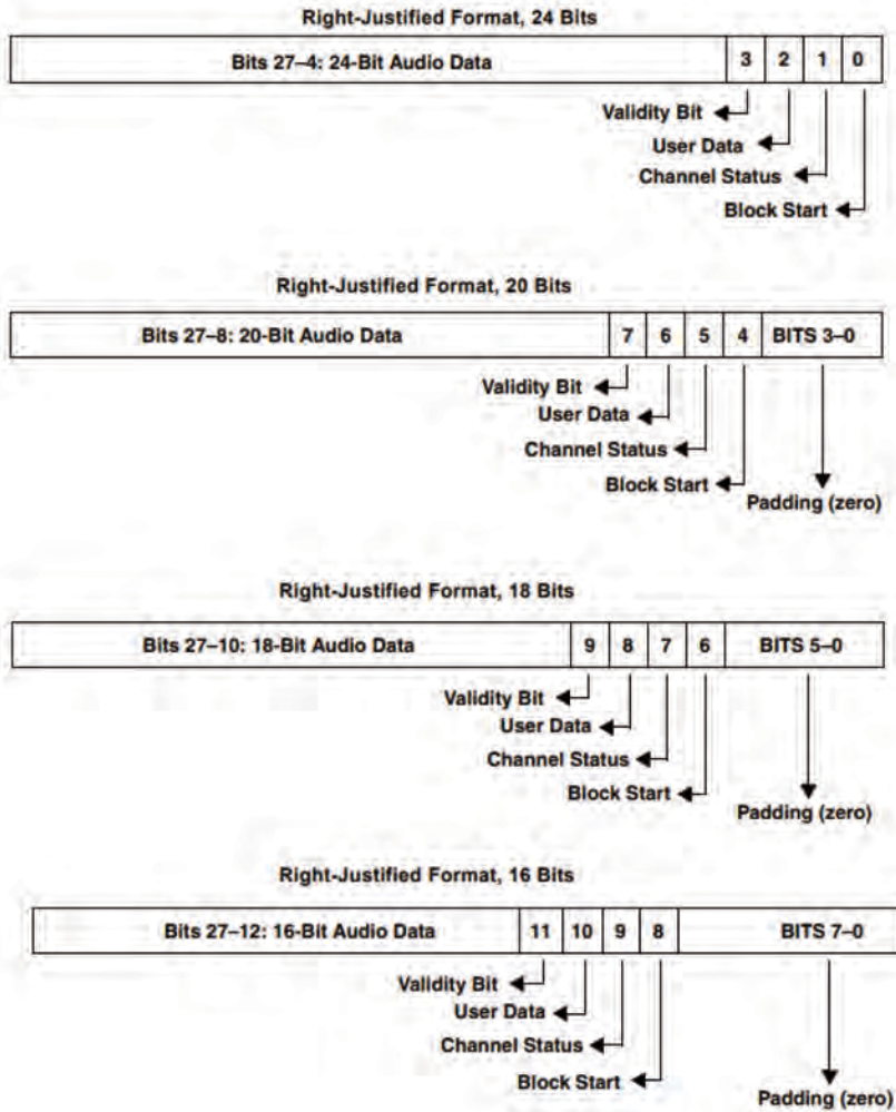
Figure 12-4. Right-Justified Formats
