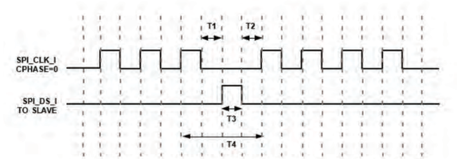
Figure 14-7. SPICLK Timing
