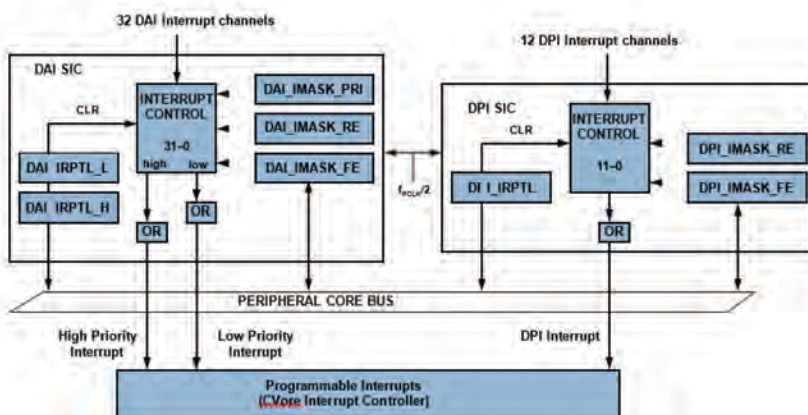
Figure 2-2. DAI/DPI System Interrupt Controllers (SIC)
