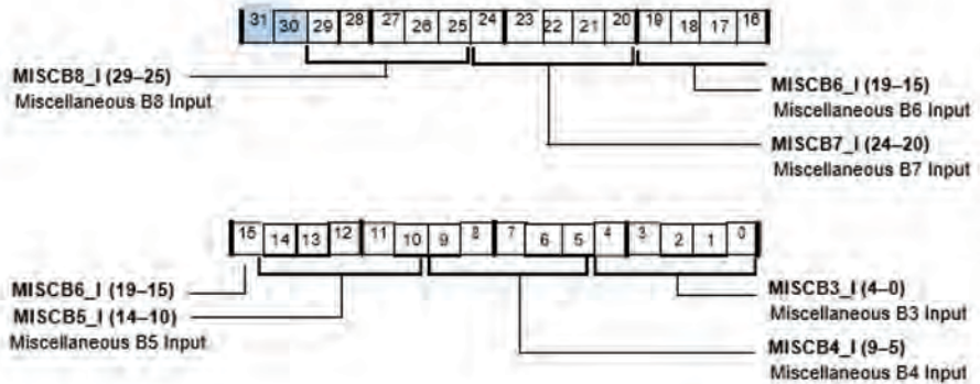
Figure A-47. SRU2_INPUT5 Register (RW)
