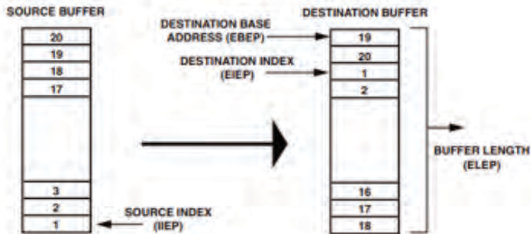
Figure 4-4. Circular Buffering Write DMA
