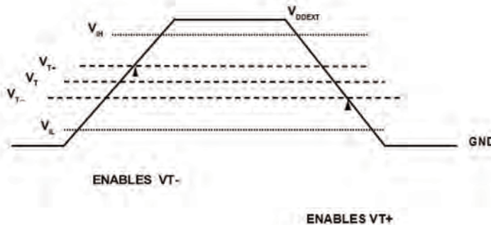
Figure 19-7. Input Pin Hysteresis
