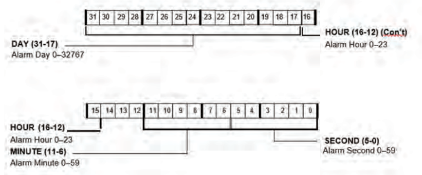
Figure A-10. RTC Alarm Register (RW)
