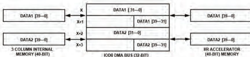
Figure 6-12. 32-Bit To 40-Bit Packing
