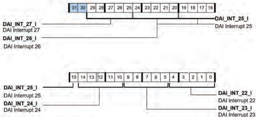
Figure A-35. SRU_EXT_MISCB Register (RW)
