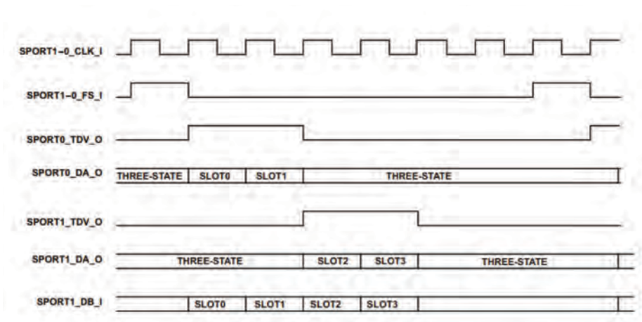
Figure 9-5. Multichannel Operation
