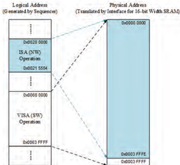
Figure 4-3. Translation of Logical to Physical L2 Memory Addressing
