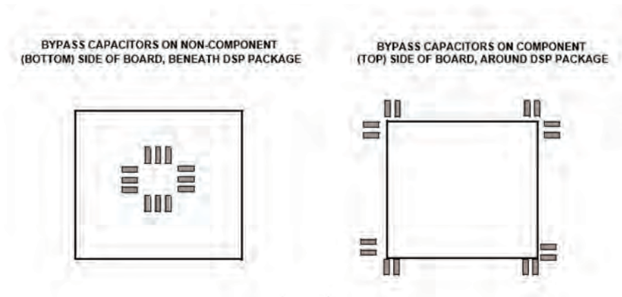
Figure 19-9. Bypass Capacitor Placement
