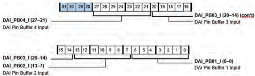
Figure A-29. SRU_PIN0 Register (RW)
