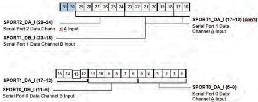
Figure A-17. SRU_DAT0 Register (RW)
