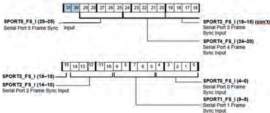
Figure A-24. SRU_FS0 Register (RW)
