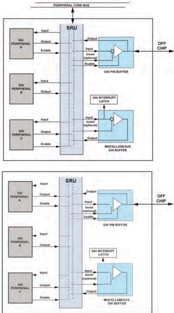
Figure 8-1. DAI Functional Block Diagram
