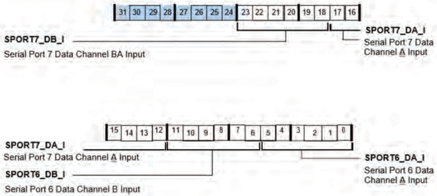
Figure A-23. SRU_DAT6 Register (RW)
