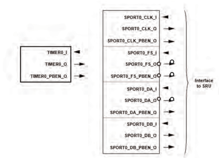
Figure 8-8. SRU Connections for Timer and SPORT0
