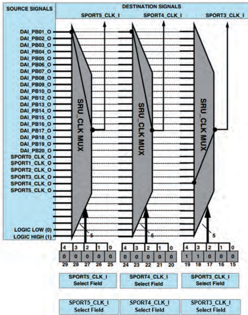
Figure 8-10. Example DAI SRU Group A Multiplexing (SRU_CLKx)
