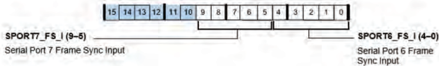
Figure A-28. SRU_FS4 Register (RW)
