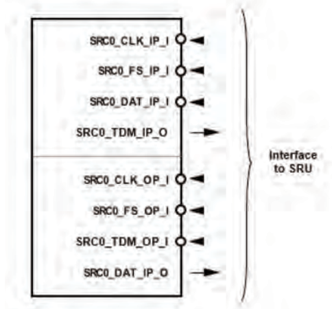
Figure 8-9. SRU Connections (no PBEN Signals)
