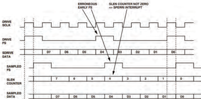
Figure 9-9. Frame Sync Error Detection
