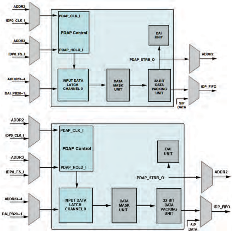
Figure 10-2. PDAP Port (Detail of IDP Channel 0)
