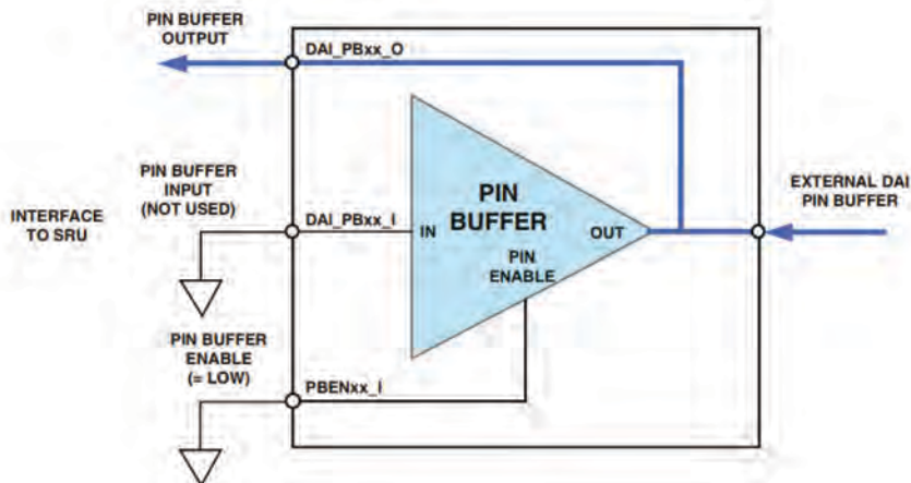
Figure 8-5. Pin Buffer as Input
