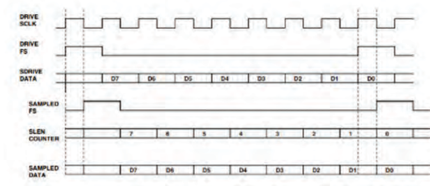
Figure 9-3. Frame Sync and Data Driven on Rising Edge
