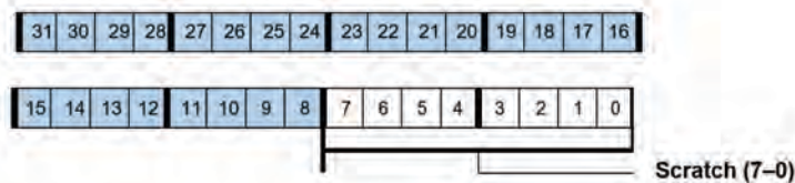
Figure A-56. UART0SCR Registers (RW)
