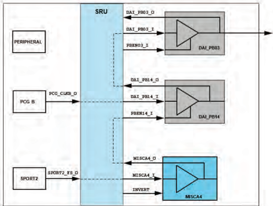
Figure 8-20. SRU Connection SPORT/PCG to MISC/DAI Pin Buffers
