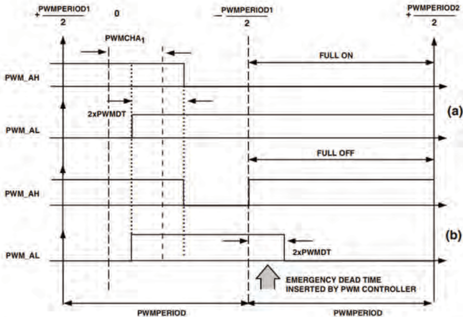
(a) — TRANSITION FROM NORMAL MODULATION TO FULL-ON, AT HALF-CYCLE BOUNDARY IN DOUBLE UPDATE MODE, WHERE NO ADDITIONAL DEAD TIME IS NEEDED. (b) TRANSITION FROM NORMAL MODULATION TO FULL-OFF, AT HALF-CYCLE BOUNDARY IN DOUBLE UPDATE MODE, WHERE ADDITIONAL DEAD TIME IS INSERTED BY THE PWM CONTROLLER
