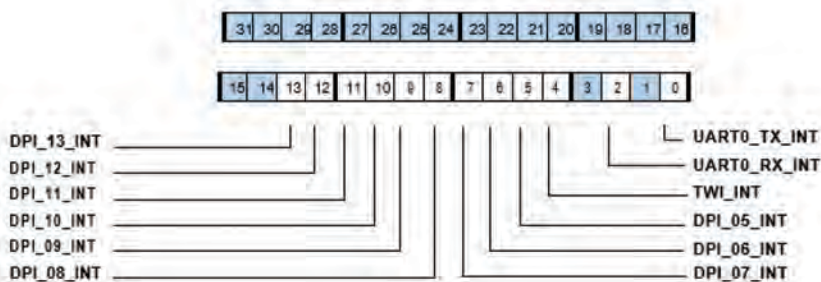
Figure A-6. DPI Interrupt Latch/Mask Register
