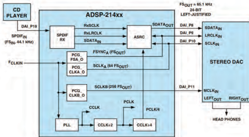
Figure 13-6. PCG Setup for I2S or Left-Justified DAI
