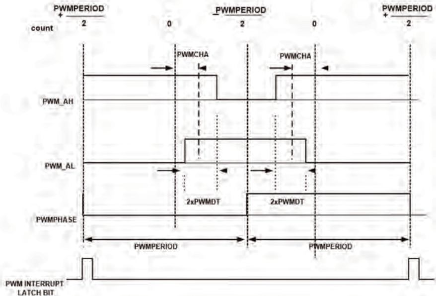
Figure 7-2. Center-Aligned Paired PWM in Single Update Mode, Low Polarity
