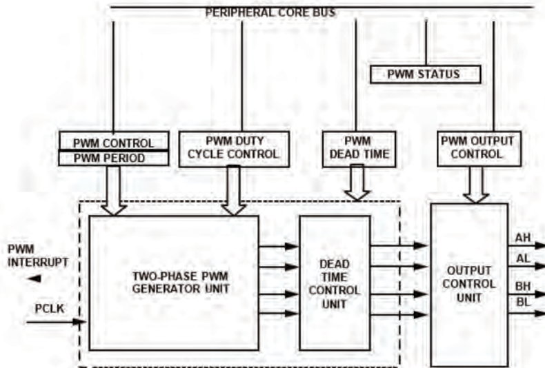
Figure 7-1. PWM Module Block Diagram
