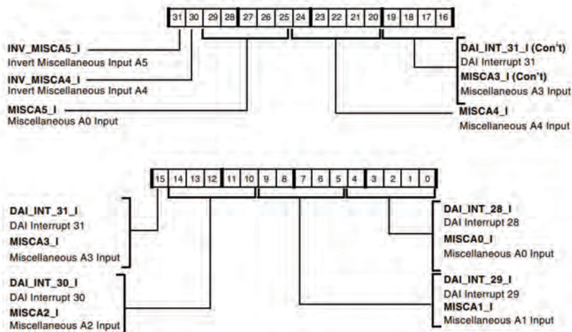
Figure A-34. SRU_EXT_MISCA Register (RW)
