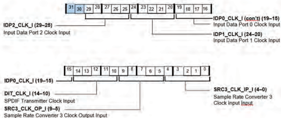
Figure A-13. SRU_CLK2 Register (RW)
