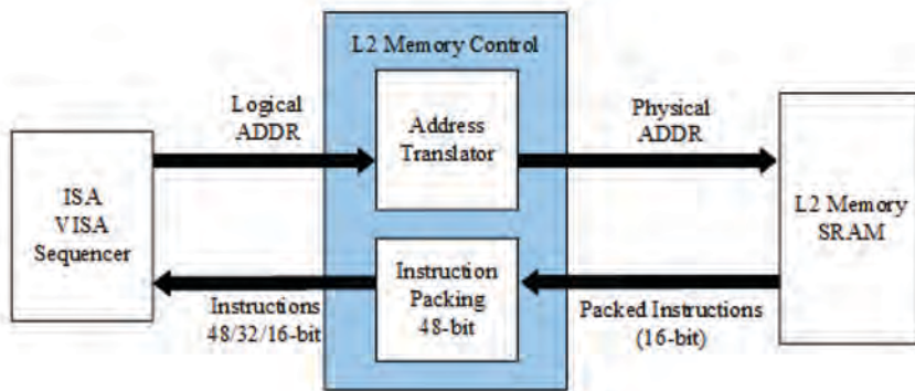
Figure 4-2. Logical vs. Physical Addresses
