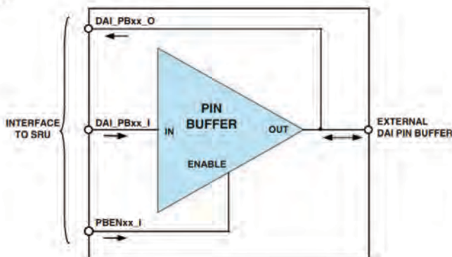
Figure 8-4. Pin Buffer Example
