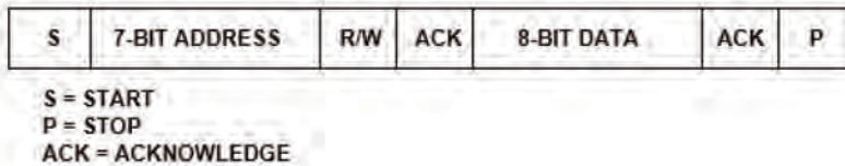
Figure 17-3. Standard Data Transfer
