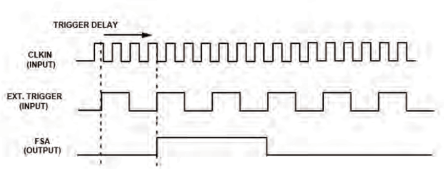
Figure 13-5. FS Output Synchronization With External Trigger Input
