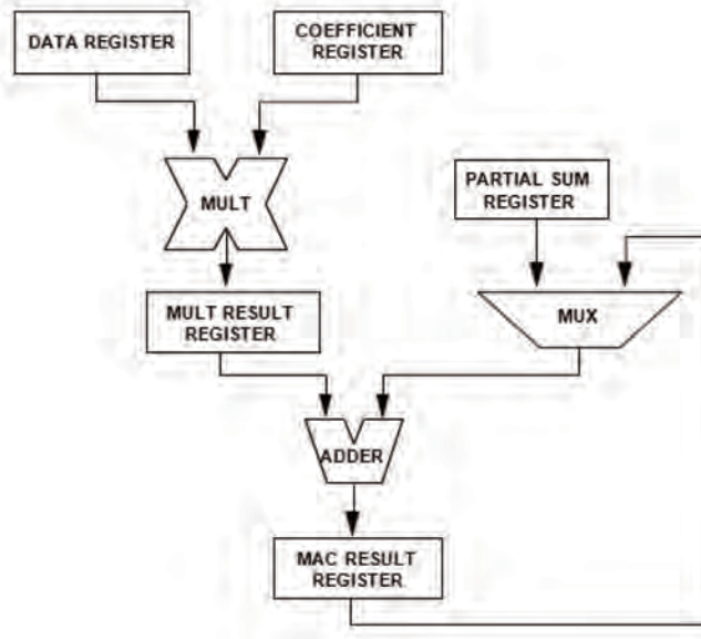
Figure 6-4. FIR MAC Unit
