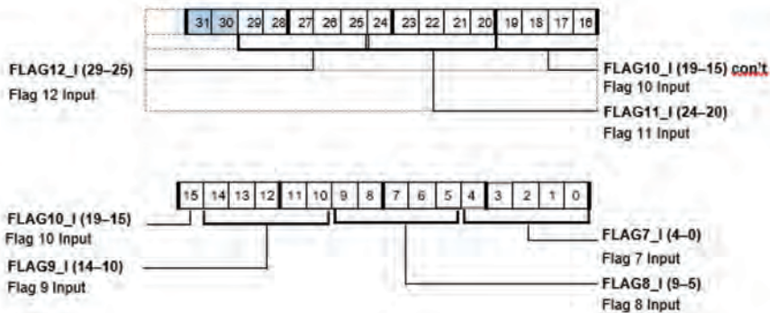
Figure A-45. SRU2_INPUT3 Register (RW)
