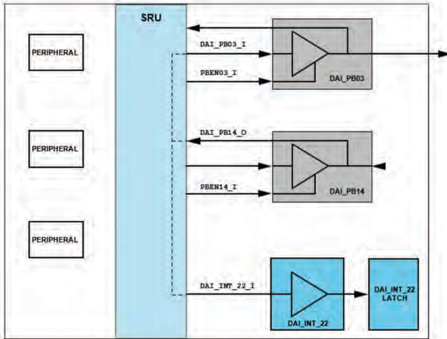
Figure 8-18. SRU Connection Between DAI Pin Buffers
