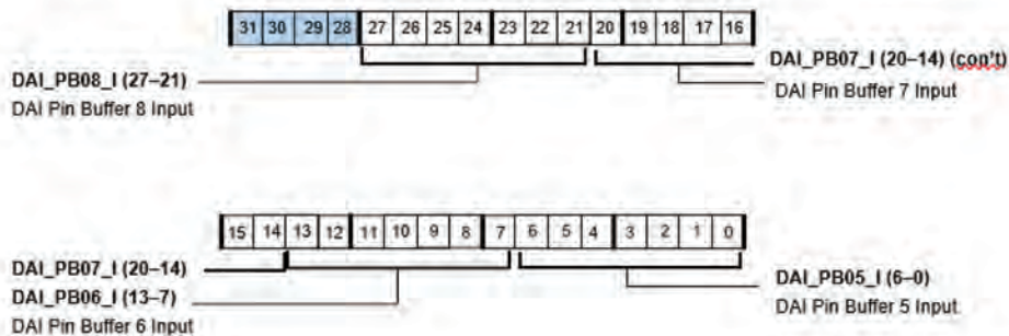
Figure A-30. SRU_PIN1 Register (RW)
