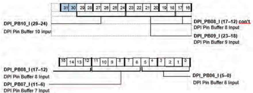
Figure A-49. SRU2_PIN1 Register
