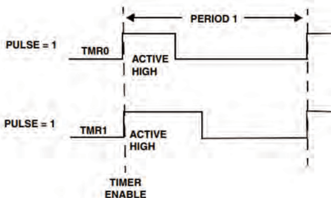
Figure 15-4. Timers with Pulses Aligned to Asserting Edge
