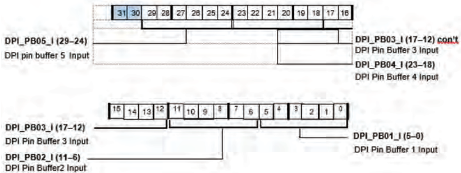
Figure A-48. SRU2_PIN0 Register
