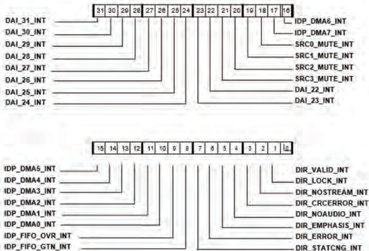
Figure A-5. DAI Interrupt Latch/Mask Register
