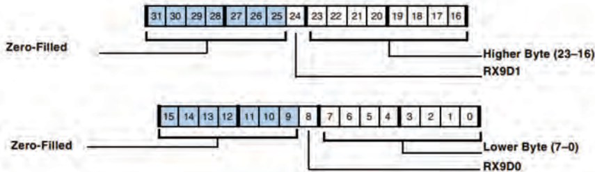
Figure 16-4. UART0 Receive Buffer Register
