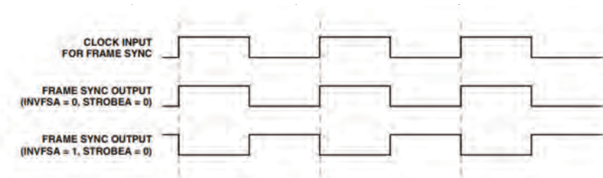
Figure 13-3. Bypass and Inverted Bypass
