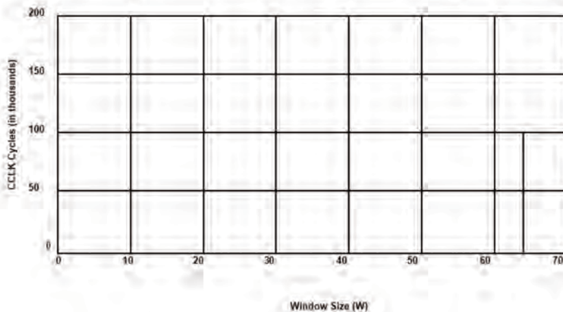
Figure 6-17. FIR Core/Accelerator Comparison, N = 2048
