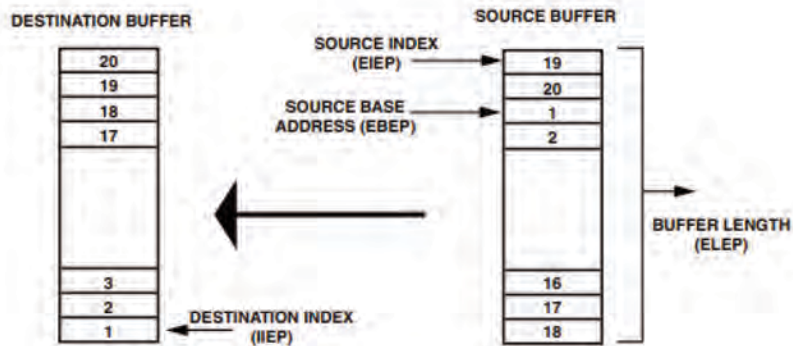
Figure 4-5. Circular Buffering Read DMA
