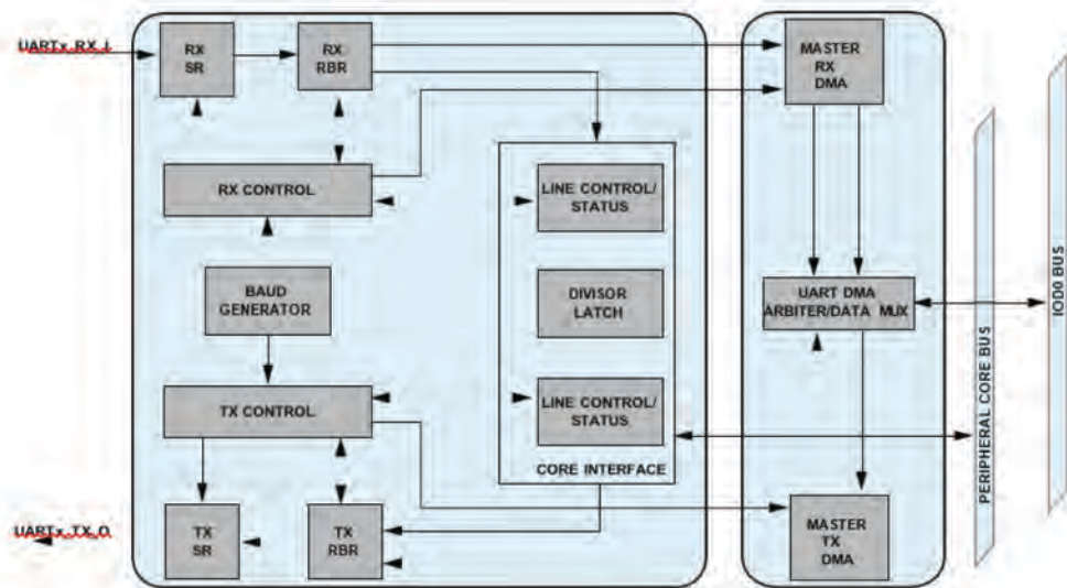
Figure 16-1. UART Functional Block Diagram
