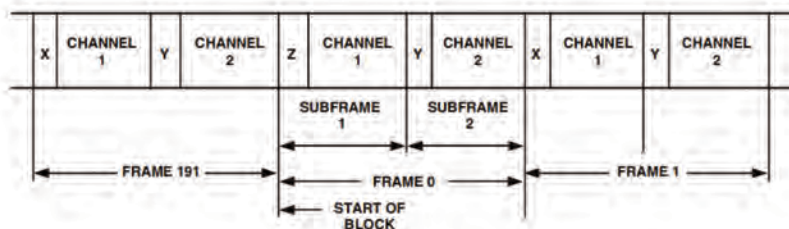
Figure C-4. S/PDIF Block Structure
