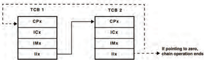
Figure 3-2. Chaining in the SPI and Serial Ports
