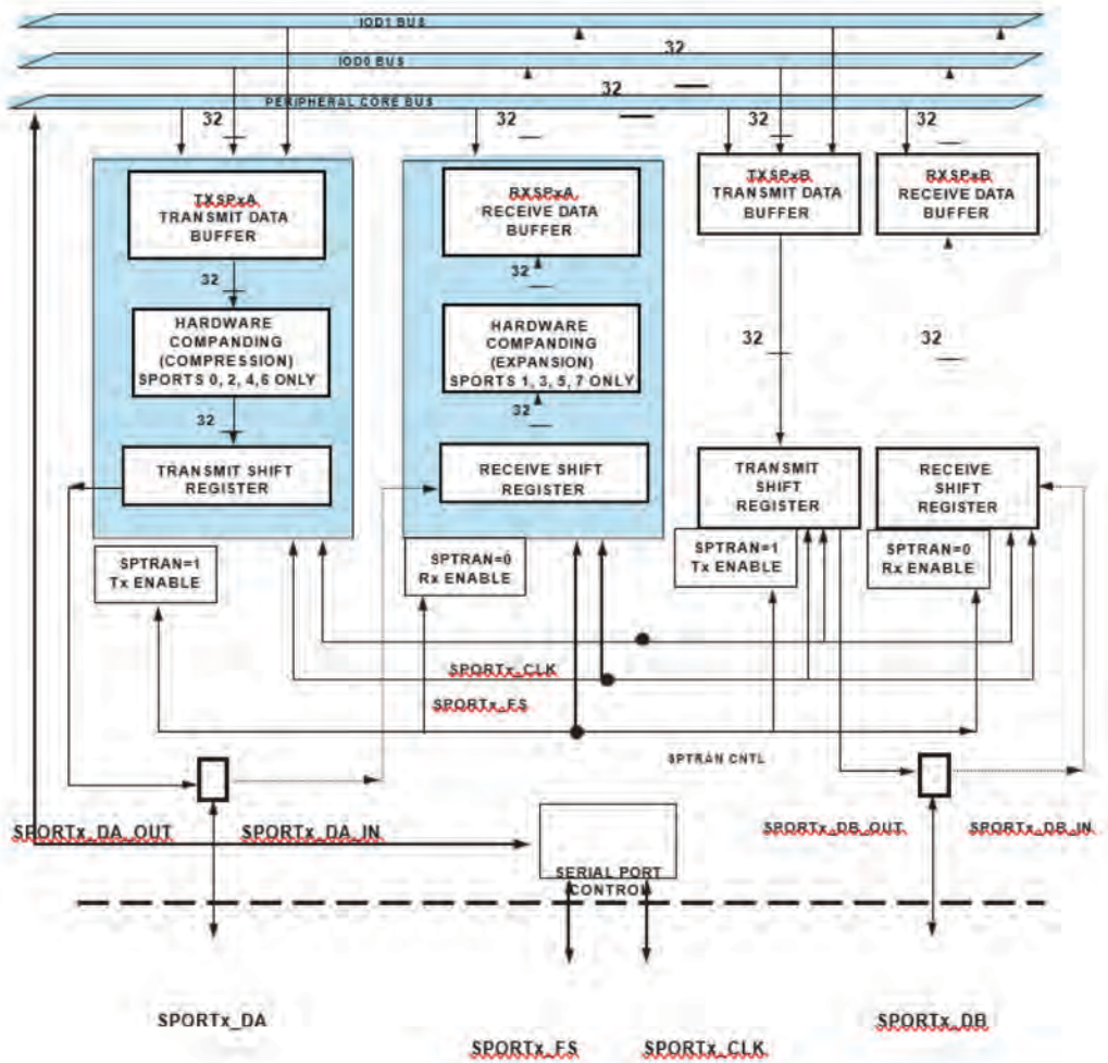
Figure 9-2. Serial Port Block Diagram
