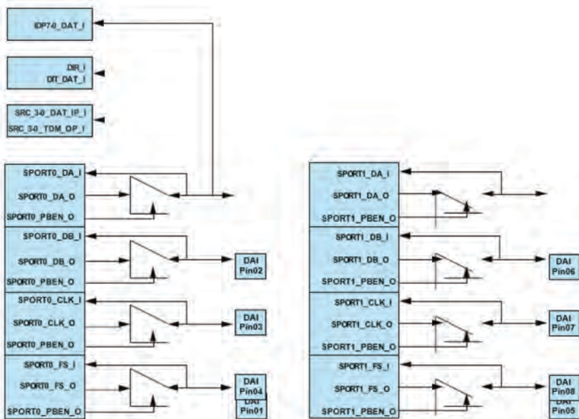
Figure 8-13. DAI Default Routing
