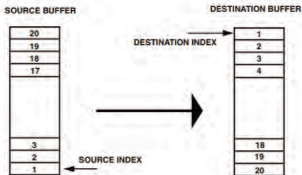
Figure 4-6. Standard Write
