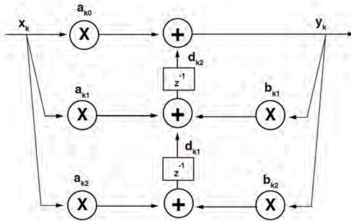
Figure 6-10. Transposed Direct Form II Biquad
