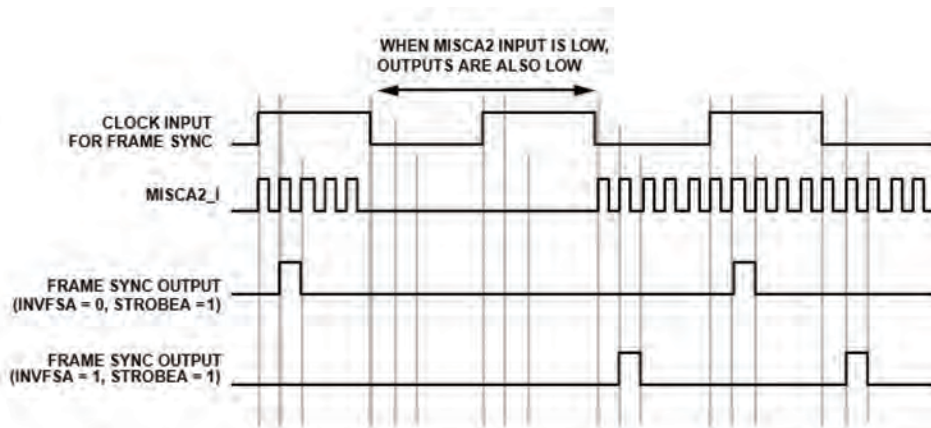
Figure 13-4. One Shot Mode PCG A (MISCA2_I input)
