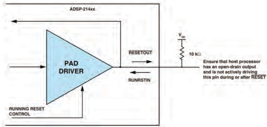
Figure 19-1. \overline{\text{RESETOUT}} Pin Multiplexed with RUNRSTIN
