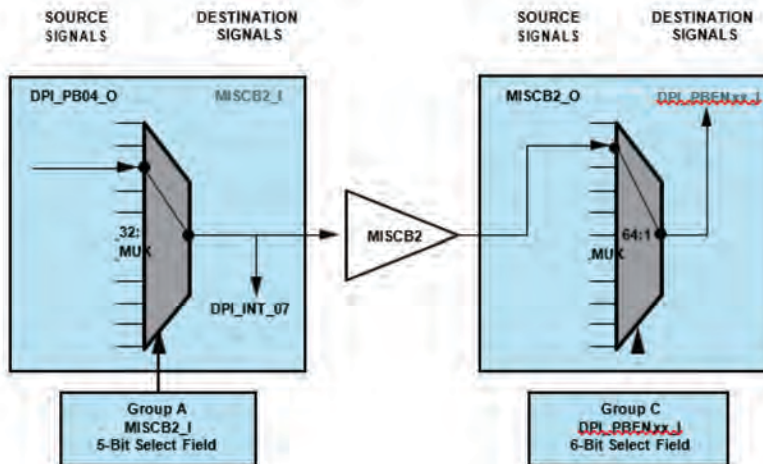
Figure 8-12. Miscellaneous DPI Connections
