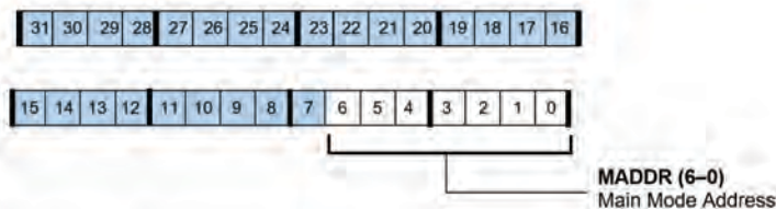
Figure A-57. TWIMADDR Register (RW)
