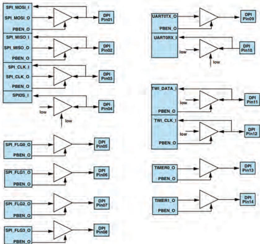
Figure 8-15. DPI Default Routing
