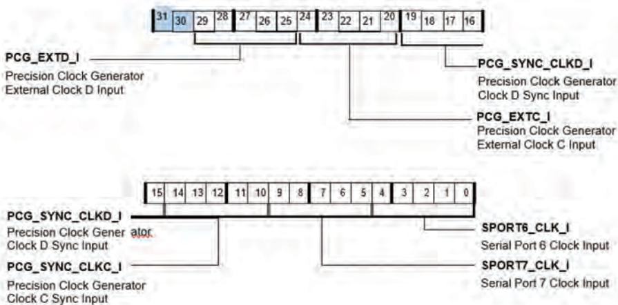
Figure A-16. SRU_CLK5 Register (RW)
