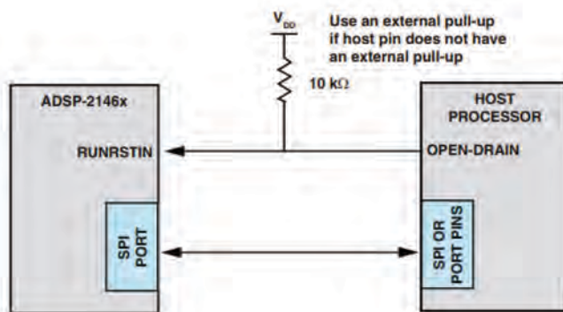
Figure 19-2. Example System Interface with an External Host
