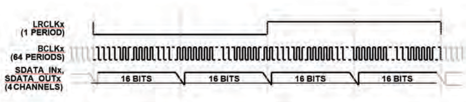
Figure C-3. Packed TDM4 Mode Timing
