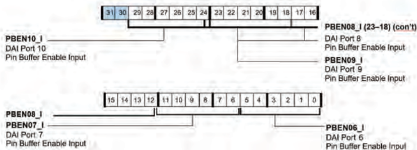
Figure A-37. SRU_PBEN1 (RW)
