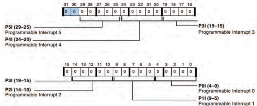
Figure A-1. PICR0 Register
