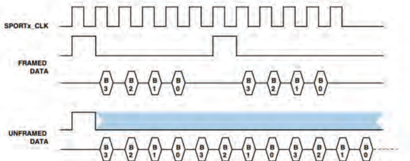
Figure 9-7. Framed vs. Unframed Data
