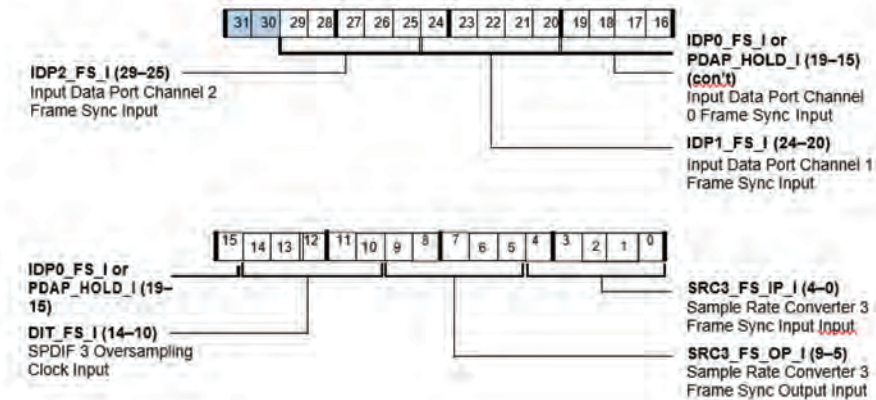
Figure A-26. SRU_FS2 Register (RW)
