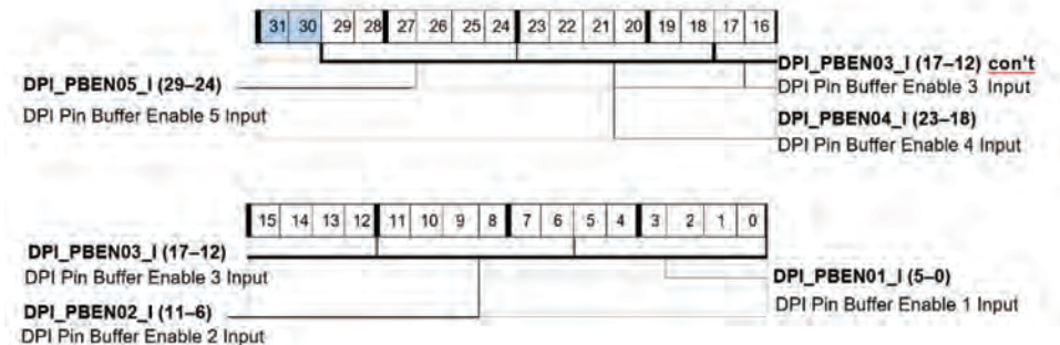
Figure A-51. SRU2_PBEN0 Register
