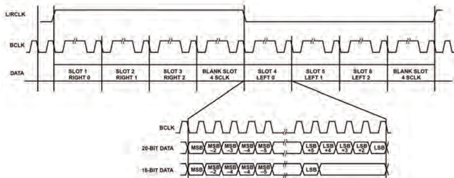
Figure C-2. Packed I 2 S Mode
