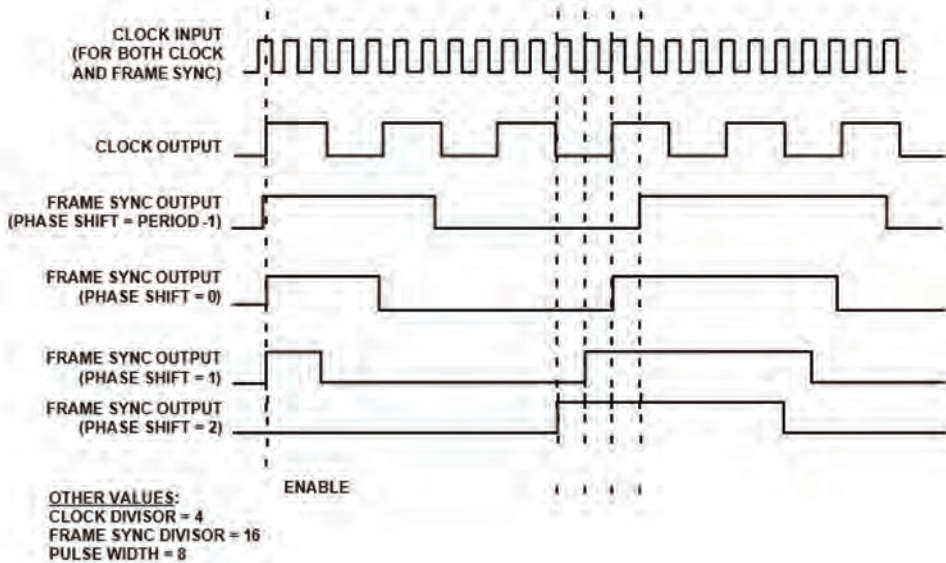
Figure 13-2. Phase and Pulse Width Settings
