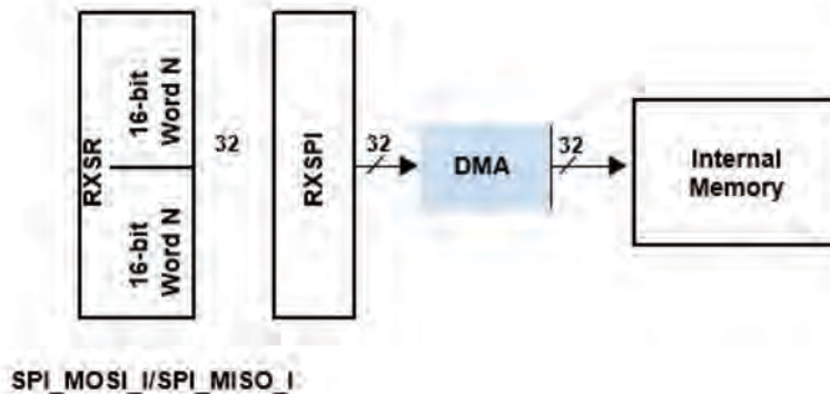
Figure 19-5. 16-Bit SPI Main/Subordinate Packing
