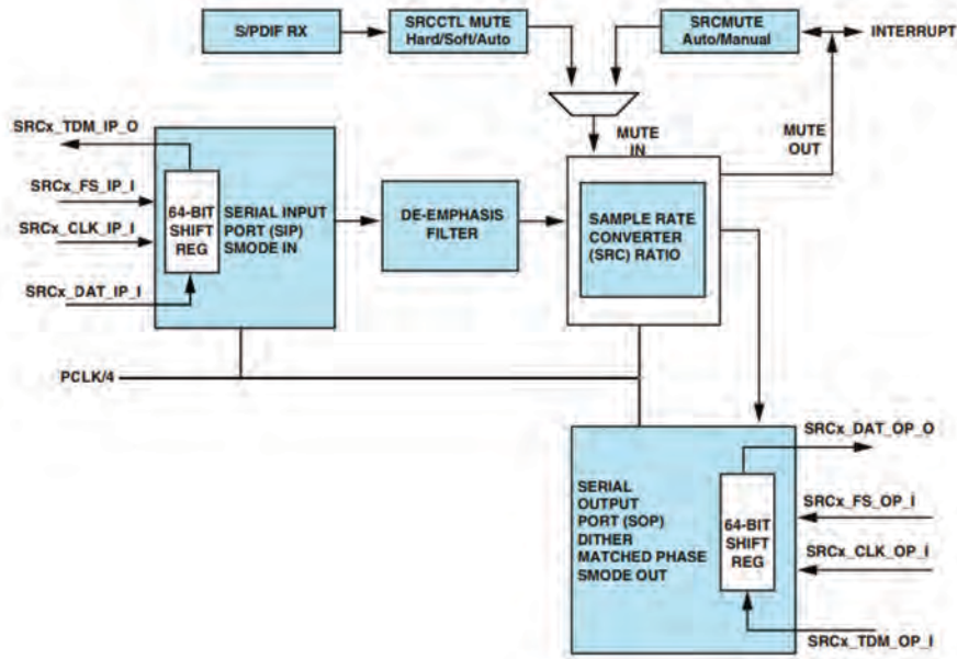
Figure 11-1. Top Level ASRC Block Diagram
