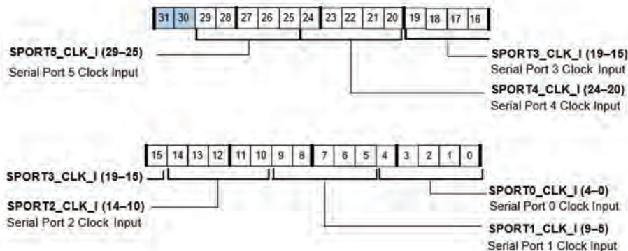
Figure A-11. SRU_CLK0 Register (RW)
