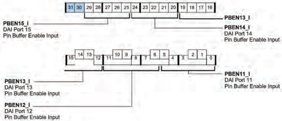
Figure A-38. SRU_PBEN2 (RW)
