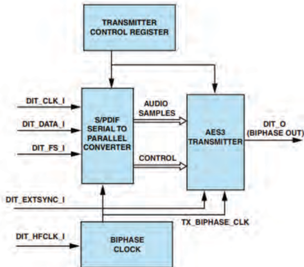
Figure 12-1. S/PDIF Transmitter Block Diagram
