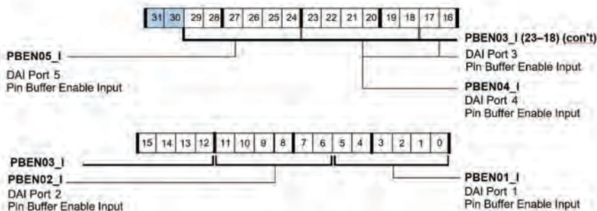
Figure A-36. SRU_PBEN0 (RW)
