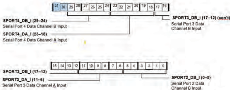
Figure A-18. SRU_DAT1 Register (RW)
