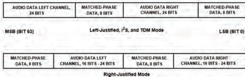
Figure 11-3. ASRC Data Frame Format by Protocol
