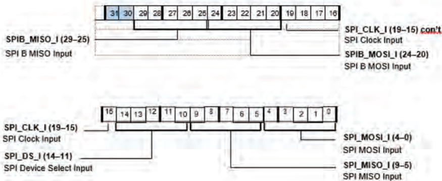
Figure A-42. SRU2_INPUT0 Register (RW)
