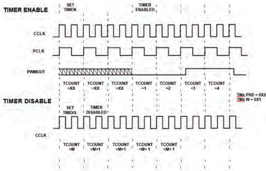
Figure 15-9. Timer PWM Enable and Disable Timing
