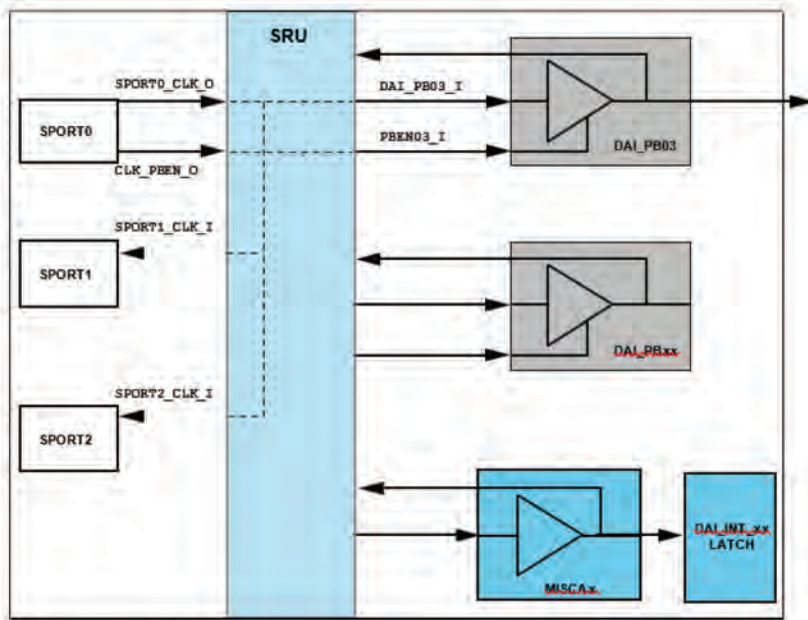
Figure 8-19. SRU Connection Between DAI Pin Buffers and SPORTs
