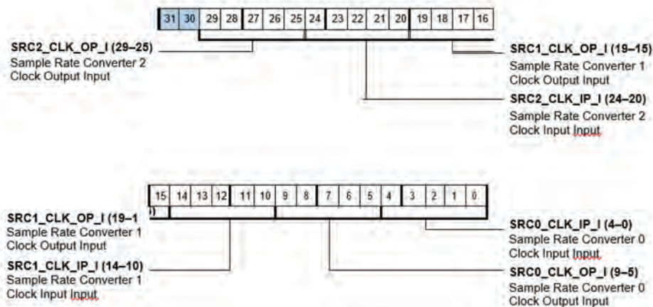
Figure A-12. SRU_CLK1 Register (RW)
