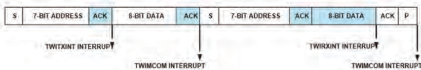
Figure 17-11. Transmit/Receive Data Repeated Start
