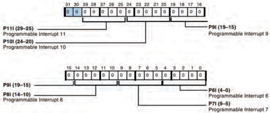
Figure A-2. PICR1 Register
