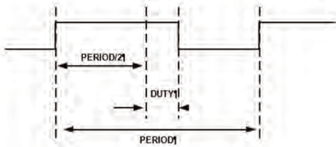
Figure 7-5. Edge Aligned PWM Wave with High Polarity
