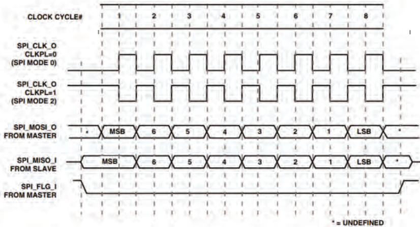
Figure 14-5. SPI Transfer Protocol for \text{CPHASE} = 0
