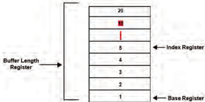
Figure 6-2. Circular Buffer Addressing
