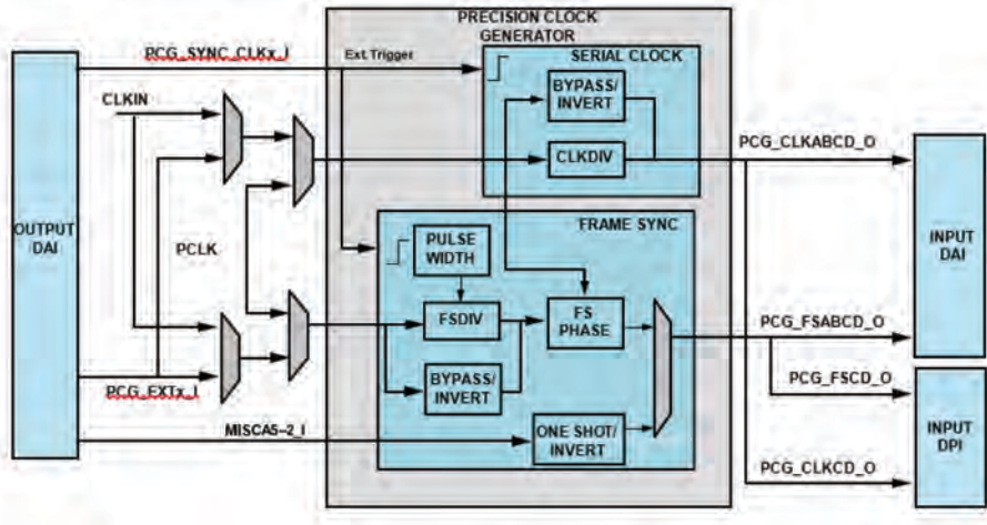
Figure 13-1. PCG Block Diagram
