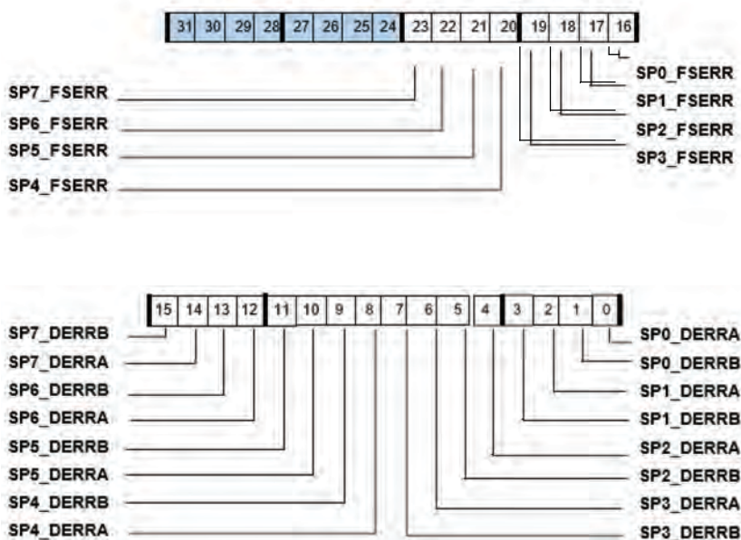
Figure A-41. SPERRSTAT Register (RO)
