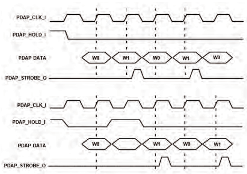
Figure 10-4. PDAP Hold Input (Packing by 2)
