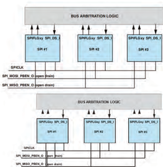
Figure 14-4. Multi-Main System
