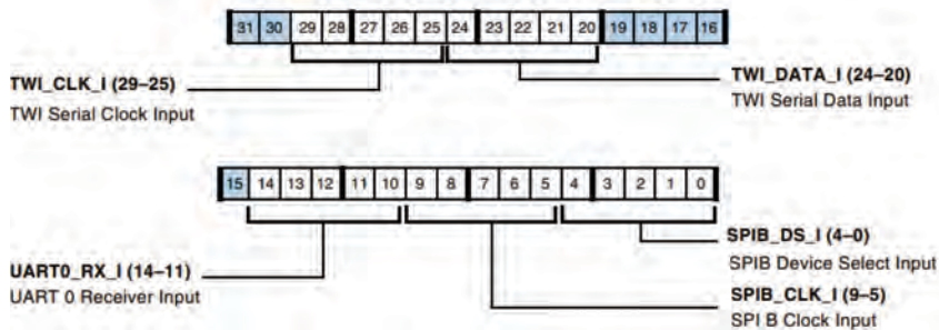
Figure A-43. SRU2_INPUT1 Register (RW)
