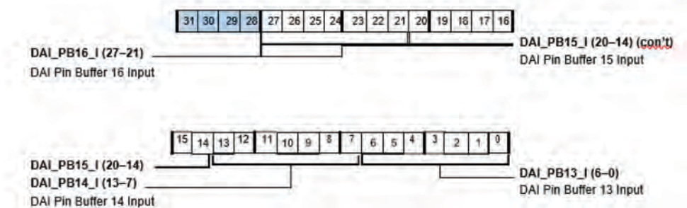
Figure A-32. SRU_PIN3 Register (RW)
