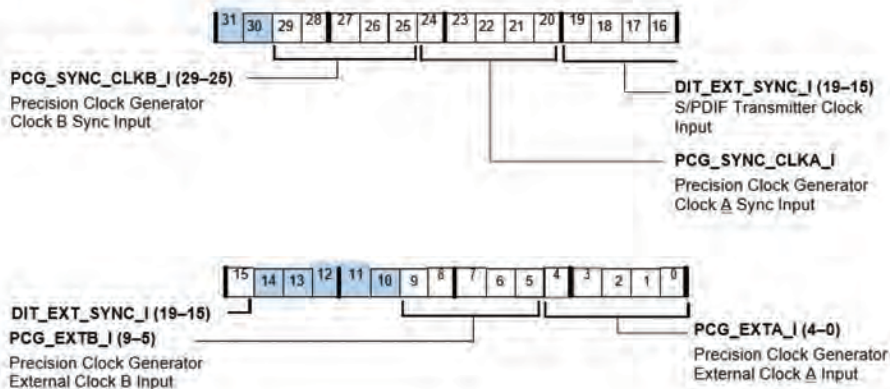
Figure A-15. SRU_CLK4 Register (RW)
