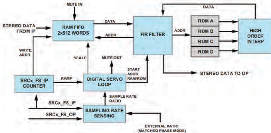
Figure 11-2. Core Architecture
