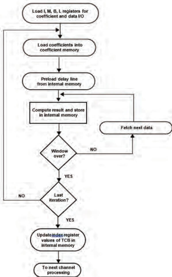
Figure 6-6. Single Channel Filtering Flow
