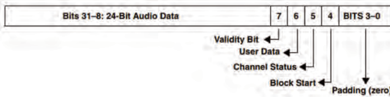
Figure 12-3. I 2 S and Left-Justified Formats
