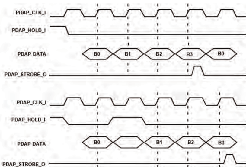
Figure 10-5. PDAP Hold Input (Packing by 4)
