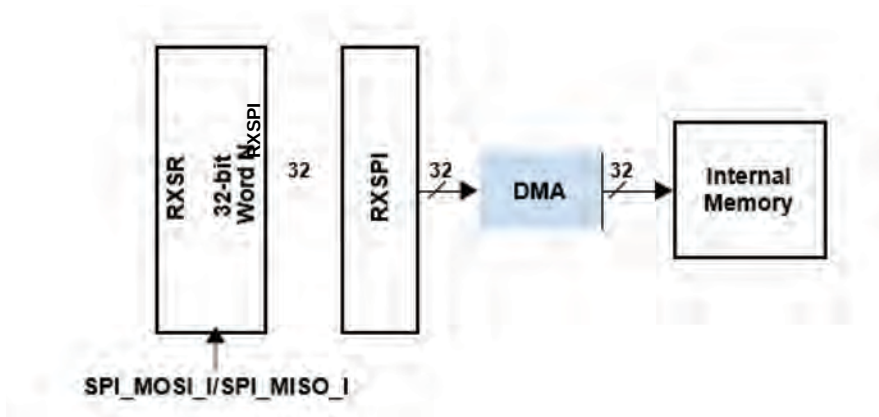
Figure 19-4. 32-Bit SPI Main/Subordinate Packing
