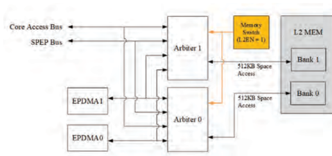
Figure 4-1. Functional Block Diagram
