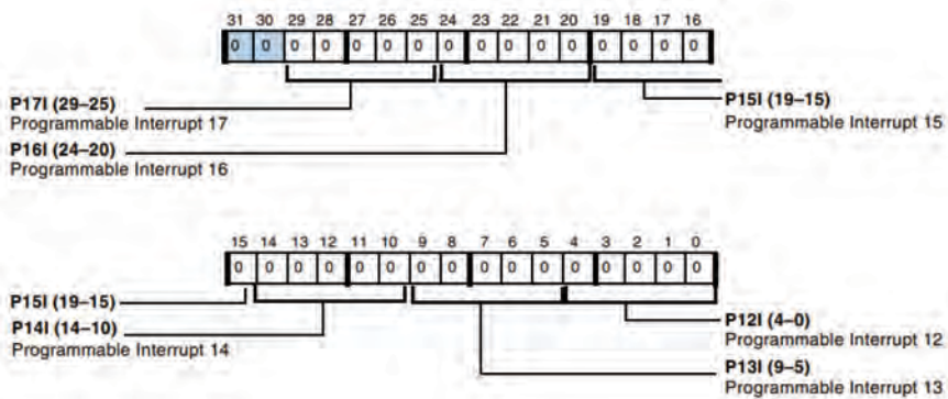
Figure A-3. PICR2 Register
