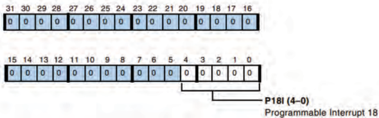
Figure A-4. PICR3 Register
