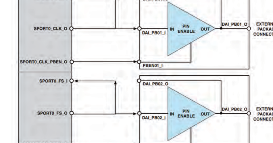
Figure 9-1. SRU Configuration when SPORT is Main Receiver
