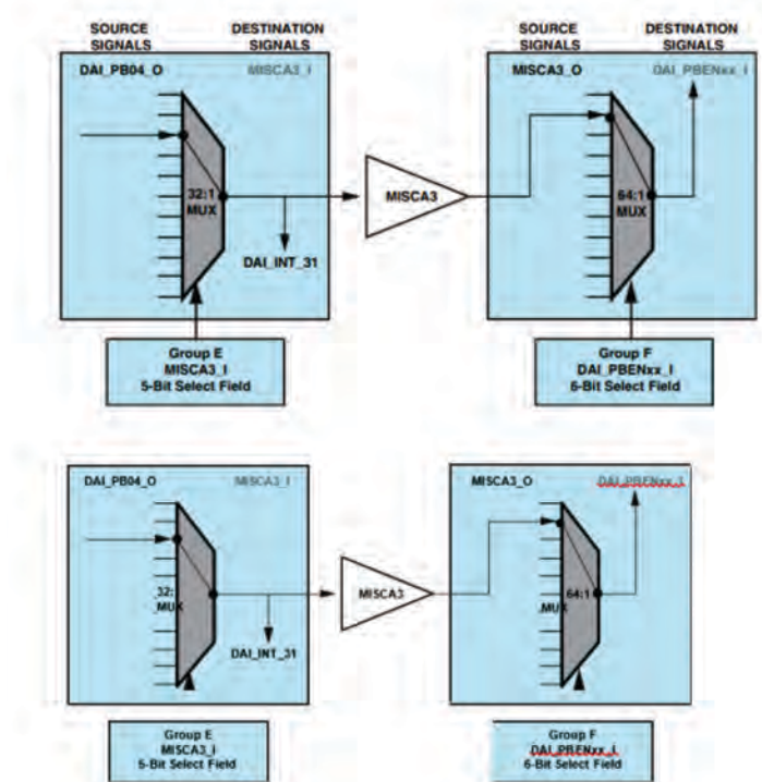
Figure 8-11. Miscellaneous DAI Connections
