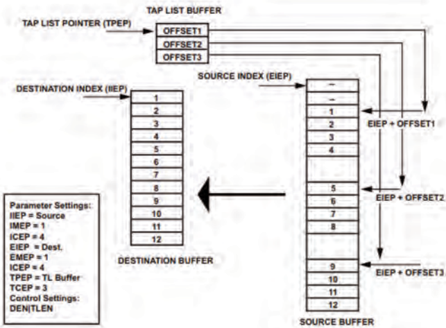
Figure 4-8. Gather DMA (Reads)
