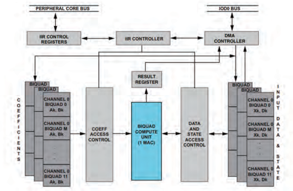
Figure 6-9. IIR Accelerator Block Diagram
