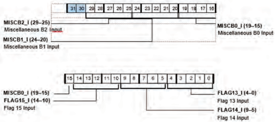
Figure A-46. SRU2_INPUT4 Register (RW)
