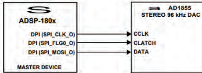
Figure 14-3. SHARC Processor as SPI Main
