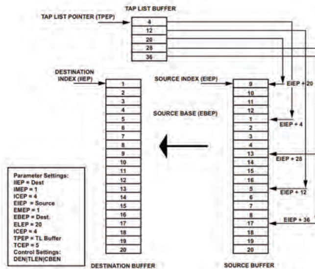
Figure 4-10. Circular Gather DMA (Reads)
