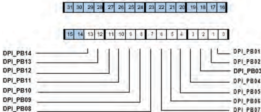
Figure A-54. DPI_PIN_STAT Register
