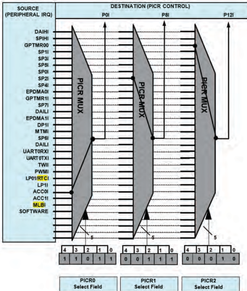
Figure 2-1. Programmable Prioritized Interrupts
