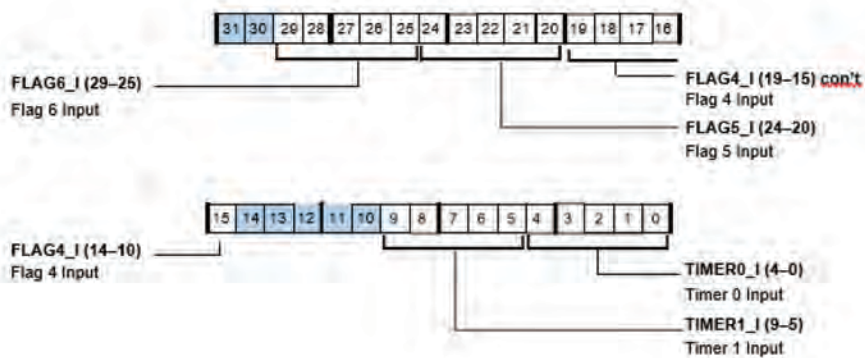
Figure A-44. SRU2_INPUT2 Register (RW)
