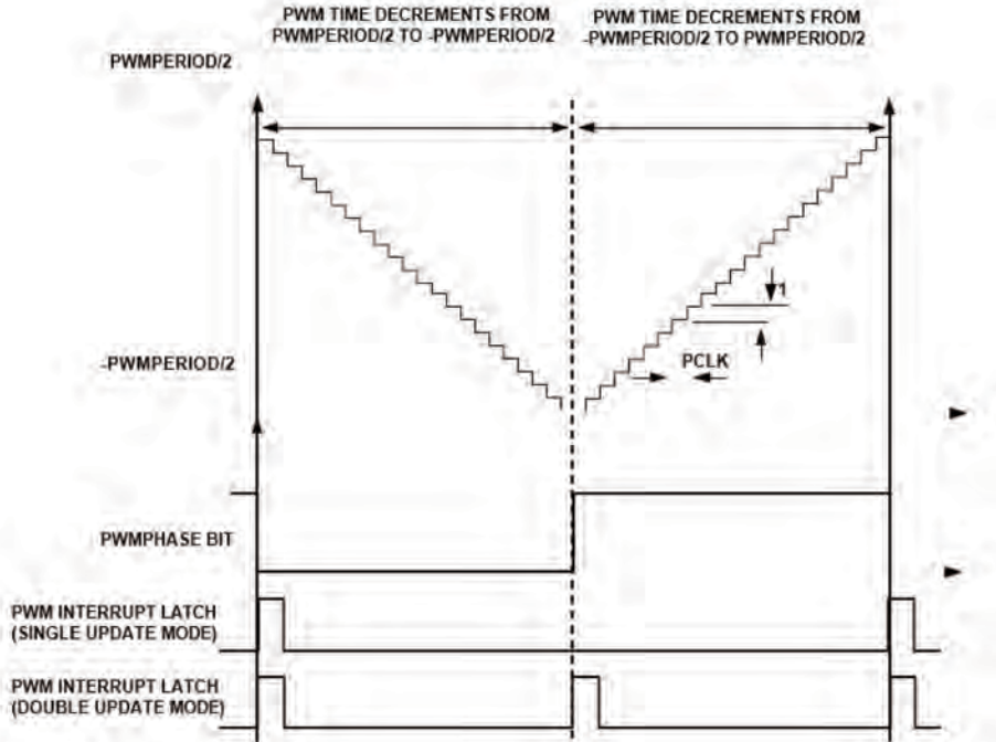
Figure 7-6. Operation of Internal PWM Timer (Center Aligned)
