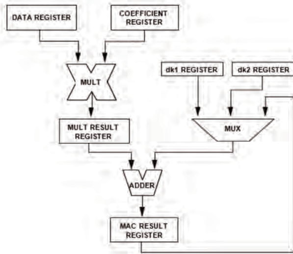
Figure 6-11. IIR MAC Unit
