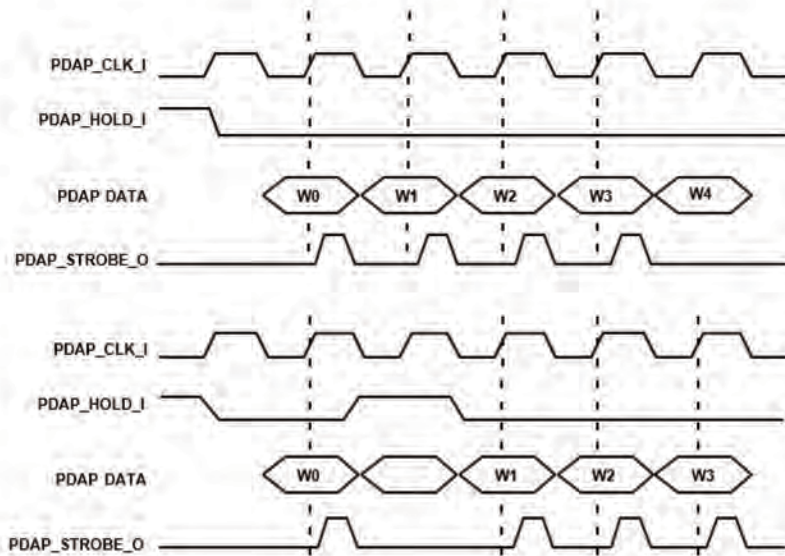
Figure 10-3. PDAP Hold Input (No Packing)
