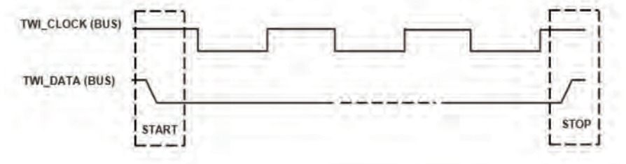
Figure 17-6. TWI Start and Stop Conditions
