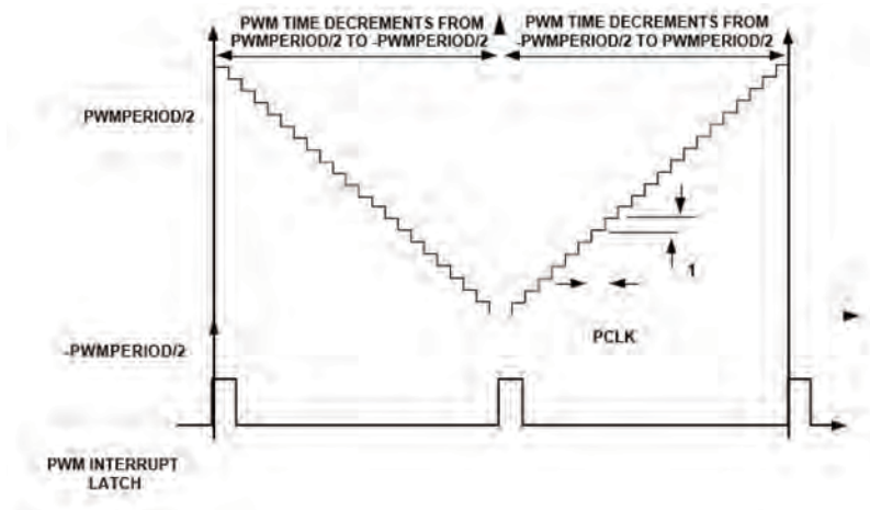
Figure 7-7. Operation of Internal PWM Timer (Edge Aligned)
