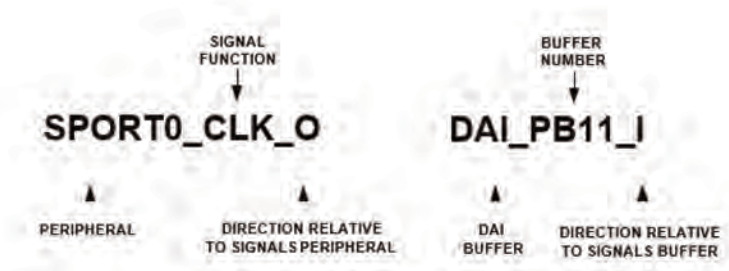
Figure 8-3. Example SRU Mnemonics
