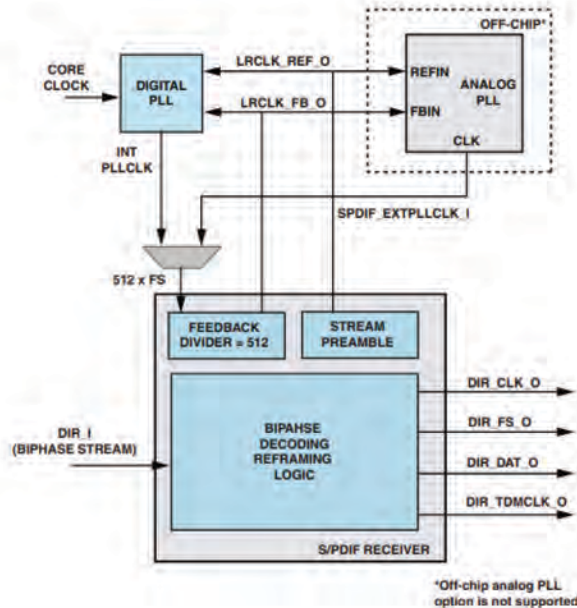
Figure 12-5. S/PDIF Receiver Block Diagram
