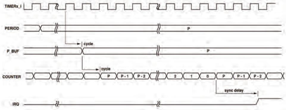
Figure 15-8. EXT_CLK Timing
