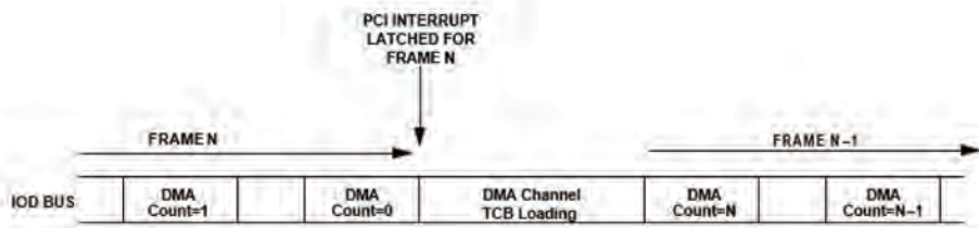
Figure 3-3. DMA Chaining
