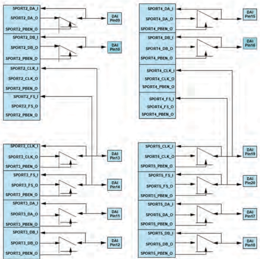
Figure 8-14. DAI Default Routing (Con't)
