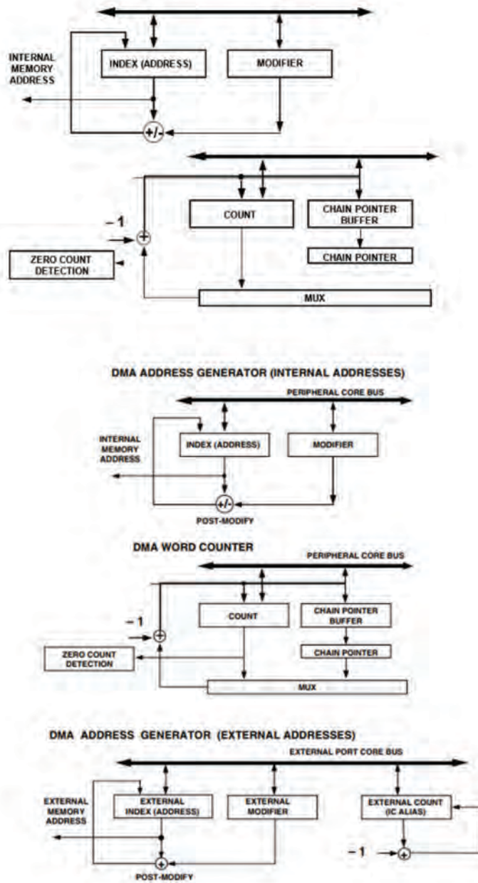
Figure 3-1. DMA Address Generator
