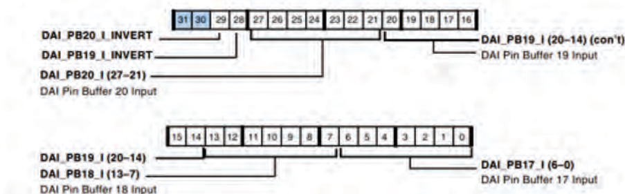
Figure A-33. SRU_PIN4 Register (RW)
