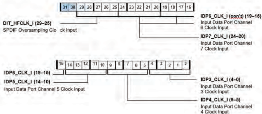
Figure A-14. SRU_CLK3 Register (RW)
