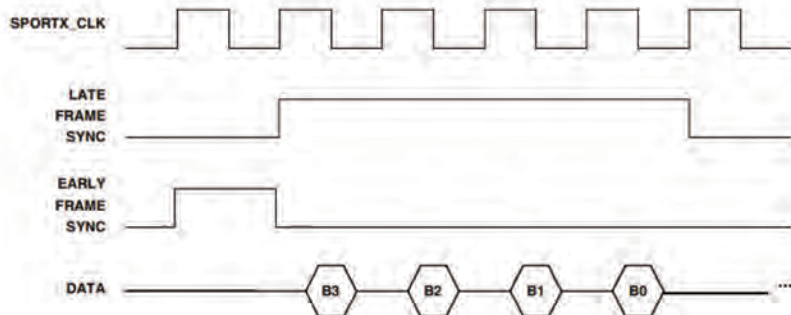
Figure 9-8. Normal vs. Alternate Framing
