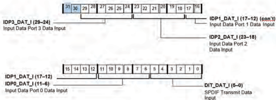
Figure A-21. SRU_DAT4 Register (RW)
