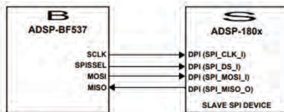
Figure 14-2. SHARC Processor as SPI Subordinate
