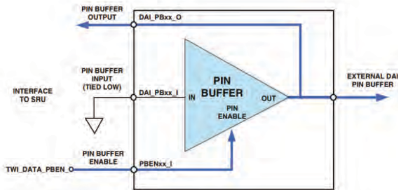
Figure 8-7. Pin Buffer as Open Drain
