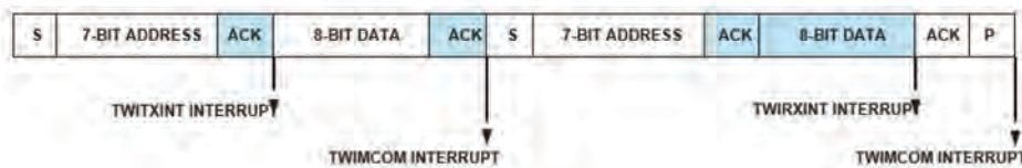
Figure 17-12. Receive/Transmit Data Repeated Start
