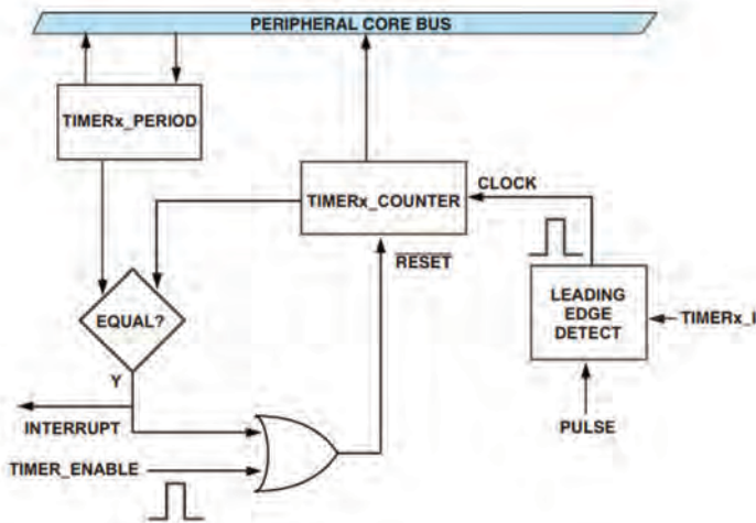
Figure 15-7. Flow Diagram EXT_CLK Mode
