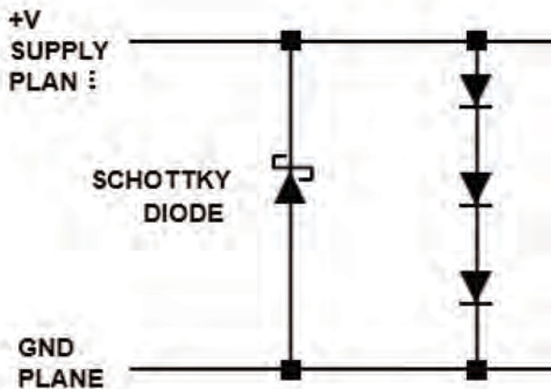
Figure 19-8. Schottky Diode
