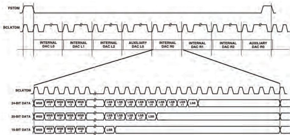
Figure C-1. TDM Mode Timing
