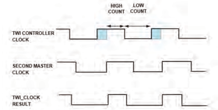
Figure 17-2. TWI Clock Synchronization
