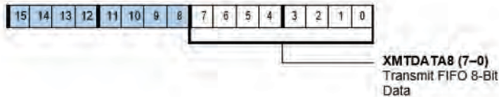
Figure 17-7. 8-Bit Transmit FIFO Register
