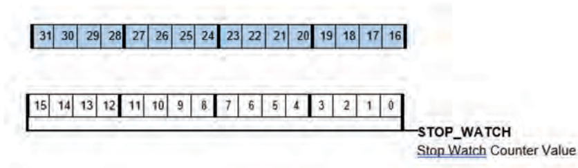
Figure A-8. RTC_STPWTCR Register (RW)
