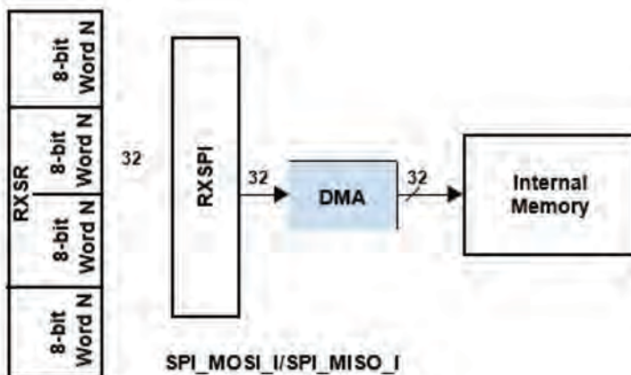
Figure 19-6. 8-Bit SPI Subordinate Packing
