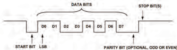
Figure 16-2. Bit Stream on the Transmit Pin
