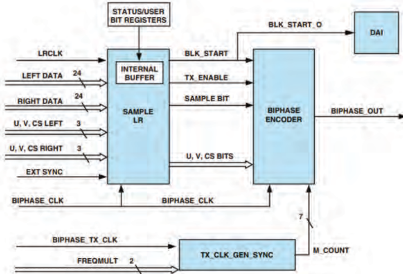
Figure 12-2. AES3 Output Block
