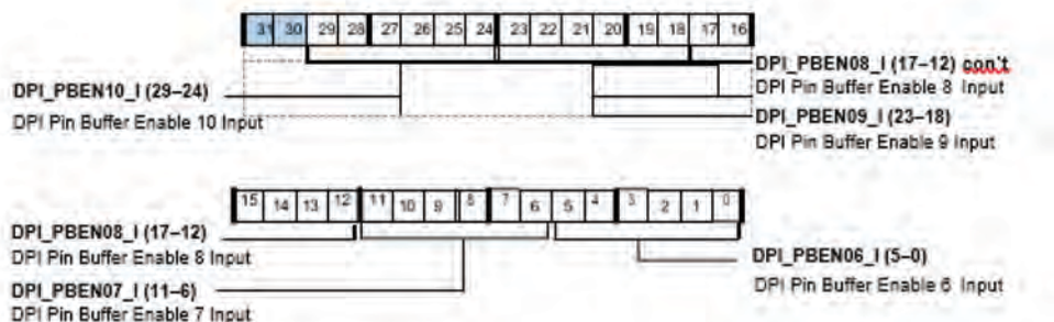
Figure A-52. SRU2_PBEN1 Register
