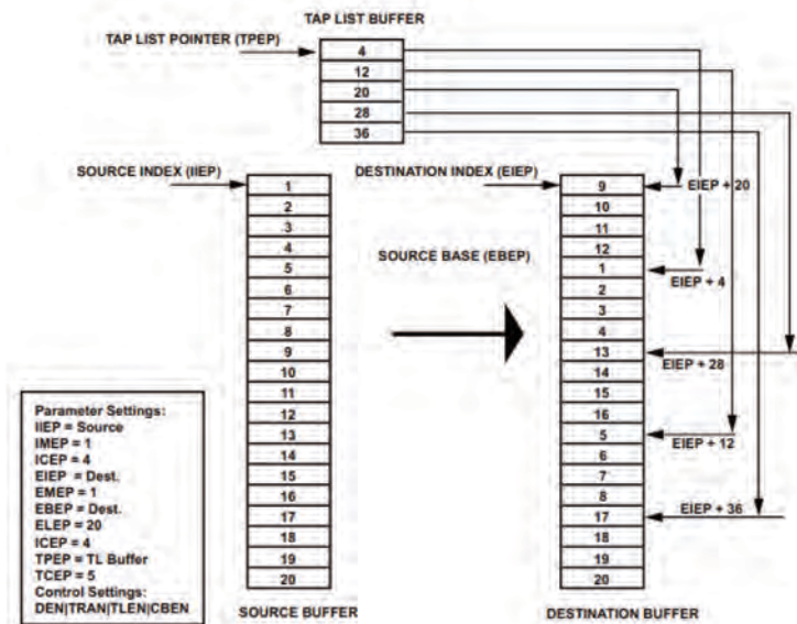
Figure 4-9. Circular Buffering Scatter DMA (Writes)
