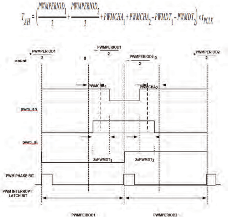
Figure 7-3. Center-Aligned Paired PWM in Double Update Mode, Low Polarity
