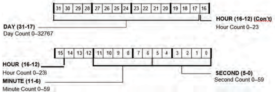
Figure A-9. RTC_CLOCK Register (RW)
