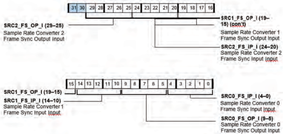
Figure A-25. SRU_FS1 Register (RW)
