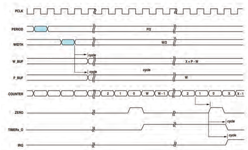
Figure 15-3. PWM_OUT Timing
