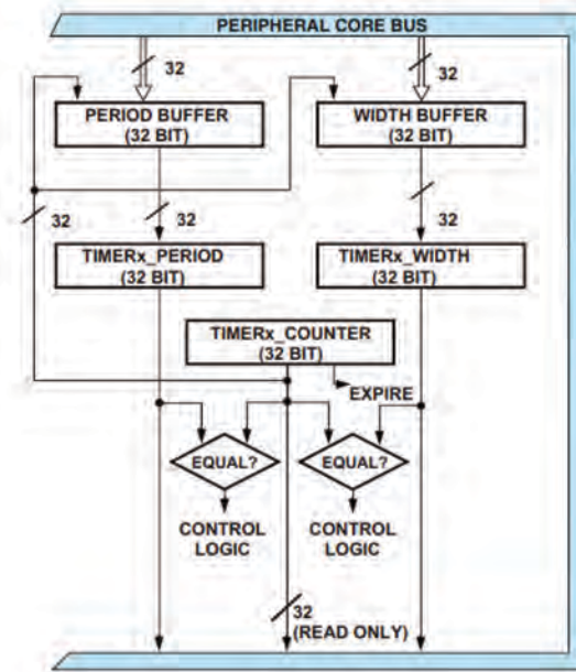
Figure 15-1. Timer Block Diagram with Buffered Period and Width Registers
