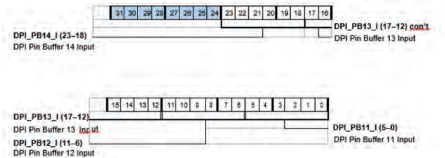
Figure A-50. SRU2_PIN2 Register
