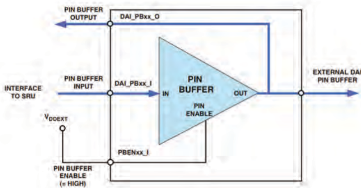
Figure 8-6. Pin Buffer as Output
