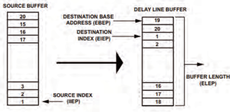
Figure 4-11. Write to Delay Line Buffer
