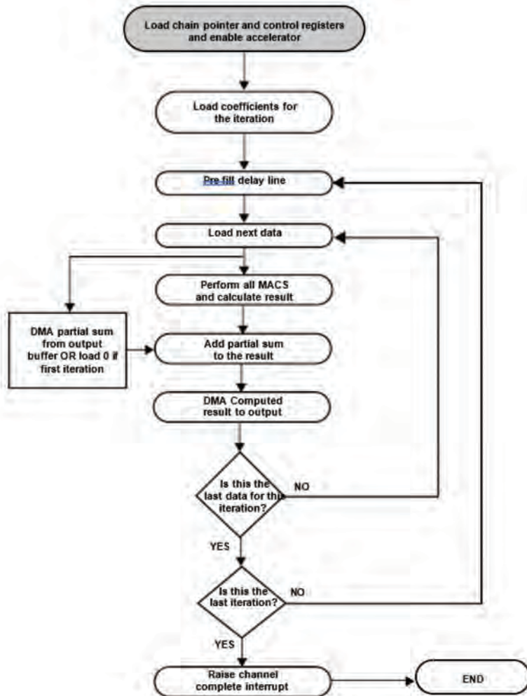
Figure 6-5. Multi-Iteration Filtering Flow
