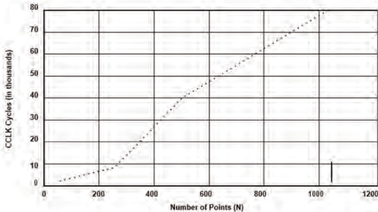
Figure 6-15. FFT Accelerator Comparison to Core
