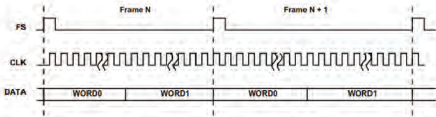
Figure 9-4. TDM and Multichannel Protocol
