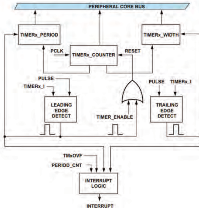
Figure 15-5. Timer Flow Diagram – WIDTH_CAP Mode
