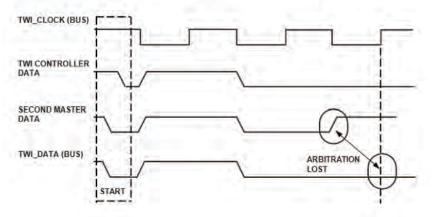
Figure 17-5. TWI Bus Arbitration
