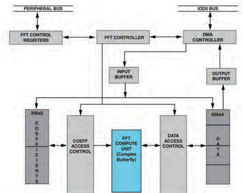
Figure 6-1. FFT Block Diagram
