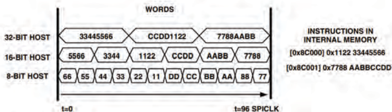
Figure 19-3. Instruction Packing for Different Hosts
