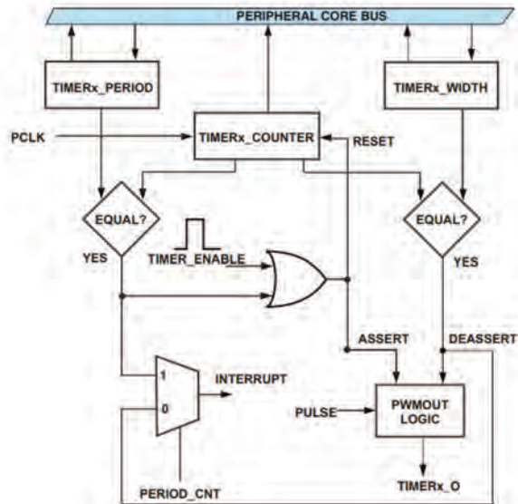
Figure 15-2. Timer Flow Diagram – PWM_OUT Mode
