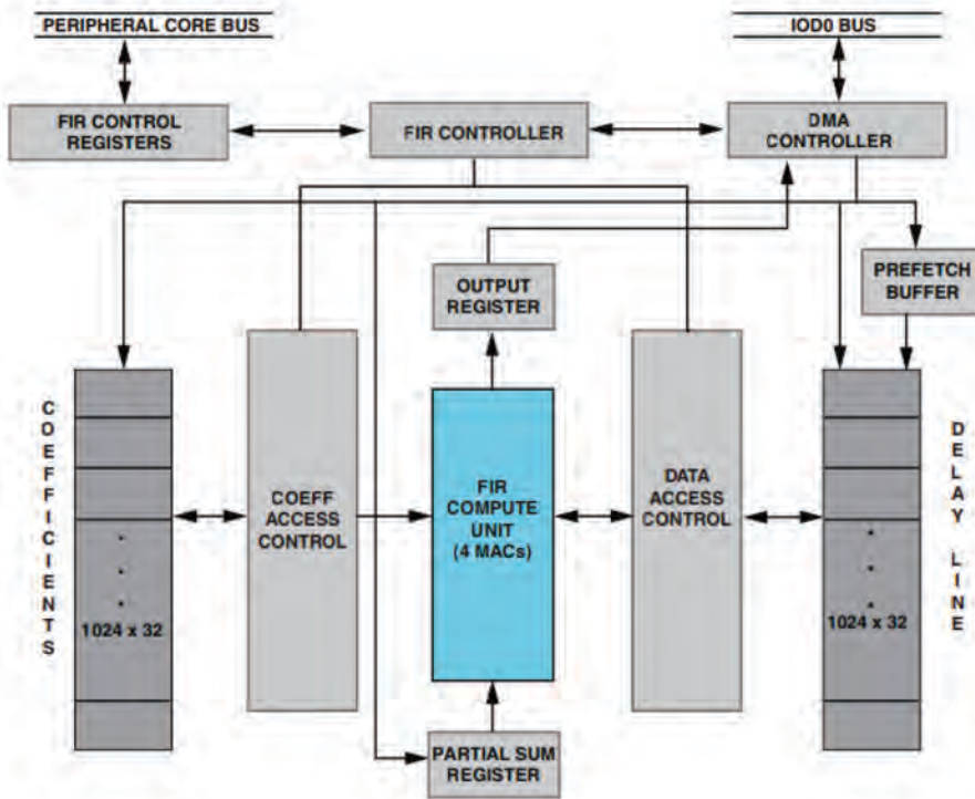
Figure 6-3. FIR Block Diagram
