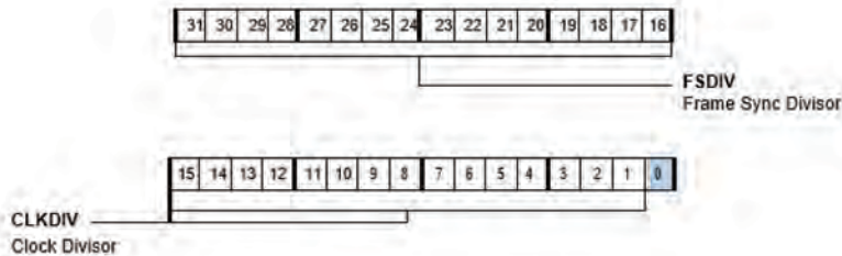
Figure A-40. DIVx Register (RW)
