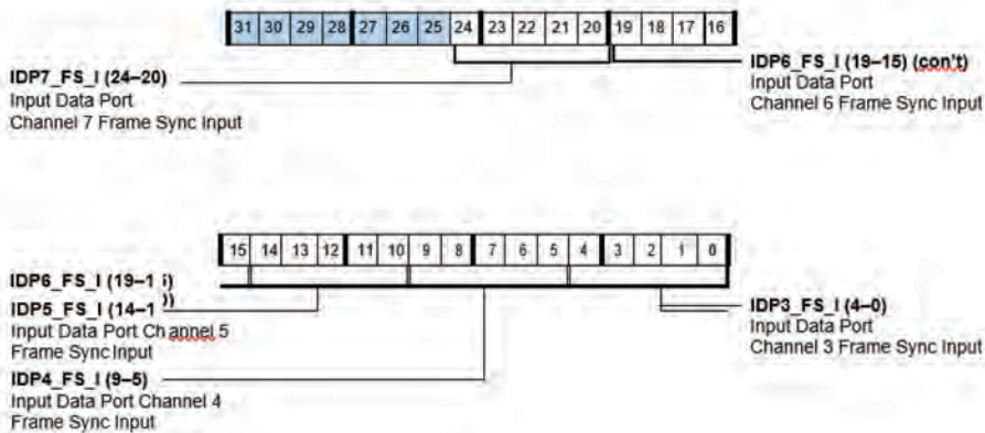
Figure A-27. SRU_FS3 Register (RW)
