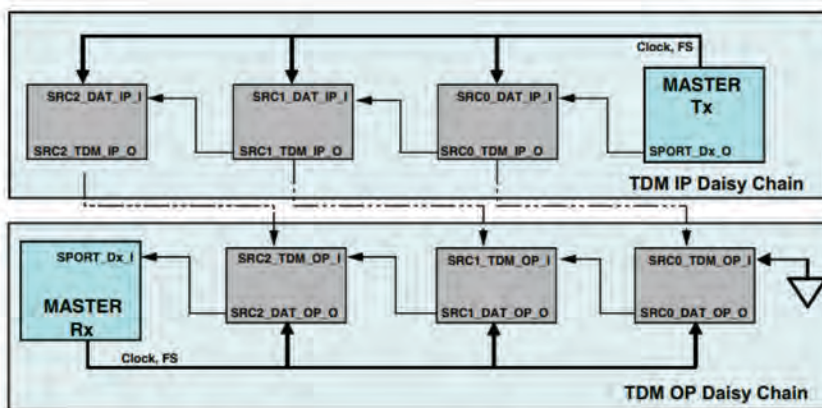
Figure 11-4. TDM Input/Output Modes
