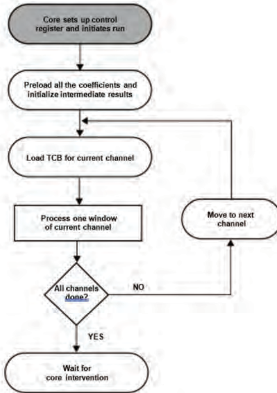
Figure 6-14. Biquad Processing Program Flow
