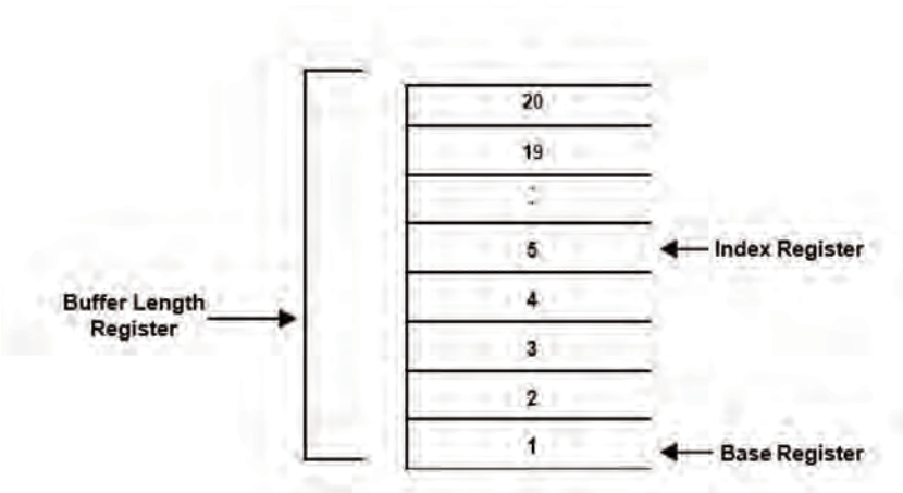
Figure 6-7. Circular Buffer Addressing
