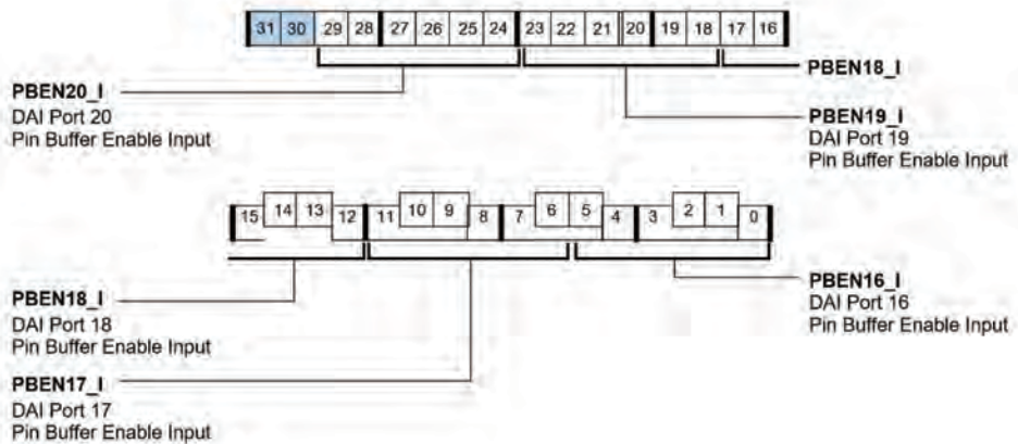
Figure A-39. SRU_PBEN3 (RW)
