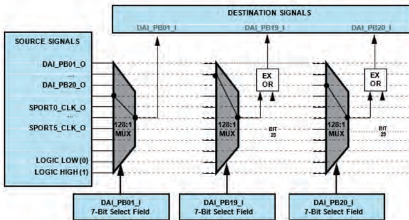
Figure 8-16. Pin Buffer Polarity
