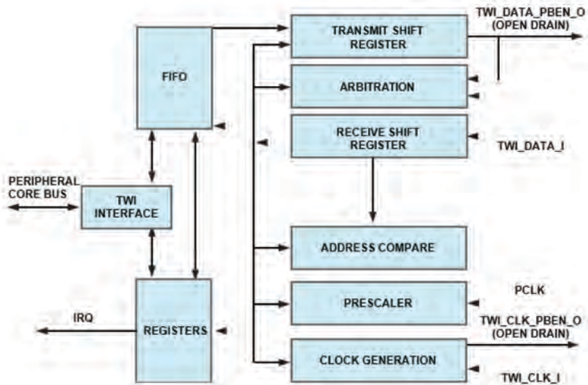
Figure 17-1. TWI Block Diagram
