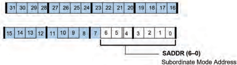
Figure A-58. TWISADDR Register (RW)
