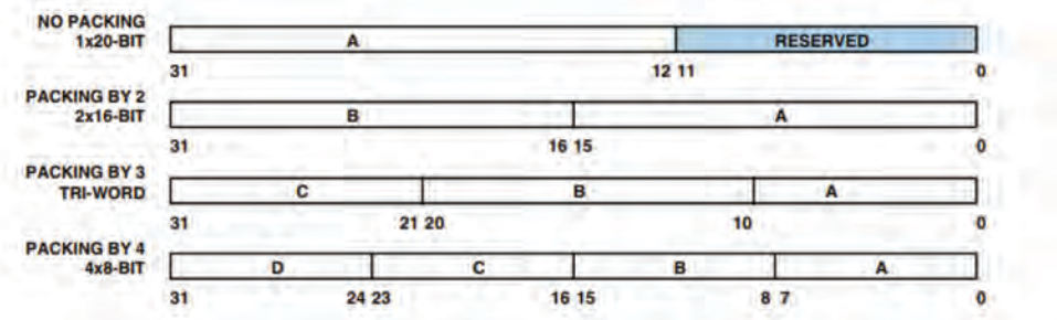
Figure 10-9. IDP Data Buffer Formats for the PDAP
