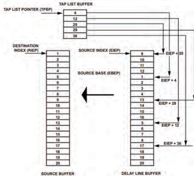
Figure 4-12. Read From Delay Line Buffer
