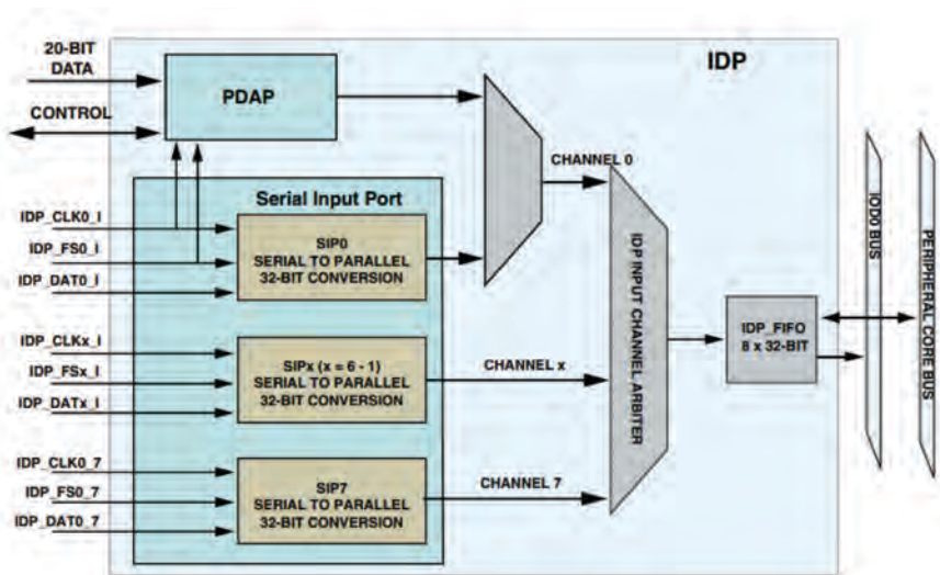
Figure 10-1. Input Data Port
