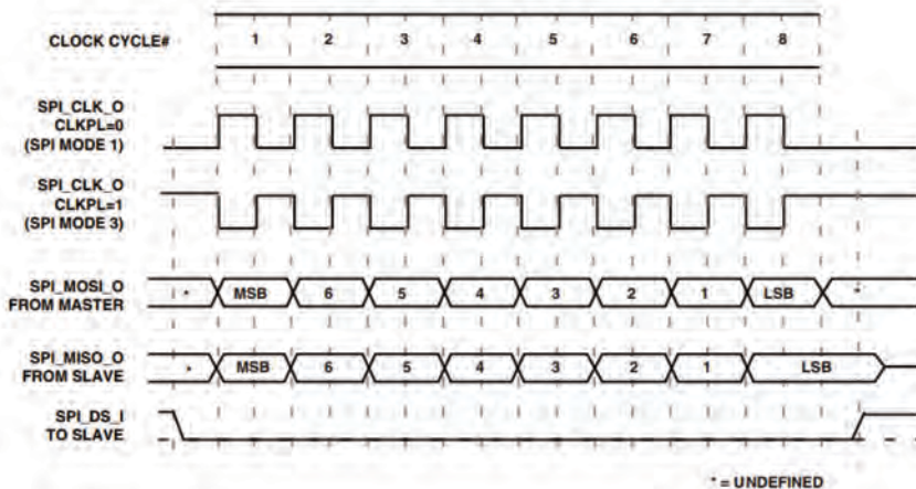
Figure 14-6. SPI Transfer Protocol for \text{CPHASE} = 1
