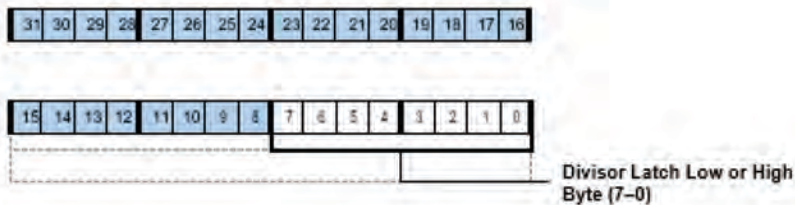
Figure A-55. UART Divisor Latch Registers (UART0DLL, UART0DLH)
