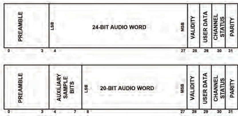
Figure C-5. Subframe Format
