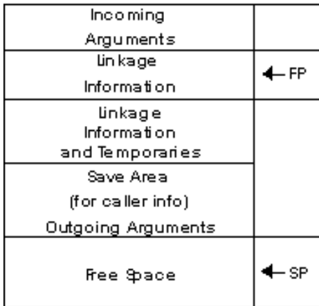
Figure 1-3. ADSP-TS101 Processor Stack
