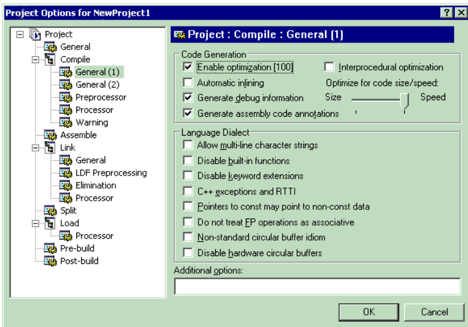
Figure 1-1. Project Options Compile General Property Page
