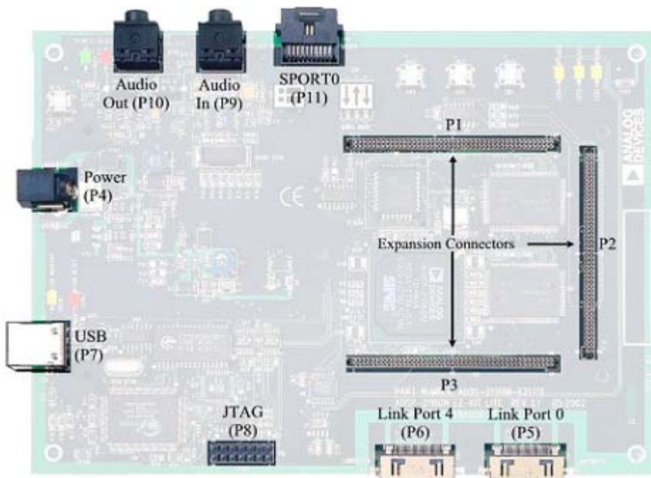
Figure 2-4. Connector Locations
