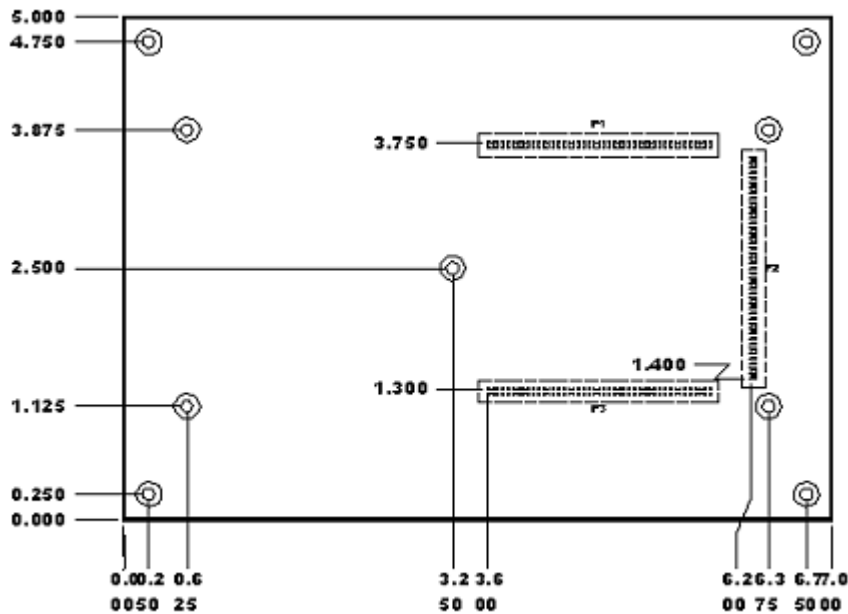
Figure 2-5. Mechanical Drawing
