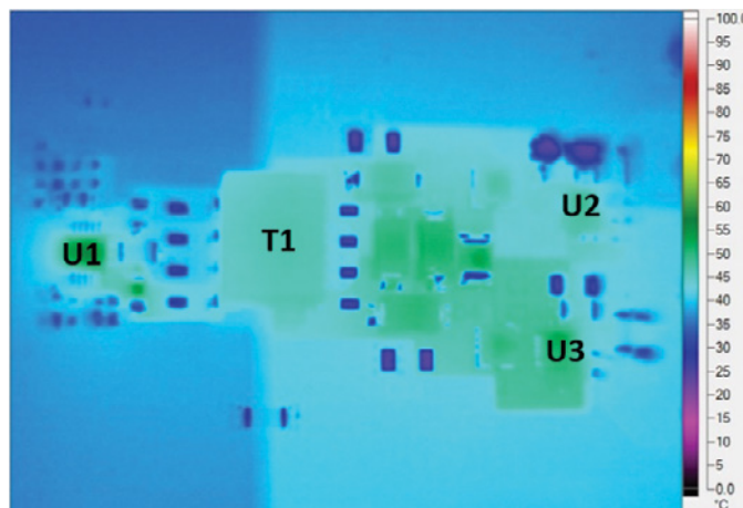
Figure 6. Thermal Image, V IN = 15V, I OUT1 = I OUT2 = 200mA
