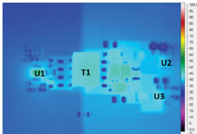
Figure 5. Thermal Image, V IN = 10V, I OUT1 = I OUT2 = 200mA
