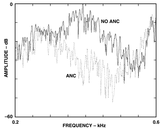
Figure 12. Performance with broadband disturbance.
