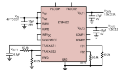
Figure 5. Example Schematic of Ratiometric Output Voltage Tracking
