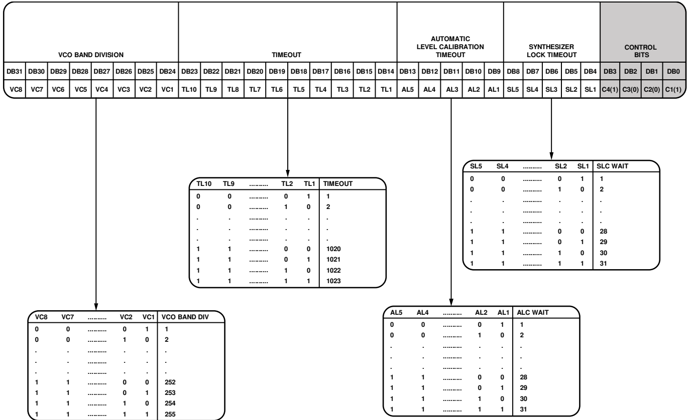
Figure 47. Register 9 Details
