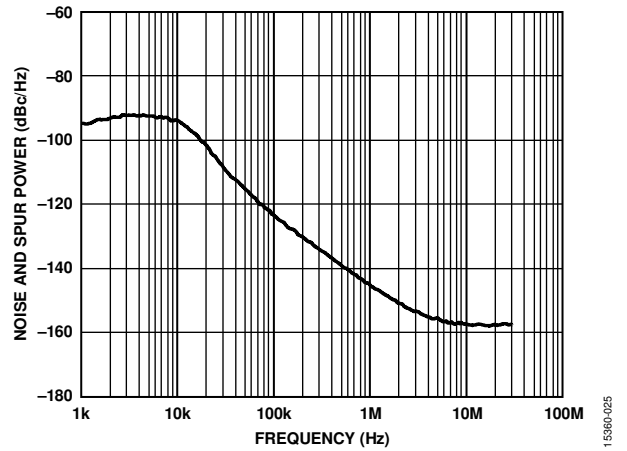
Figure 25. Fractional-N Spur Performance, GSM1800 Band, RF_{OUTA+} = 1550.2 MHz, f_{REFIN} = 122.88 MHz, f_{PFD} = 61.44 MHz, Output Divide by 4 Selected, Loop Filter Bandwidth = 10 kHz, Channel Spacing = 20 kHz
