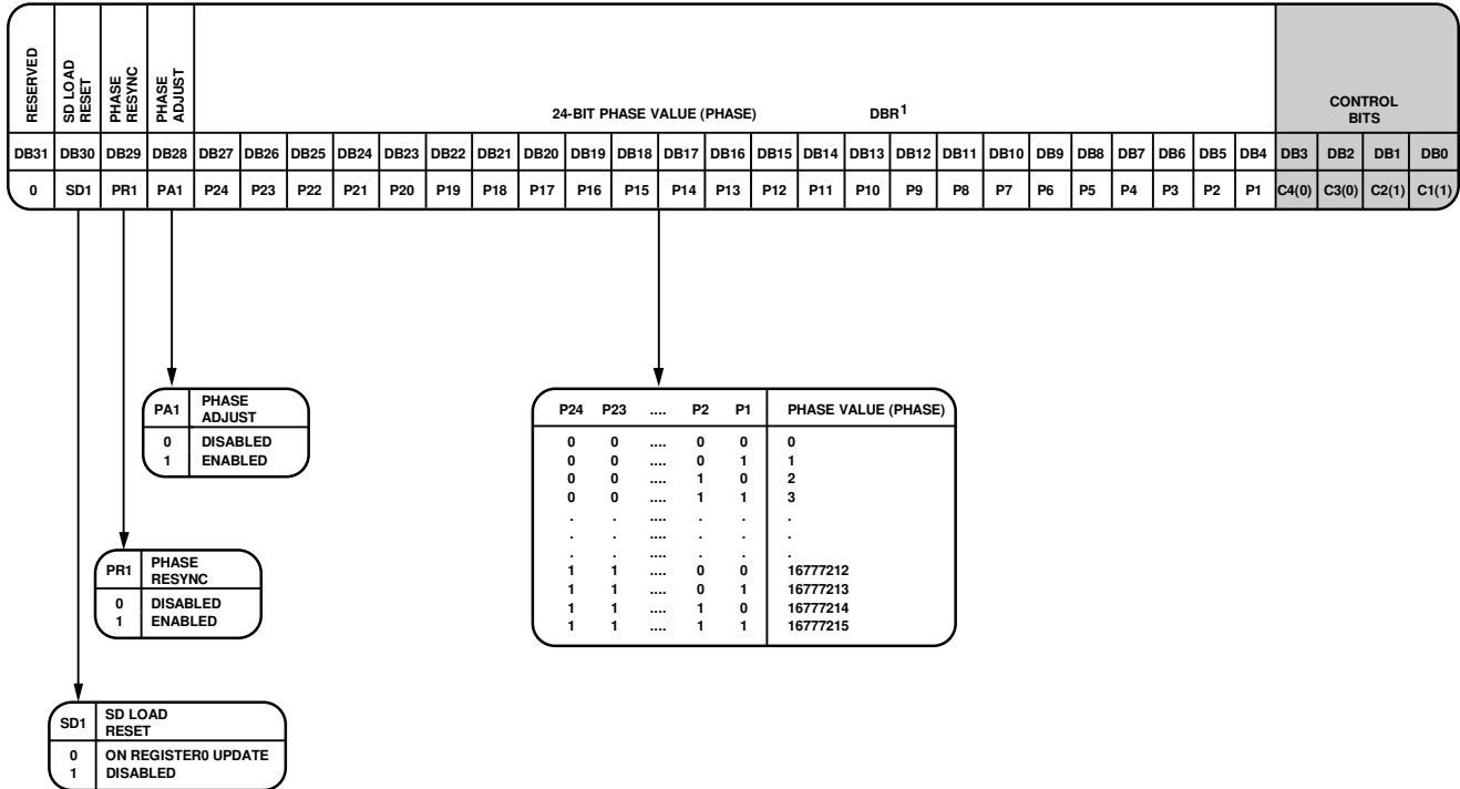
Figure 41. Register 3
