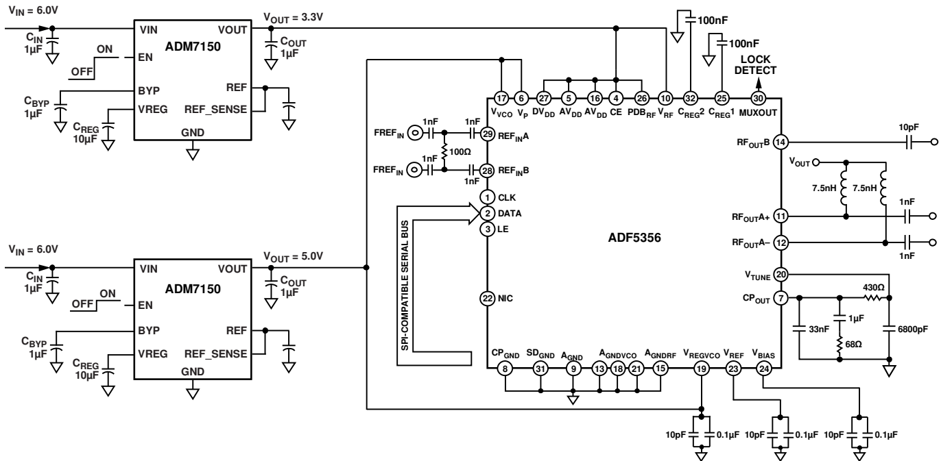
Figure 53. Power Supplies
