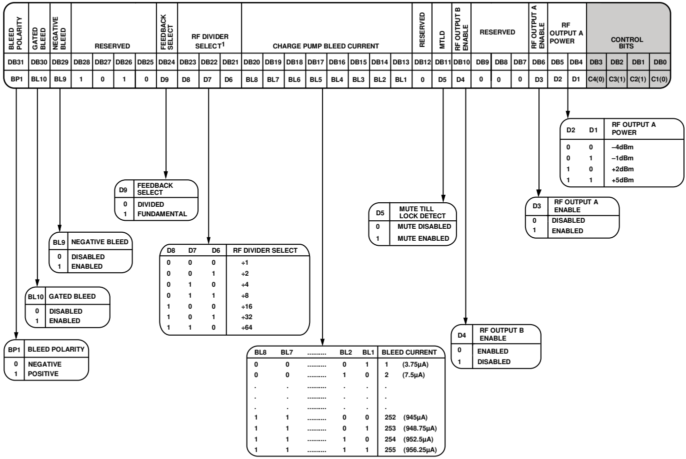
Figure 44. Register 6 Details
