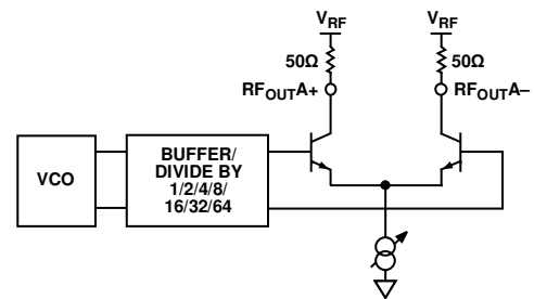
Figure 34. Output Stage
