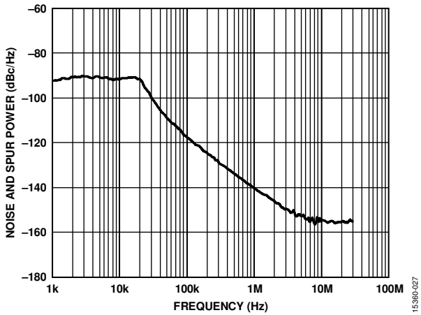
Figure 27. Fractional-N Spur Performance, R_{F_{OUT}A+} = 2.591 GHz, f_{REFIN} = 122.88 MHz, f_{PPD} = 61.44 MHz, Output Divide by 2 Selected, Loop Filter Bandwidth = 10 kHz, Channel Spacing = 20 kHz
