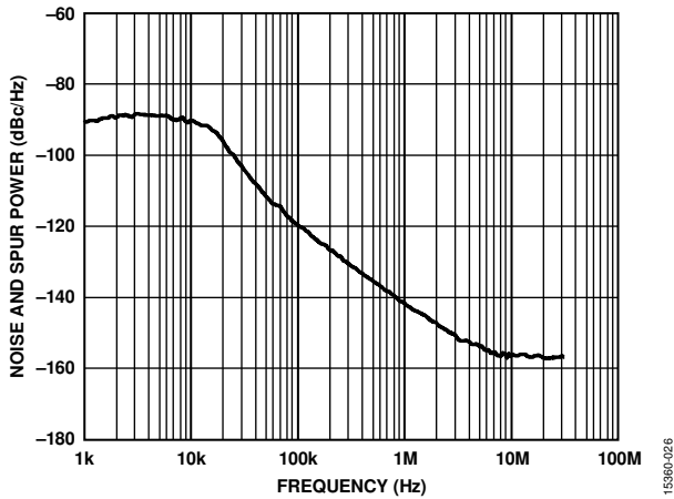
Figure 26. Fractional-N Spur Performance, W-CDMA Band, R_{F_{OUT}A+} = 2113.5 MHz, f_{REFIN} = 122.88 MHz, f_{PPD} = 61.44 MHz, Output Divide by 2 Selected, Loop Filter Bandwidth = 10 kHz, Channel Spacing = 20 kHz
