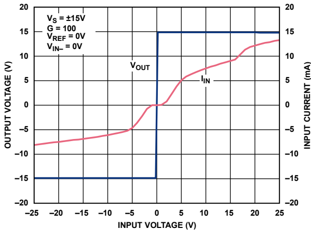
Figure 18. Input Overvoltage Performance; G = 100 , V_S = \pm 15V
