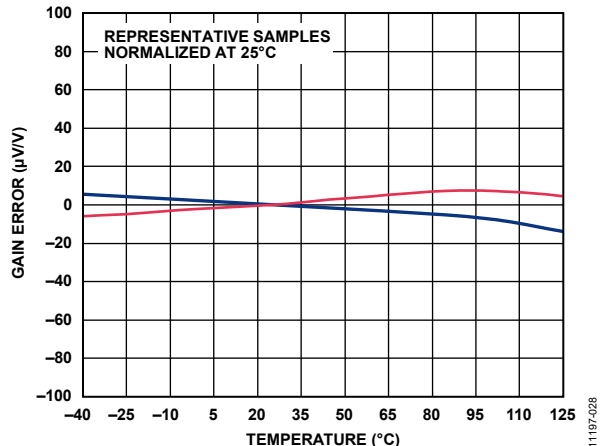
Figure 28. Gain vs. Temperature ( G = 1 )
