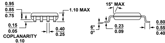
COMPLIANT TO JEDEC STANDARDS MO-187-AA Figure 67. 8-Lead Mini Small Outline Package [MSOP] (RM-8) Dimensions shown in millimeters
