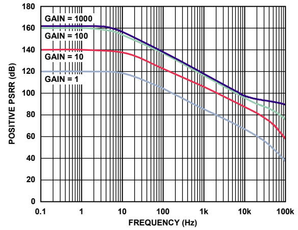
Figure 21. Positive PSRR vs. Frequency
