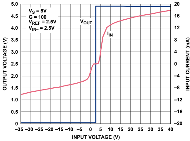
Figure 17. Input Overvoltage Performance; G = 100 , V_S = 5V
