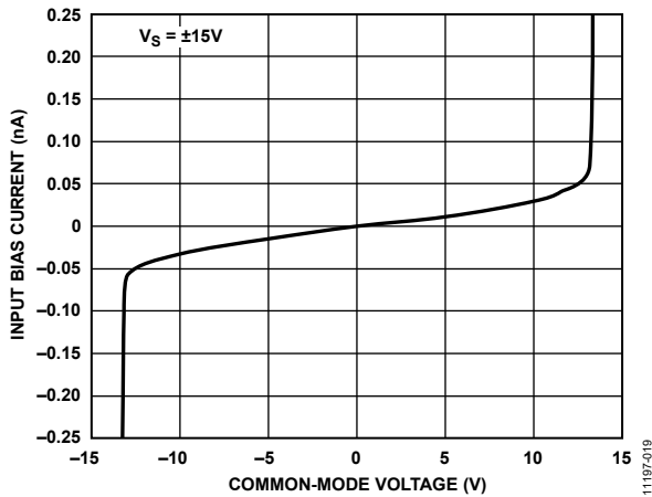
Figure 19. Input Bias Current vs. Common-Mode Voltage, V_S = \pm 15V
