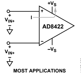
Figure 61. Input Overvoltage Protection with no External Components
