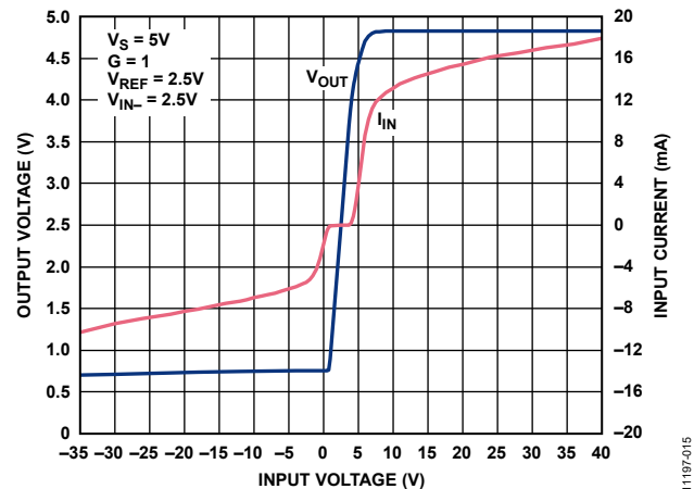
Figure 15. Input Overvoltage Performance; G = 1 , V_S = 5\text{ V}
