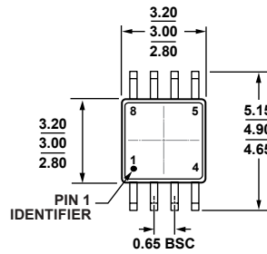
Figure 66. 8-Lead Standard Small Outline Package [SOIC_N] Narrow Body (R-8) Dimensions shown in millimeters and (inches)
