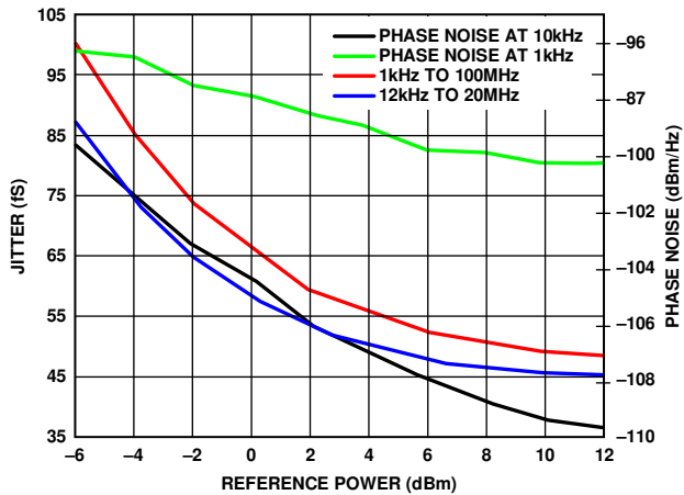
Figure 28. Jitter and Phase Noise, f_{\text{PFD}} = 100 \text{ MHz}
