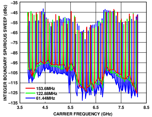
Figure 16. Integer Boundary Spurious Sweep vs. Carrier Frequency, f_{PFD} = 61.44 MHz, 122.88 MHz, and 153.6 MHz, Loop Filter Bandwidth = 100 kHz
