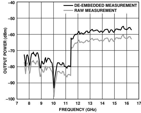
Figure 25. RF16P and RF16N Output Power When Disabled, De-Embedded Board and Cable Measurement, Combined Using Balun
