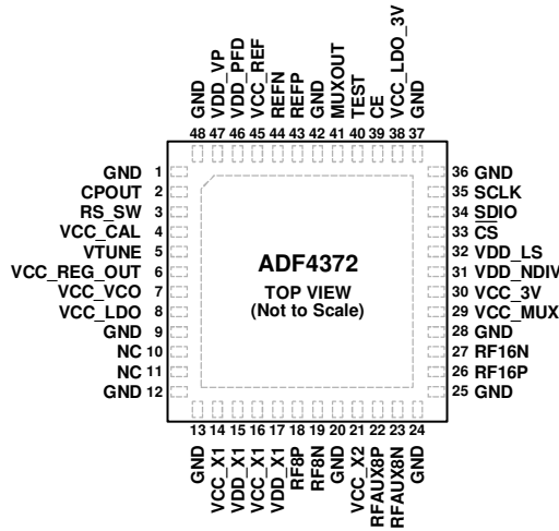
Figure 6. Pin Configuration
