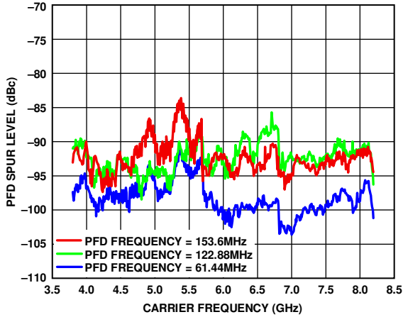
Figure 14. PFD Spurious Sweep, f_{PFD} = 61.44 MHz, Loop Filter Bandwidth = 100 kHz
