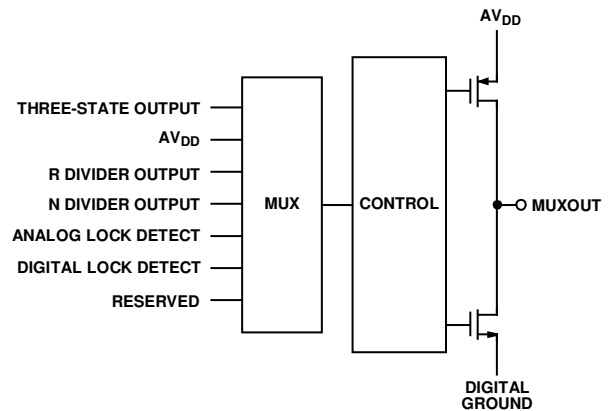
Figure 32. MUXOUT Schematic
