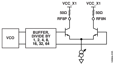
Figure 35. Output Stage
