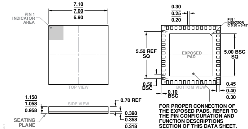
Figure 38. 48-Terminal Land Grid Array Package [LGA] (CC-48-4) Dimensions shown in millimeters
