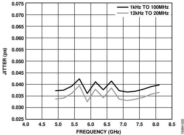
Figure 21. RMS Jitter, Integer-N, f_{PFD} = 245.76 MHz, Loop Filter Bandwidth = 220 kHz, V_{CC\_VCO} = 5 V
