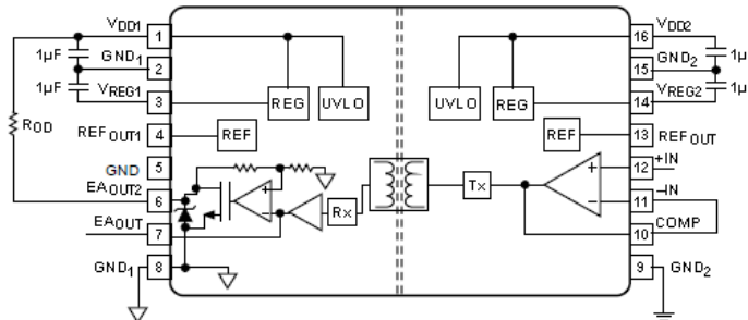
Figure 5. Test Circuit 3: Isolated Amplifier Circuit ADuM3190S rev. C. Page 8 of 14
