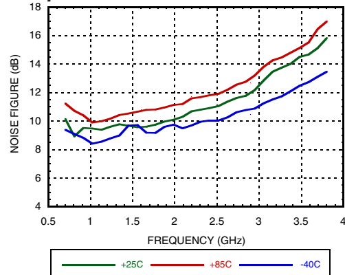
Figure 24. High Side LO Noise Figure vs. Temperature at VGATE=5V
