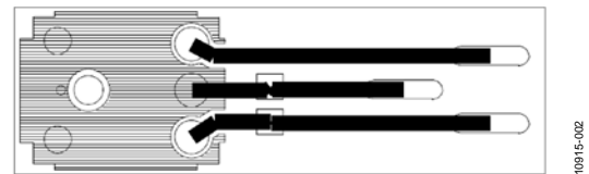
Figure 2. Evaluation Board Layout (Top View)
