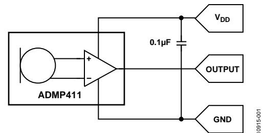
Figure 1. Evaluation Board Schematic
