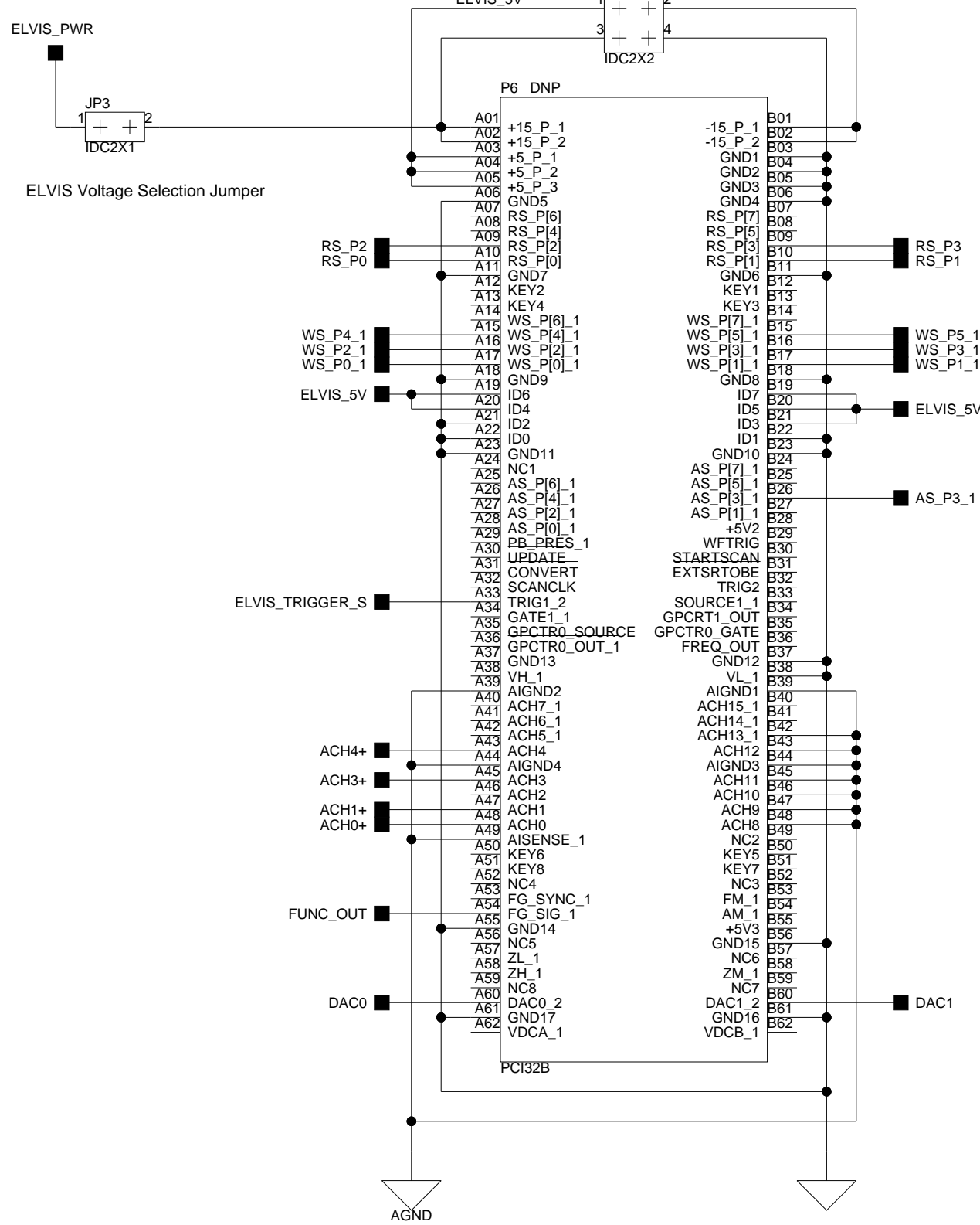
ELVIS CONNECTOR
