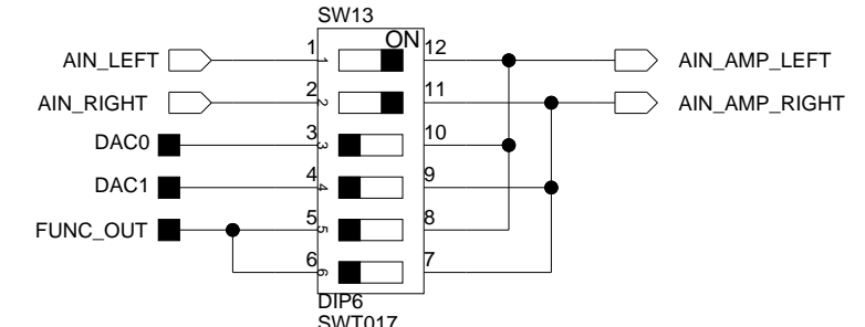
Function Generator Switch
