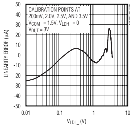
ACTIVE-LOAD LINEARITY ERROR I_{DUT\_} vs. V_{LDL\_}
