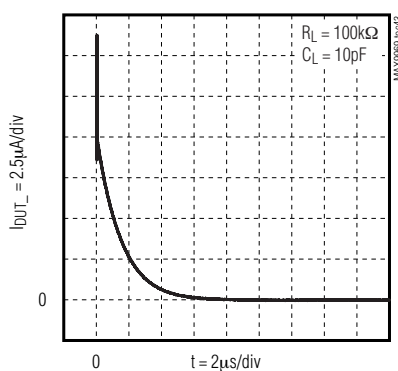
DRIVE 1V TO LOW-LEAKAGE TRANSITION
