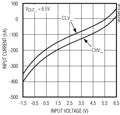
COMPARATOR REFERENCE CURRENT vs. INPUT VOLTAGE
