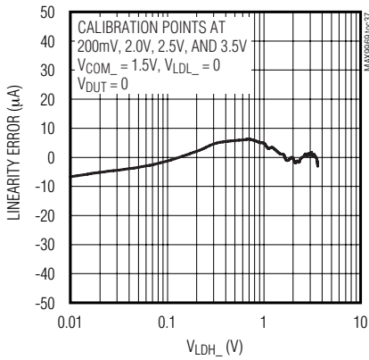
ACTIVE-LOAD LINEARITY ERROR I_{DUT\_} vs. V_{LDH\_}
