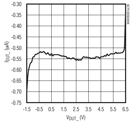
HIGH-IMPEDANCE CURRENT vs. DUT\_ VOLTAGE
