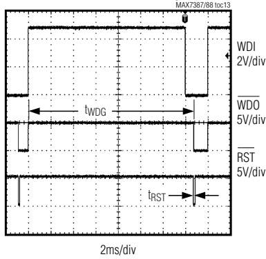
RESPONSE OF \overline{RST} AND \overline{WDO} WDI EXCEEDING t_{WDG}
