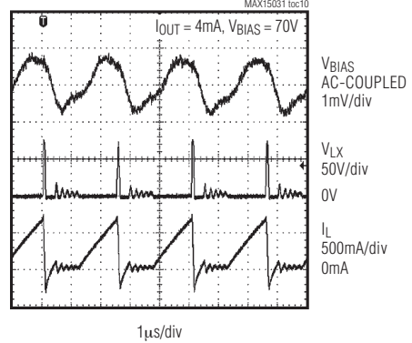
HEAVY-LOAD SWITCHING WAVEFORM WITH RC FILTER
