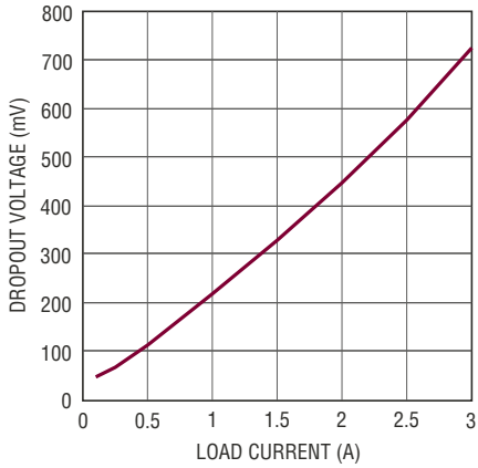
压差电压
