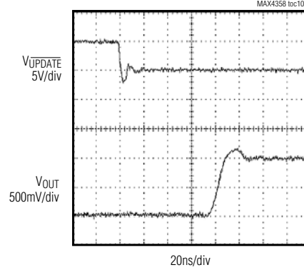
SWITCHING TIME
