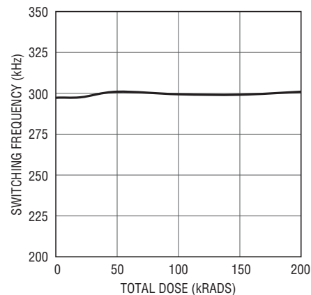
Operating Switching Frequency vs TID
