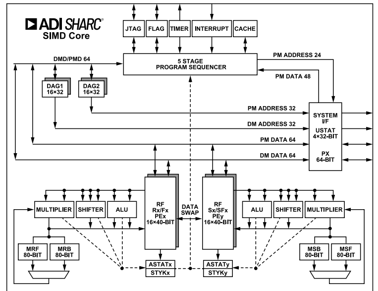
Figure 38. SHARC Core Block Diagram
