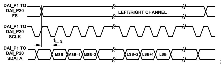
Figure 24. Left-Justified Mode
