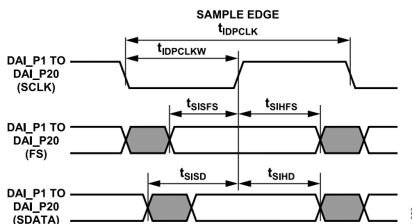
Figure 17. IDP Main Timing
