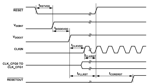
Figure 2. Power-Up Sequencing
