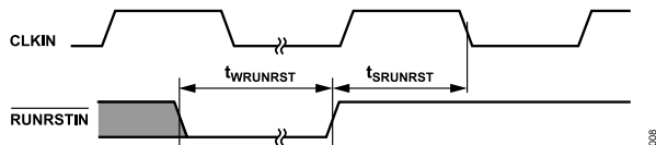
Figure 5. Running Reset
