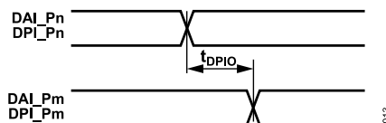
Figure 10. DAI/DPI Pin to Pin Routing
