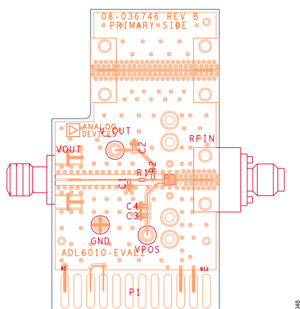
Figure 48. Evaluation Board Layout, Top Side
