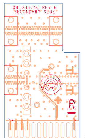
Figure 49. Evaluation Board Layout, Bottom Side
