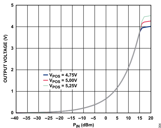
Figure 6. Output Voltage ( V_{OUT} ) vs. RF Input Power ( P_{IN} ) for Various Supply Voltages
