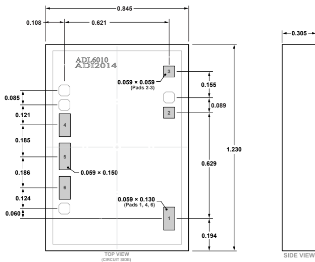
Figure 51. 6-Pad Bare Die [CHIP] (C-6-14)
