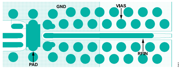
Figure 41. ADL6010 Evaluation Board
