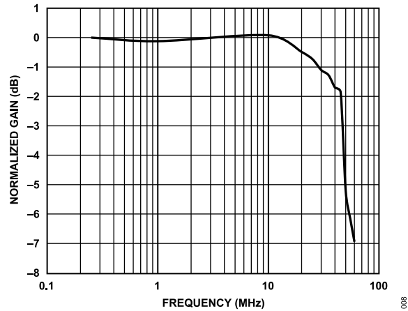
Figure 10. Envelope Bandwidth of V_{OUT} vs. Frequency at P_{IN} = -10 dBm and Modulation Depth = 10% (See Figure 39 in the Measurement Setups Section)
