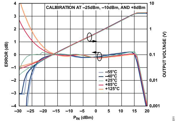
Figure 13. Conformance Error and Output Voltage ( V_{OUT} ) vs. RF Input Power ( P_{IN} ) for Various Temperatures at 5 GHz
