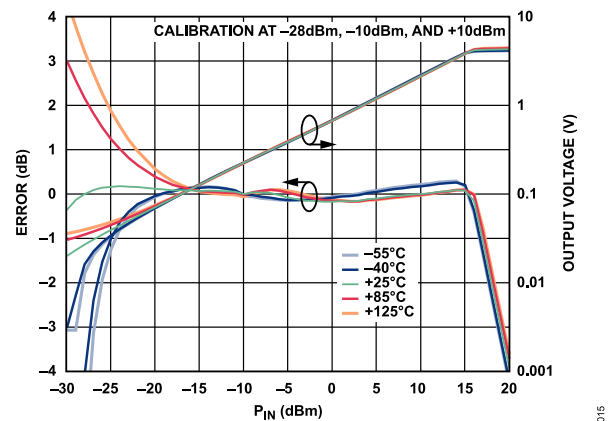
Figure 14. Conformance Error and Output Voltage ( V_{OUT} ) vs. RF Input Power ( P_{IN} ) for Various Temperatures at 10 GHz
