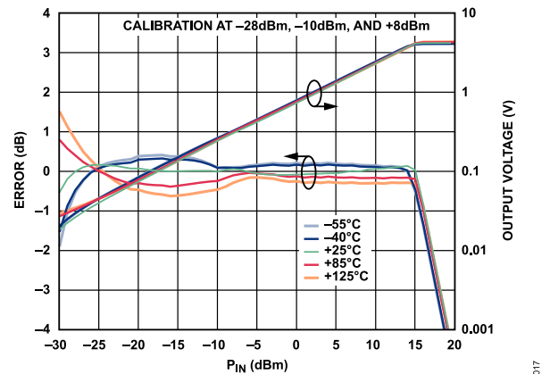
Figure 19. Conformance Error and Output Voltage ( V_{OUT} ) vs. RF Input Power ( P_{IN} ) for Various Temperatures at 20 GHz
