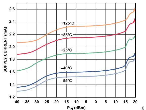
Figure 9. Supply Current vs. RF Input Power ( P_{IN} ) for Various Temperatures
