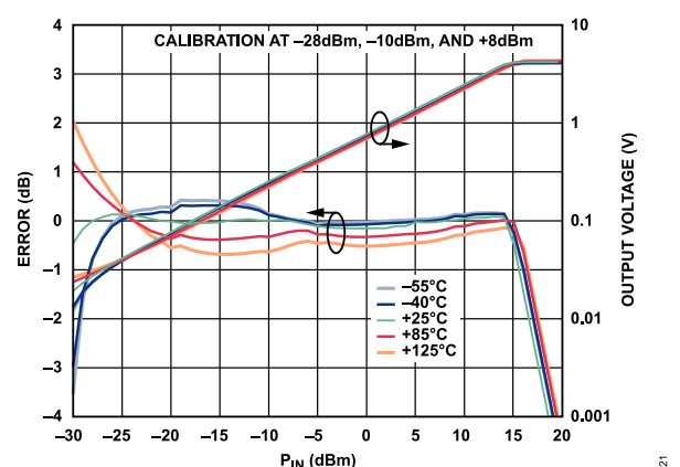
Figure 20. Conformance Error and Output Voltage ( V_{OUT} ) vs. RF Input Power ( P_{IN} ) for Various Temperatures at 25 GHz
