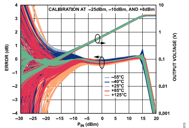
Figure 15. Distribution of Conformance Error with Respect to Output Voltage ( V_{OUT} ) at 25°C vs. RF Input Power ( P_{IN} ) for Various Temperatures at 1 GHz
