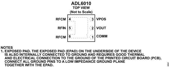
Figure 2. 6-Lead LFCSP Pin Configuration
