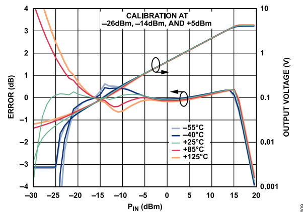
Figure 8. Conformance Error and Output Voltage ( V_{OUT} ) vs. RF Input Power ( P_{IN} ) for Various Temperatures at 0.5 GHz
