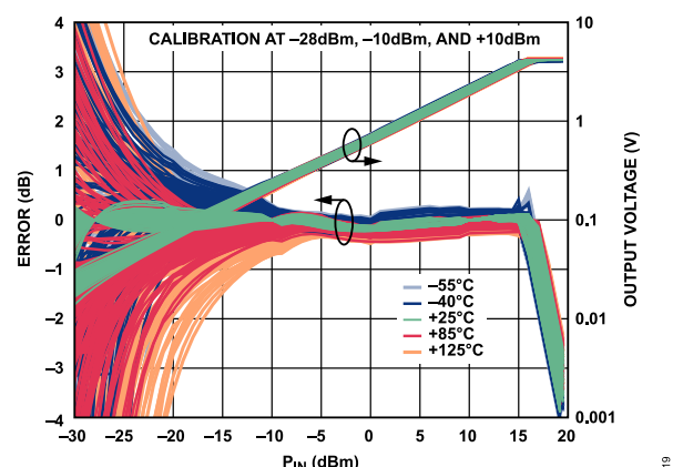
Figure 21. Distribution of Conformance Error with Respect to Output Voltage ( V_{OUT} ) at 25°C vs. RF Input Power ( P_{IN} ) for Various Temperatures at 15 GHz
