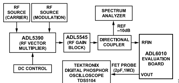
Figure 39. Hardware Configuration for Envelope Output Response Measurement
