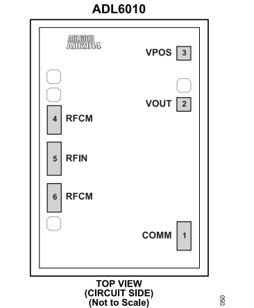
Figure 3. 6-Pad Bare Die Pin Configuration
