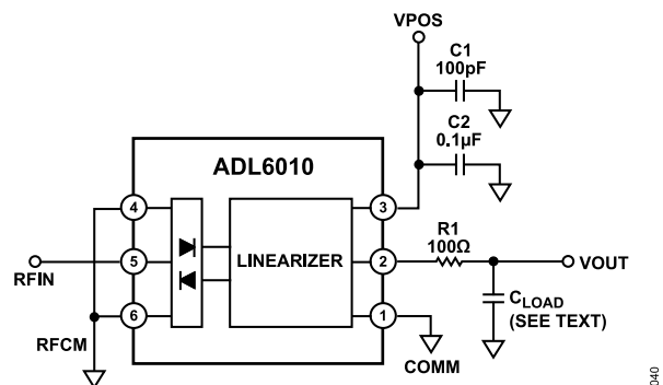
Figure 40. Basic Connections
