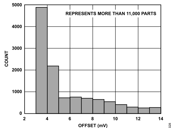
Figure 30. Distribution of V_{OUT} Offset with No Applied P_{IN} at 25°C
