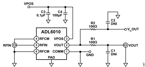
Figure 47. ADL6010 Evaluation Board Schematic
