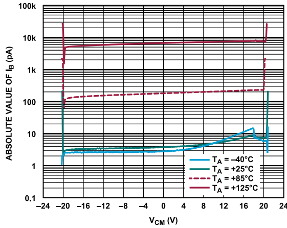
Figure 22. I_B vs. V_{CM} , Four Temperatures, SOIC_N
