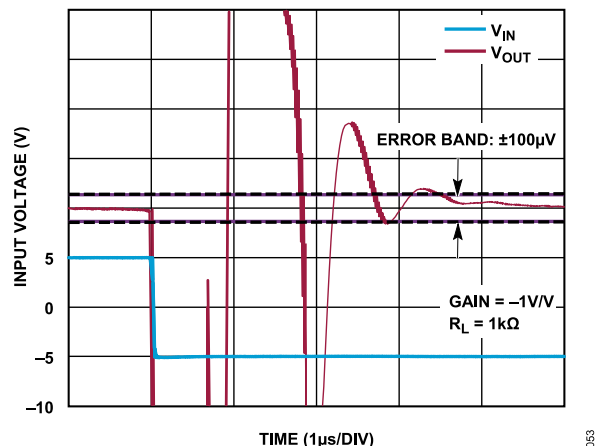
Figure 56. Negative Step Settling Time to 0.001%, V_{OUT} = 10\text{ V}
