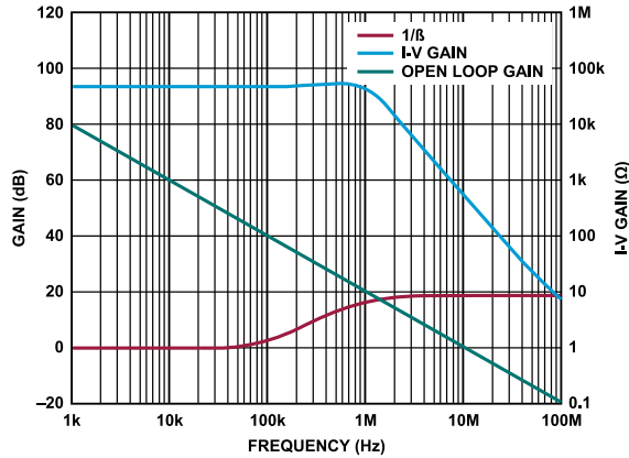
Figure 84. Compensating the TIA, C_F = 3.1 \text{ pF}
