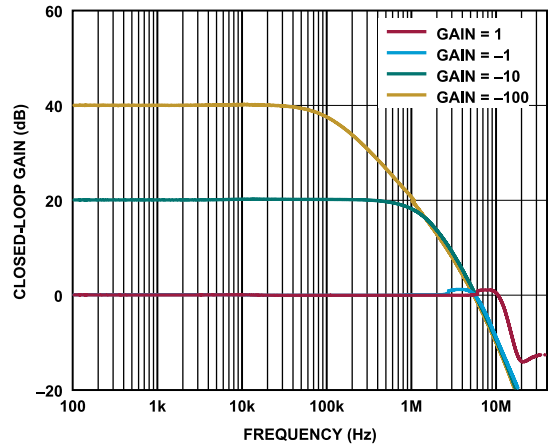
Figure 36. Closed-Loop Gain vs. Frequency
