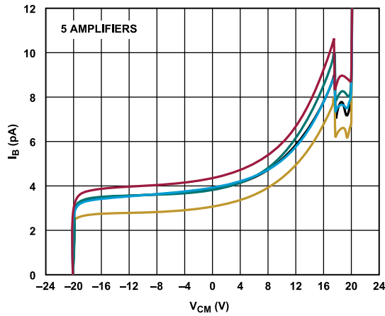
Figure 23. I_B vs. V_{CM}
