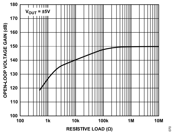
Figure 74. DC Open-Loop Gain vs. R_L
