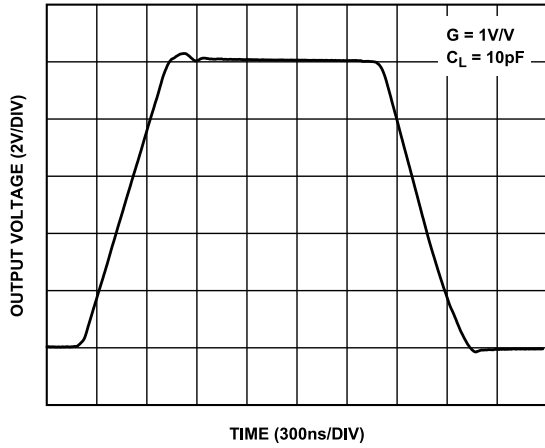
Figure 63. Large Signal Transient Response, G = 1\text{ V/V}
