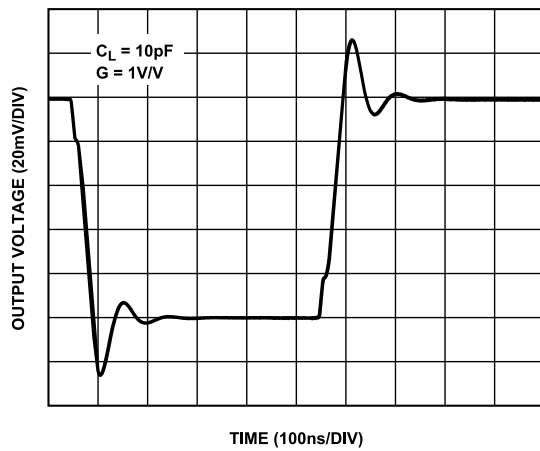
Figure 58. Small Signal Transient Response, G = 1\text{ V/V}
