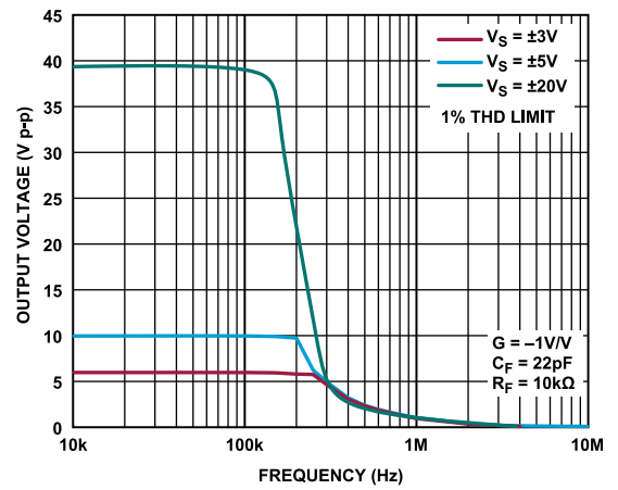
Figure 43. Maximum Undistorted Output Swing vs. Frequency
