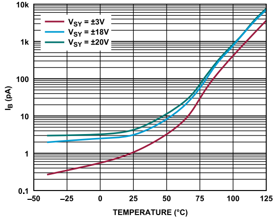
Figure 21. I_B vs. Temperature, SOIC_N
