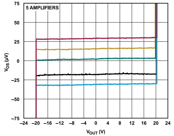
Figure 31. V_{OS} vs. V_{OUT}
