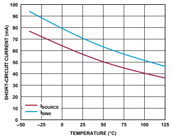
Figure 49. Short-Circuit Output Current vs. Temperature
