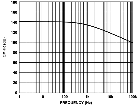
Figure 39. CMRR vs. Frequency
