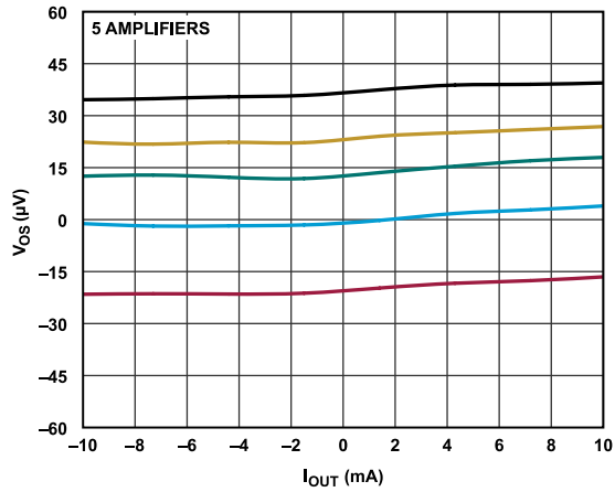
Figure 28. V_{OS} vs. I_{OUT}
