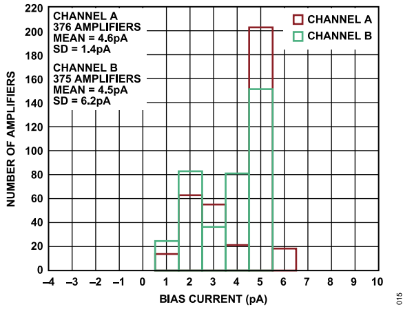
Figure 16. I_B Distribution at -40°C
