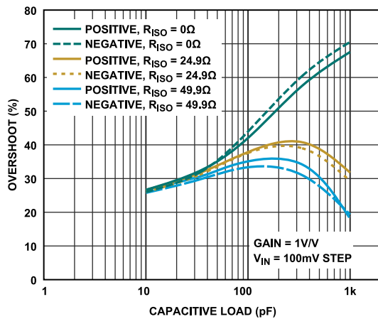
Figure 59. Overshoot vs. Capacitance Load, G = 1\text{ V/V}
