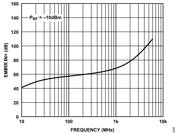
Figure 26. EMIRR IN+ vs. Frequency ( P_{RF} = RF Power)
