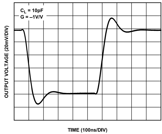
Figure 61. Small Signal Transient Response, G = -1\text{ V/V}
