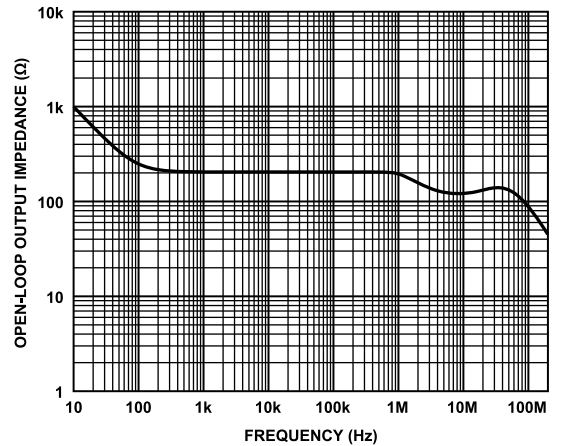
Figure 32. Z_O vs. Frequency
