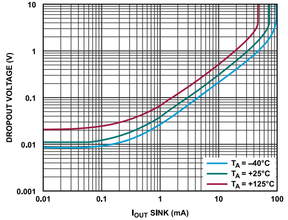
Figure 30. V_{DROPOUT}(V_{OUT} - (V-)) vs. I_{OUT} Sink
