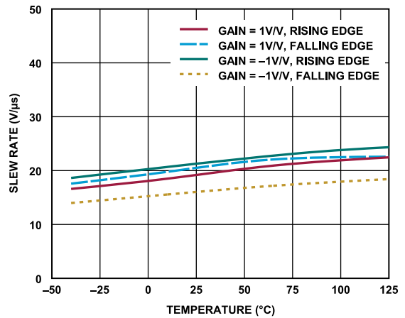
Figure 67. Slew Rate vs. Temperature
