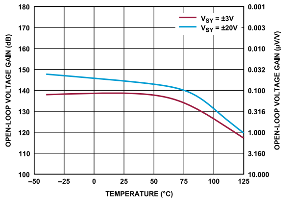
Figure 71. DC Open-Loop Gain vs. Temperature
