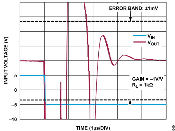
Figure 55. Negative Step Settling Time to 0.01%, V_{OUT} = 10\text{ V}
