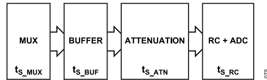
Figure 79. Block Diagram for Settling Time Analysis
