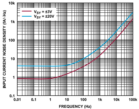
Figure 68. Current Noise Spectral Density vs. Frequency
