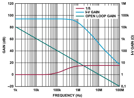
Figure 85. Compensating the TIA, C_F = 5.5 \text{ pF}
