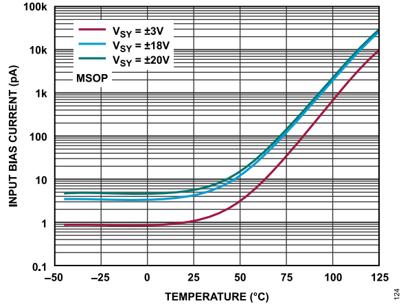
Figure 24. I_B vs. Temperature, MSOP
