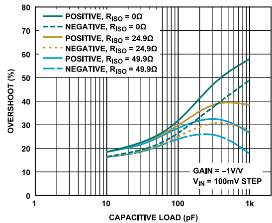
Figure 62. Overshoot vs. Capacitance Load, G = -1\text{ V/V}
