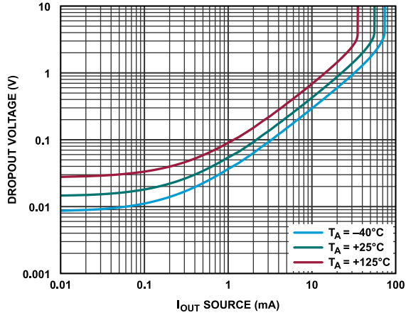
Figure 27. V_{DROPOUT}(V+) - V_{OUT} vs. I_{OUT} Source
