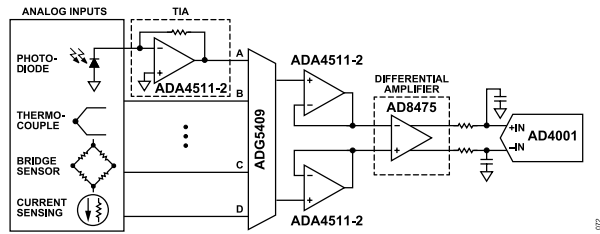
Figure 76. Multiplexed Data Acquisition System
