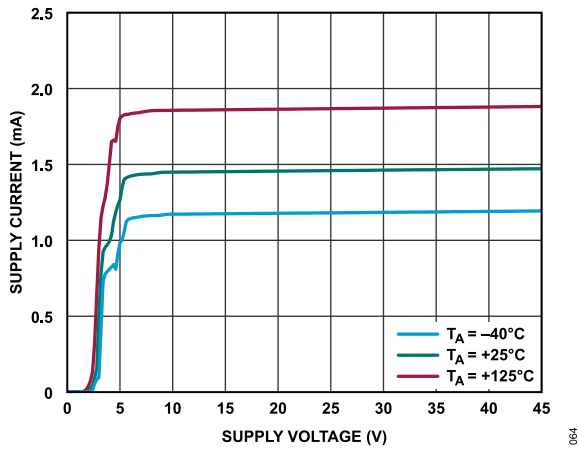
Figure 70. I_S per Amplifier vs. Supply Voltage at Various Temperatures
