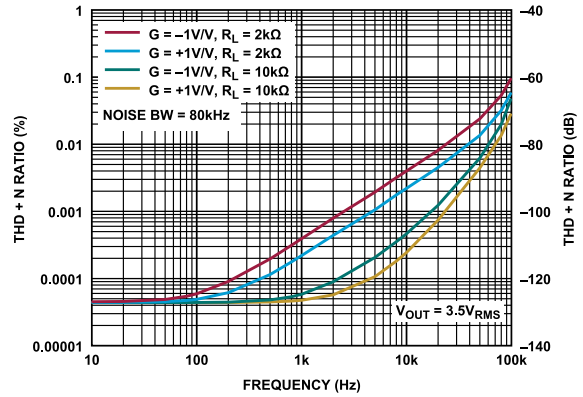
Figure 48. THD + N vs. Frequency
