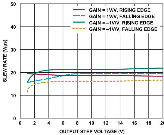
Figure 64. Slew Rate vs. Output Step Voltage
