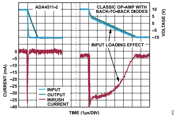
Figure 77. ADA4511-2 Inrush Current Reduction
