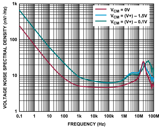
Figure 65. Input Voltage Noise Spectral Density vs. Frequency
