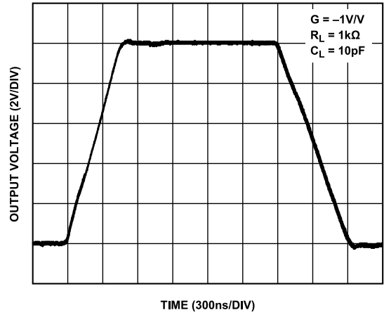
Figure 66. Large Signal Transient Response, G = -1\text{ V/V}
