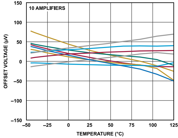
Figure 9. V_{OS} vs. Temperature, SOIC_N
