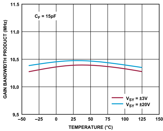
Figure 34. Gain Bandwidth Product vs. Temperature
