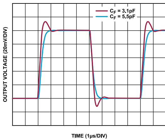
Figure 86. Pulse Response for Various C_F
