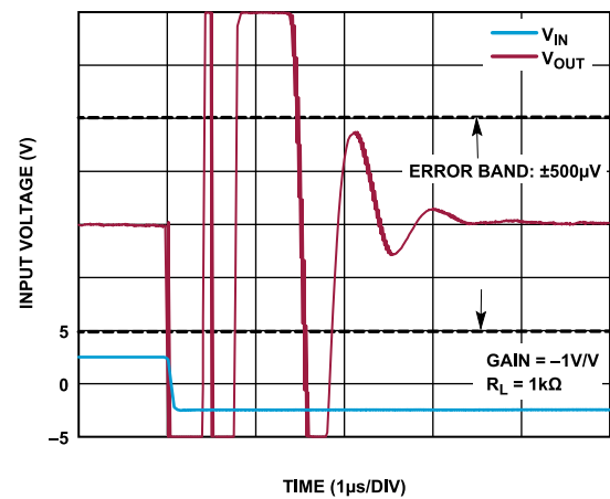
Figure 50. Negative Step Settling Time to 0.01%, V_{OUT} = 5\text{ V}
