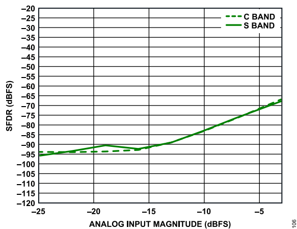
Figure 101. Single-Tone SFDR (Excluding Second and Third Harmonics and f_{s/2} - A_{1N} ) vs. Analog Input Magnitude
