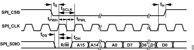
Figure 3. Timing Diagram for 3-Wire Operation
