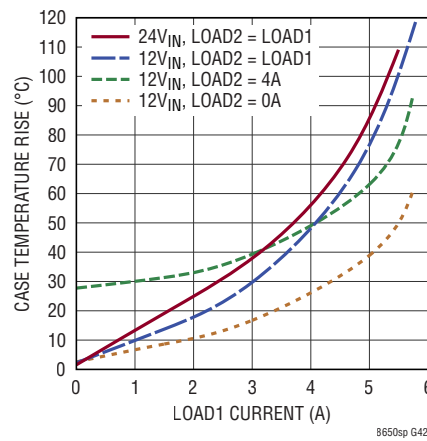
Case Temperature Rise without Heat Sink
