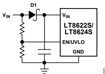
Figure 63. Reverse V_{IN} Protection
