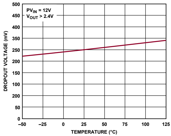
Figure 25. SV_{IN} Dropout Voltage
