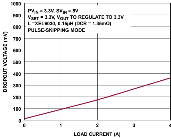
Figure 22. PV_{IN} Dropout Voltage
