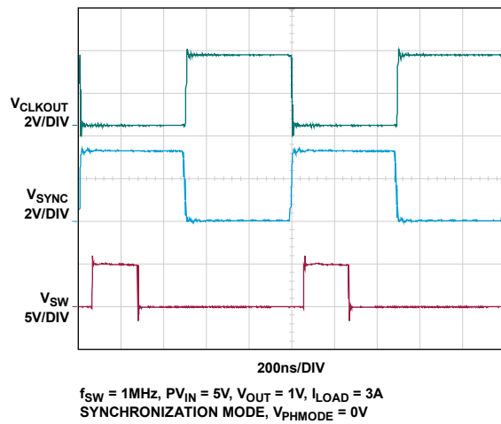
Figure 43. CLKOUT Waveforms
