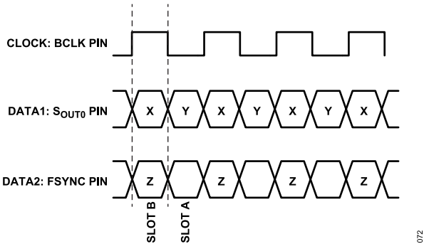
Figure 72. Example PDM Port Data Format
