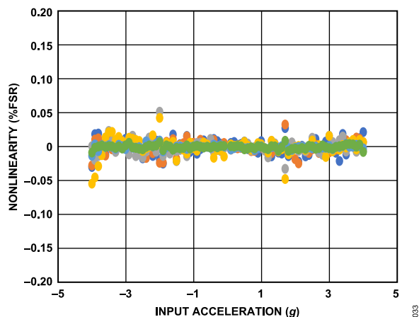
Figure 33. Z-axis \pm 4 g Nonlinearity at 25°C, Measured Across 6 Samples, V_S = 3.3 V
