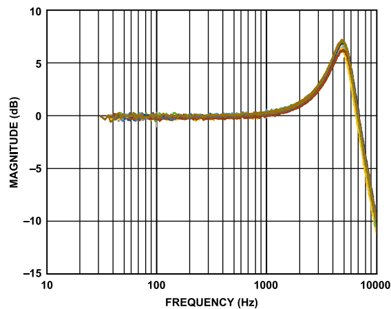
Figure 28. X-Axis PDM Frequency Response at 25°C, Measured Across 9 Samples, V_S = 3.3\text{ V}
