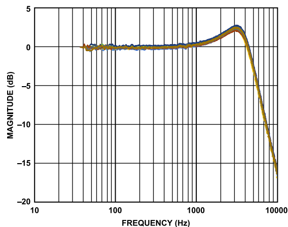
Figure 30. Z-Axis PDM Frequency Response at 25°C, Measured Across 9 Samples, V_S = 3.3\text{ V}
