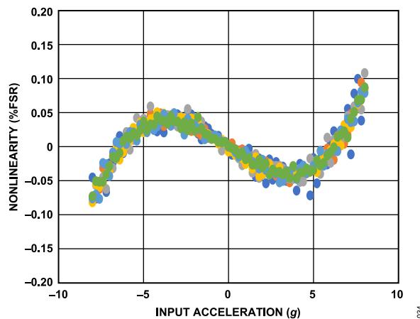
Figure 34. X-axis \pm 8 g Nonlinearity at 25°C, Measured Across 6 Samples, V_S = 3.3 V
