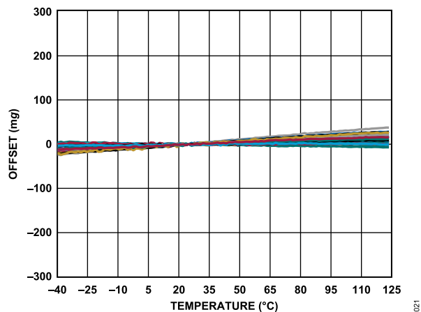
Figure 21. Z-Axis Offset vs. Temperature, Measured Across 48 Samples, V_S = 3.3\text{ V}
