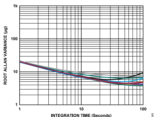
Figure 45. Z-Axis Root Allan Variance at 25°C, Measured Across 12 Samples, V_S = 3.3\text{ V}
