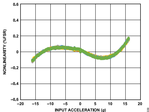
Figure 39. Z-Axis \pm 16 g Nonlinearity at 25^{\circ}\text{C} , Measured Across 6 Samples, V_S = 3.3 V
