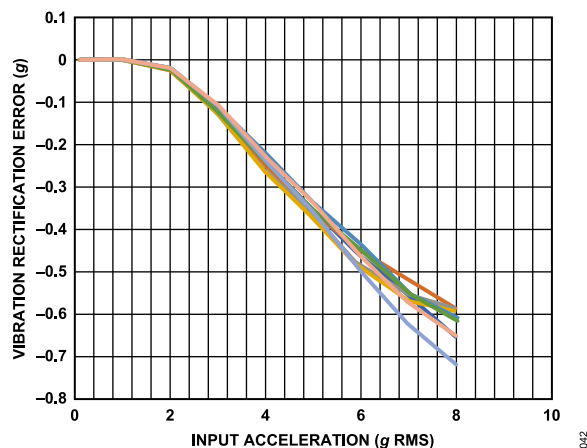
Figure 42. Z-Axis Vibration Rectification Error, Z-Axis in +1 g Field, \pm 4 g Range, Measured Across 8 Samples, V_S = 3.3 V
