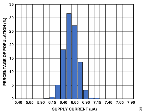
Figure 56. Standby Mode Supply Current at 25°C, V_S = 3.3 V
