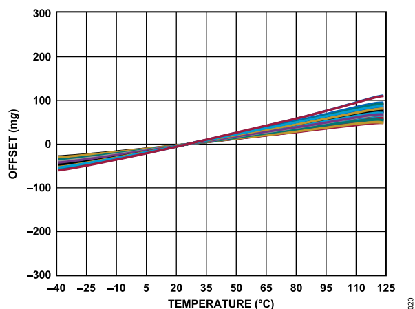
Figure 20. Y-Axis Offset vs. Temperature, Measured Across 48 Samples, V_S = 3.3\text{ V}
