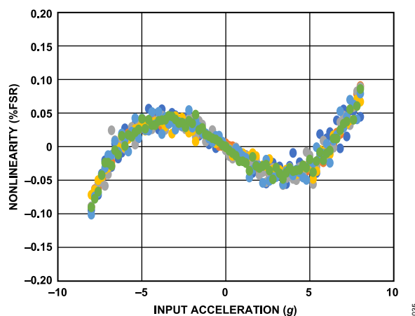
Figure 35. Y-axis \pm 8 g Nonlinearity at 25°C, Measured Across 6 Samples, V_S = 3.3 V
