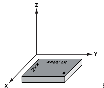
Figure 59. Axes of Acceleration Sensitivity
