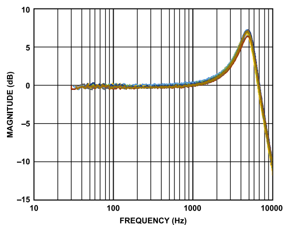
Figure 29. Y-Axis PDM Frequency Response at 25°C, Measured Across 9 Samples, V_S = 3.3\text{ V}
