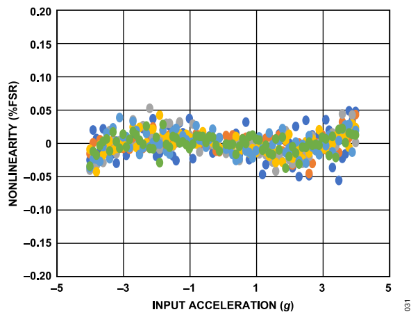
Figure 31. X-axis \pm 4 g Nonlinearity at 25°C, Measured Across 6 Samples, V_S = 3.3 V
