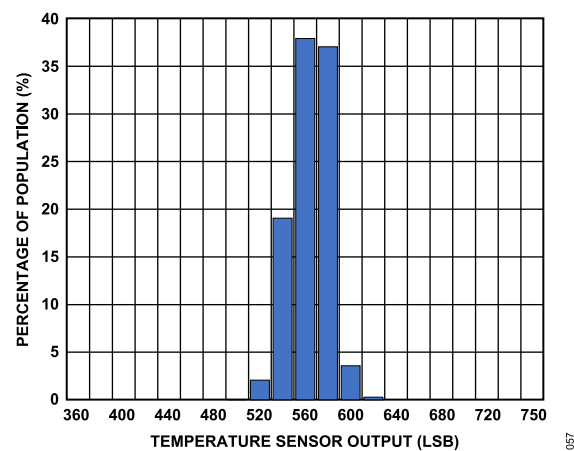
Figure 57. Temperature Sensor Output at 25°C, HIGH\_GAIN\_TEMP = 0 , V_S = 3.3 V
