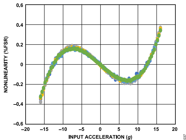
Figure 37. X-Axis \pm 16 g Nonlinearity at 25^{\circ}\text{C} , Measured Across 6 Samples, V_S = 3.3 V
