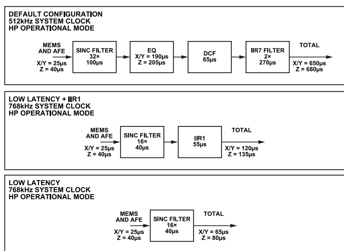
Figure 78. ADXL380 Latency vs. Filter Options
