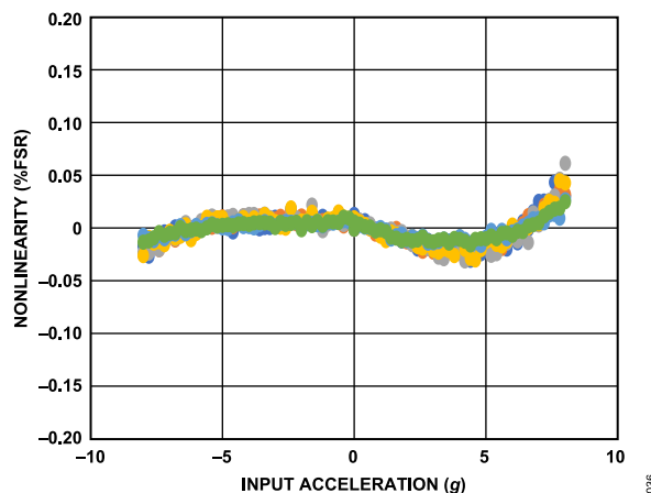
Figure 36. Z-axis \pm 8 g Nonlinearity at 25°C, Measured Across 6 Samples, V_S = 3.3 V
