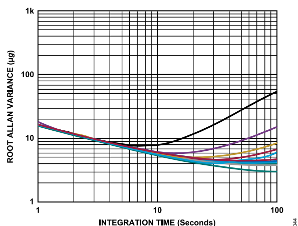
Figure 44. Y-Axis Root Allan Variance at 25°C, Measured Across 12 Samples, V_S = 3.3\text{ V}
