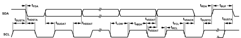
Figure 9. I²C Port Timing Diagram
