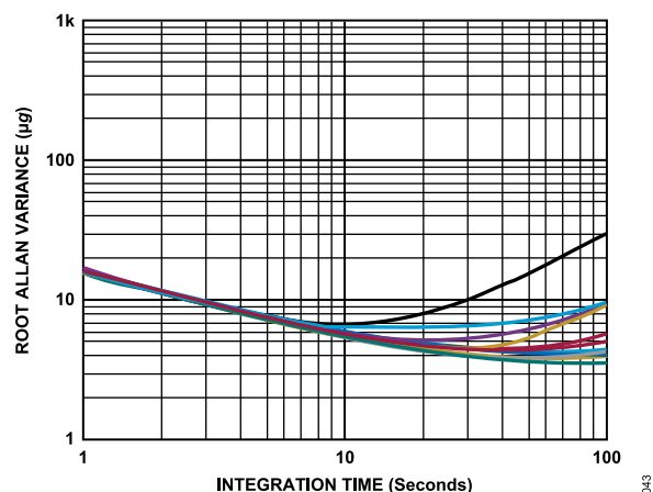
Figure 43. X-Axis Root Allan Variance at 25°C, Measured Across 12 Samples, V_S = 3.3\text{ V}
