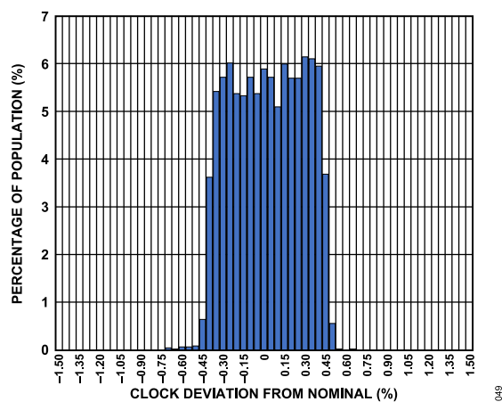
Figure 49. Clock Deviation from Nominal at 25°C, V_S = 3.3\text{ V}
