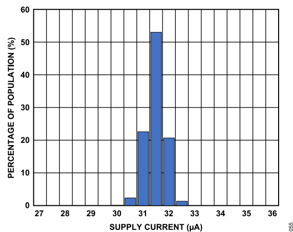
Figure 55. HS Mode Supply Current at 25°C, 1-Axis, V_S = 3.3 V
