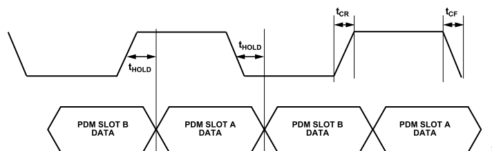
Figure 10. PDM Output Timing Diagram
