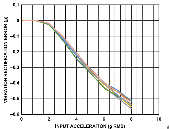
Figure 40. X-Axis Vibration Rectification Error, X-Axis in +1 g Field, \pm 4 g Range, Measured Across 8 Samples, V_S = 3.3 V
