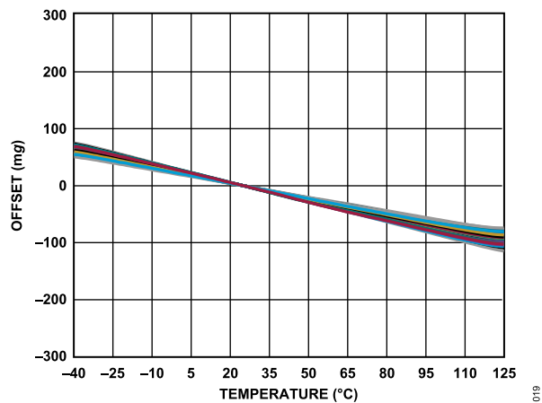
Figure 19. X-Axis Offset vs. Temperature, Measured Across 48 Samples, V_S = 3.3\text{ V}
