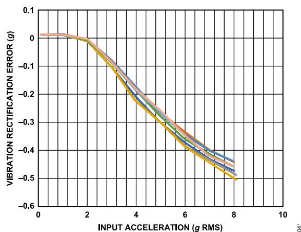
Figure 41. Y-Axis Vibration Rectification Error, Y-Axis in +1 g Field, \pm 4 g Range, Measured Across 8 Samples, V_S = 3.3 V
