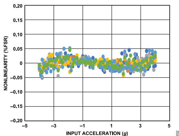
Figure 32. Y-axis \pm 4 g Nonlinearity at 25°C, Measured Across 6 Samples, V_S = 3.3 V
