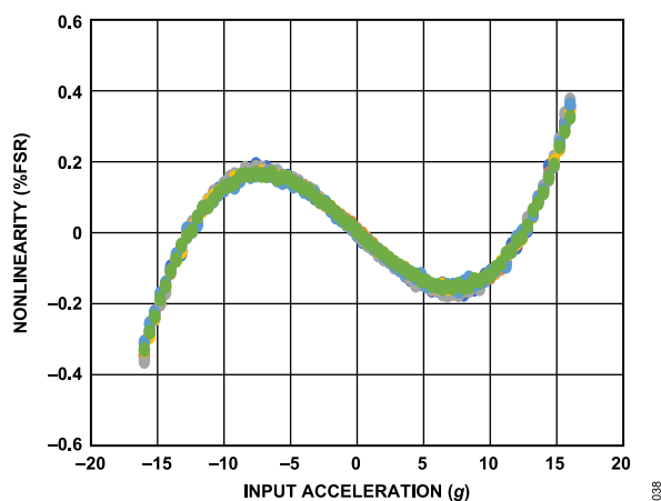
Figure 38. Y-Axis \pm 16 g Nonlinearity at 25^{\circ}\text{C} , Measured Across 6 Samples, V_S = 3.3 V
