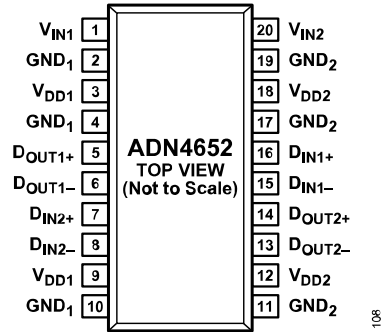
Figure 8. ADN4652 Pin Configuration
