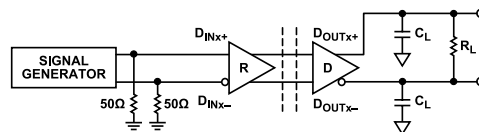
Figure 37. Timing Test Circuit
