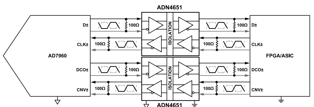
Figure 44. Example Isolated Analog Front-End Implementation (Isolated AD7960 Using the ADN4651)
