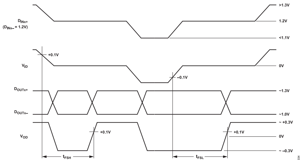
Figure 4. Fail-Safe Timing Diagram
