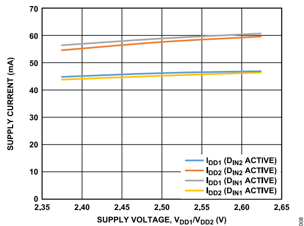
Figure 13. I_{DD1}/I_{DD2} Supply Current vs. Supply Voltage, V_{DD1}/V_{DD2}
