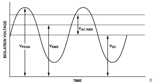
Figure 42. Critical Voltage Example
