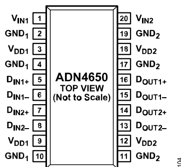
Figure 6. ADN4650 Pin Configuration
