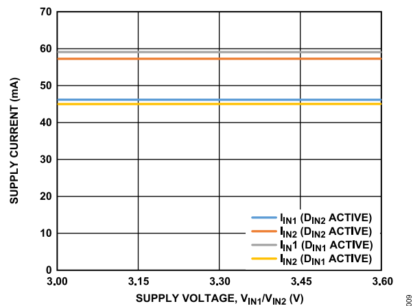
Figure 14. I_{IN1}/I_{IN2} Supply Current vs. Supply Voltage, V_{IN1}/V_{IN2}
