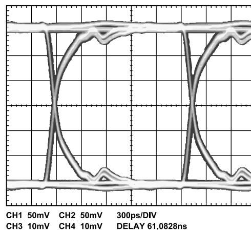
Figure 32. ADN4651 Eye Diagram for D_{OUT1\pm}
