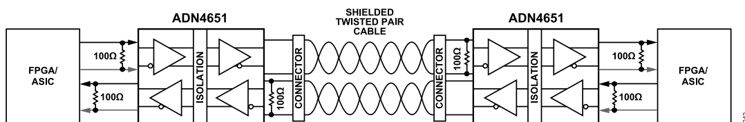
Figure 46. Example Isolated LVDS Cable Application Using the ADN4651
