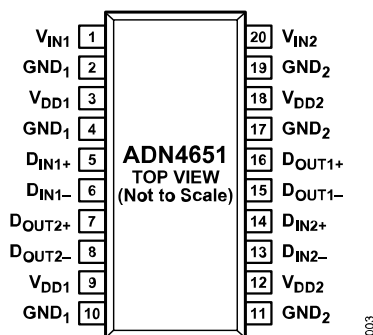
Figure 7. ADN4651 Pin Configuration
