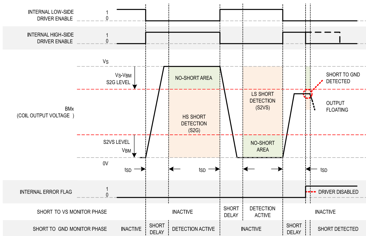
Figure 16: Short Detection (U/V/W Outputs)
