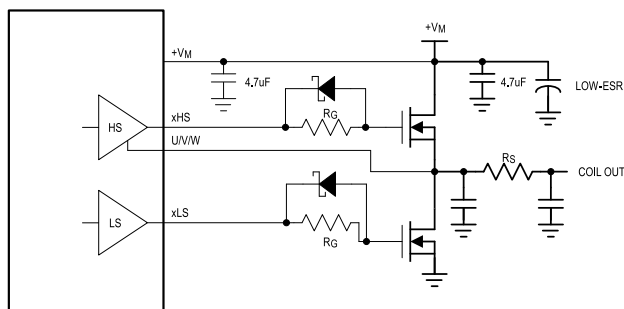
Figure 13: Bridge Design Example
