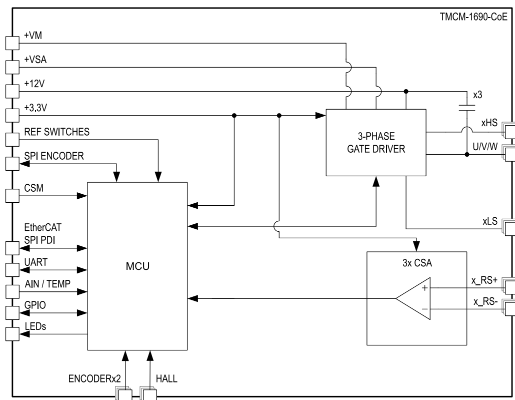
Figure 4: TMCM-1690-CoE System Architecture
