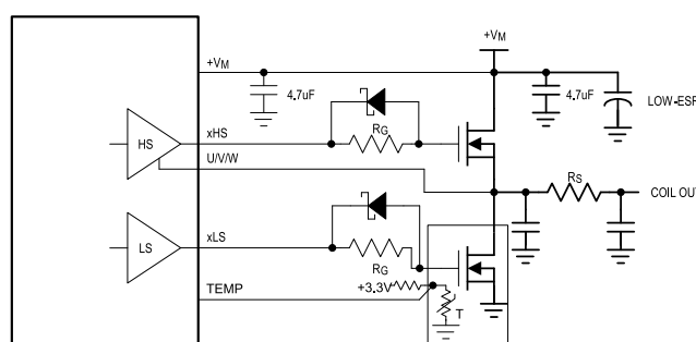
Figure 15: Thermistor Implementation
