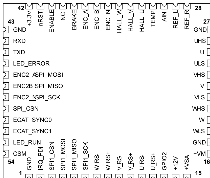
Figure 3: TMCM-1690-CoE Pinout (Top View)
