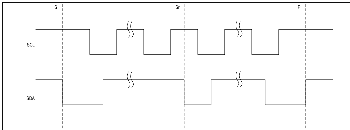
Figure 10. I²C START, STOP, and REPEATED START Conditions
