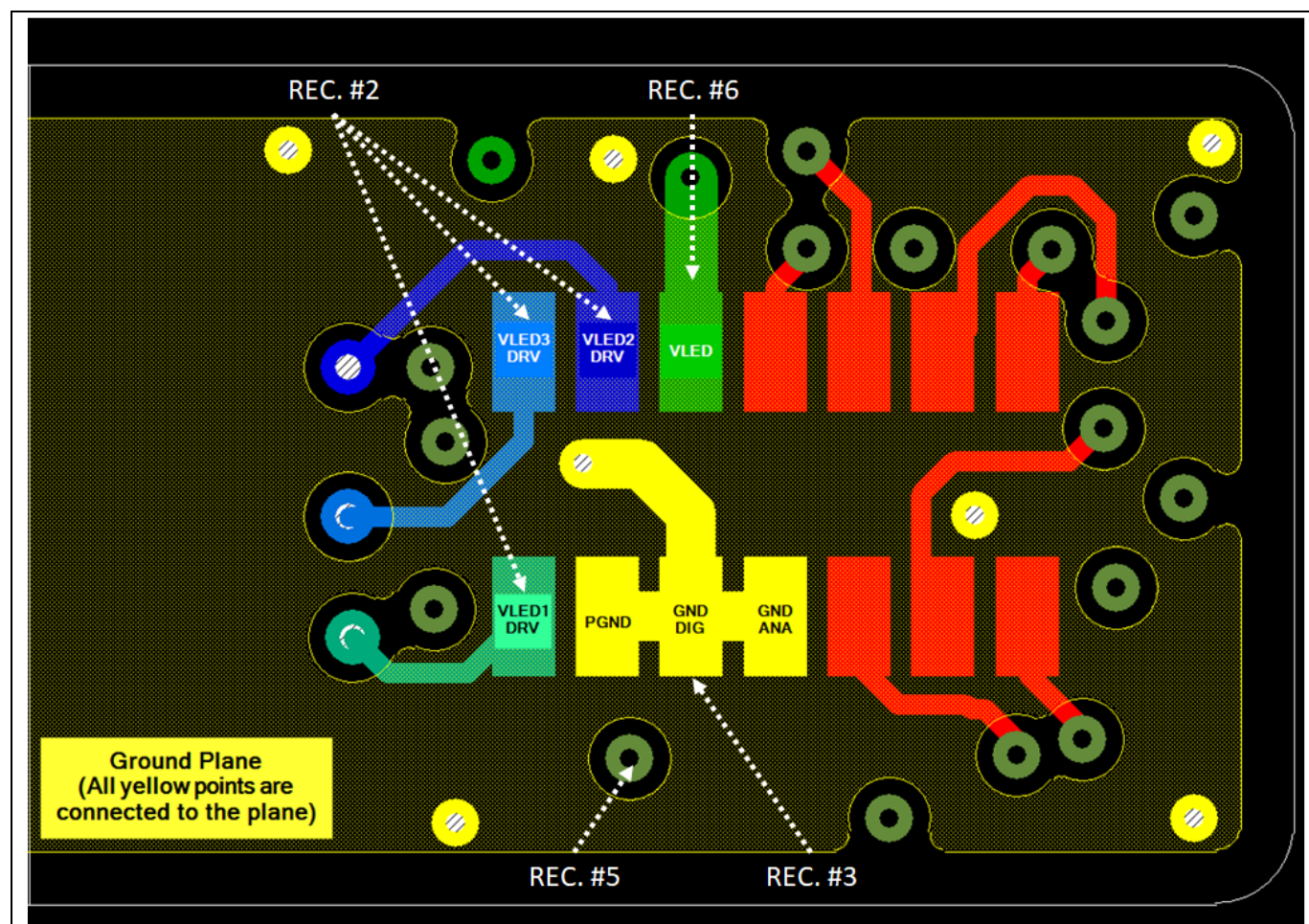
Figure 8. Layout Guideline
