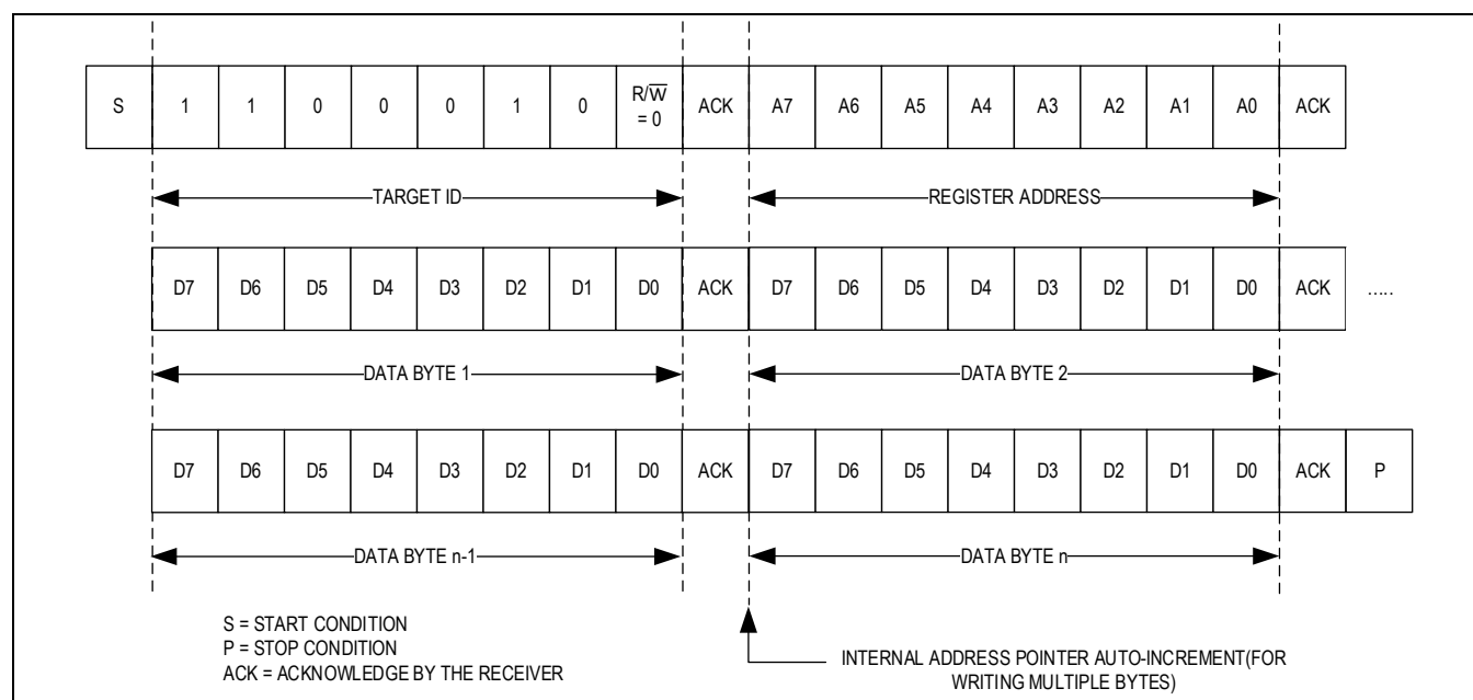
Figure 13. I 2 C Multi-Byte Write Transaction
