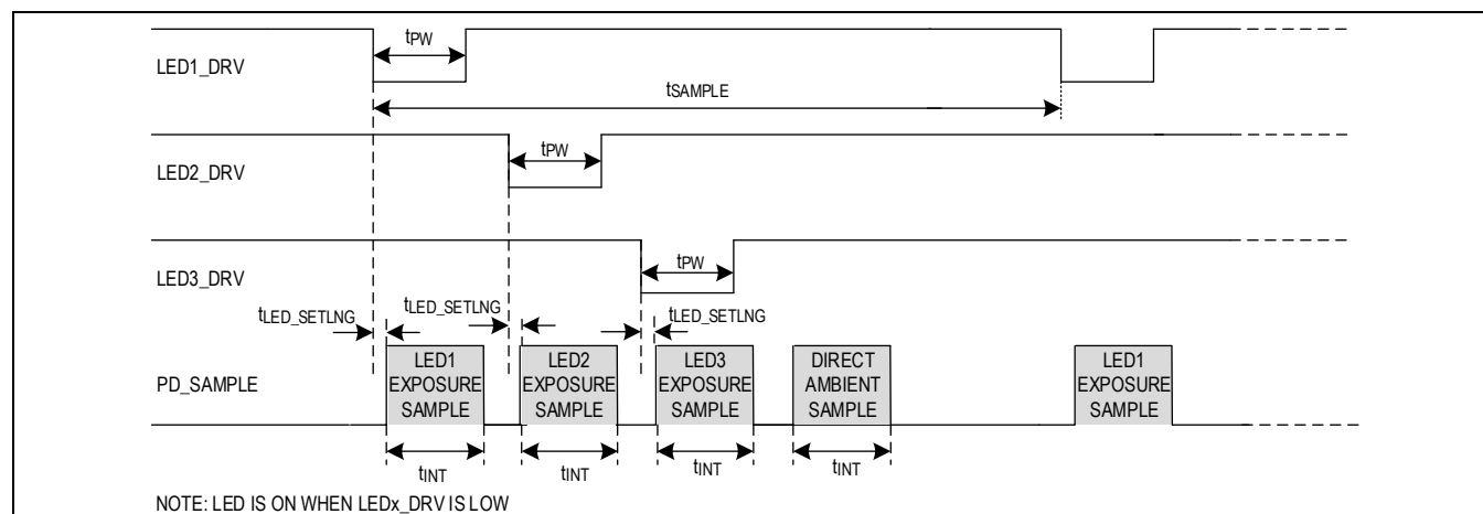
Figure 4. Timing for LED1, LED2, and LED3 Pulsing Sequentially with Direct Ambient Sampling
