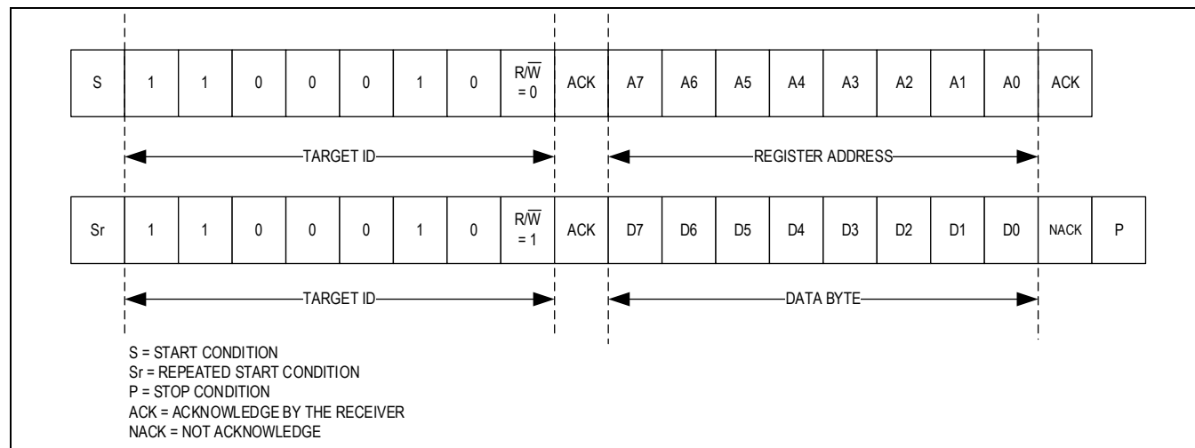
Figure 14. I 2 C Single Byte Read Transaction
