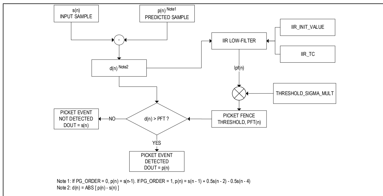
Figure 6. Picket Fence Function Flow
