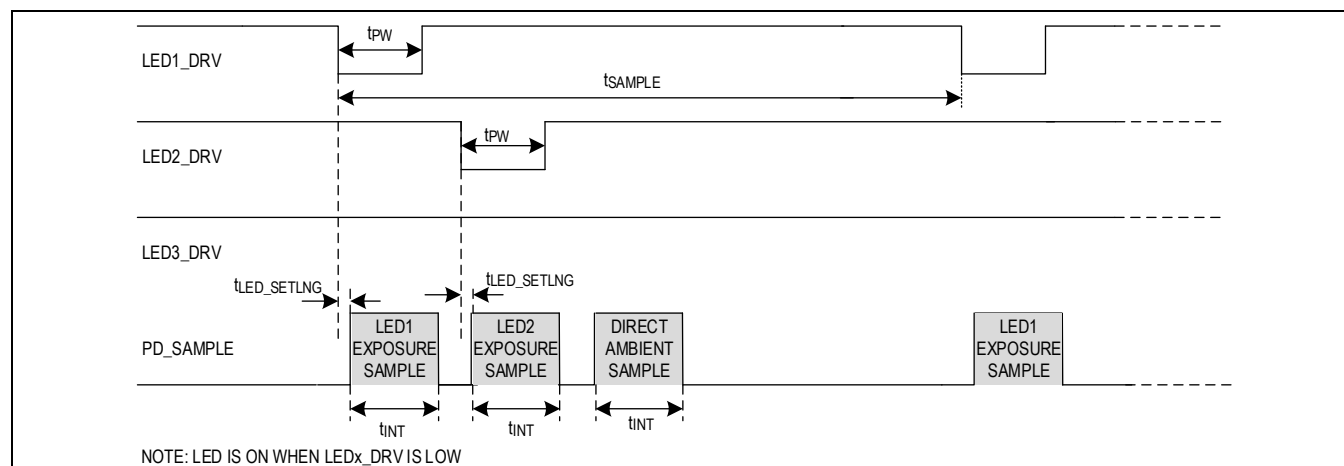
Figure 3. Timing for LED1 and LED2 Pulsing Sequentially with Direct Ambient Sampling
