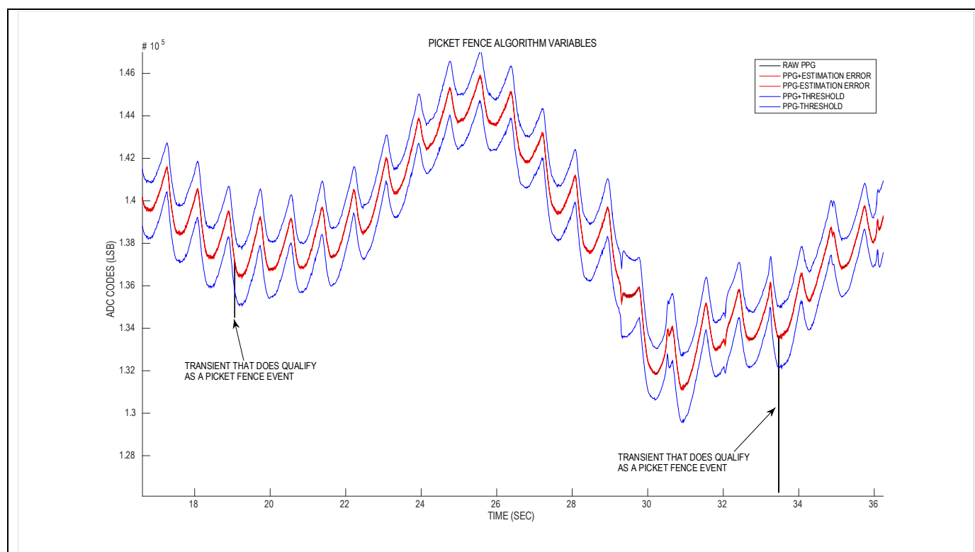
Figure 7. Picket Fences Variables in a PPG Waveform
