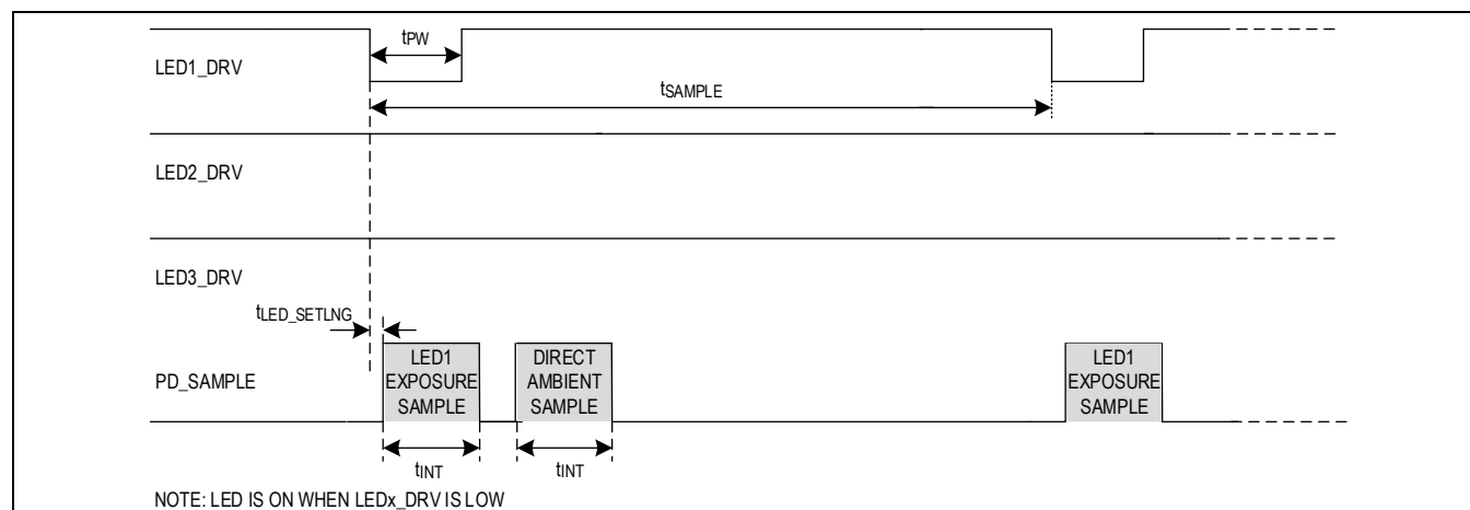
Figure 2. Timing for LED1 Pulsing with Direct Ambient Sampling
