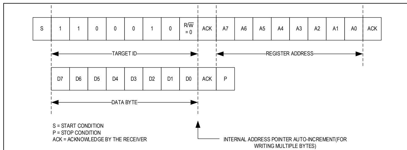
Figure 12. I 2 C Single Byte Write Transaction
