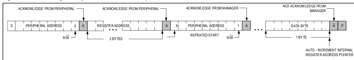
Figure 37. I 2 C Reading n-Bytes of Data from the Peripheral
