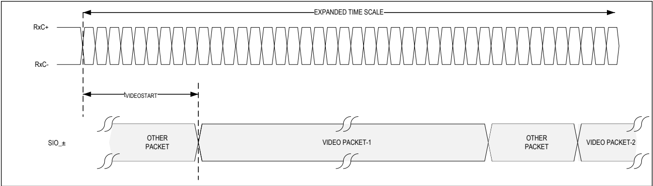
Figure 3. Video Initialization Time
