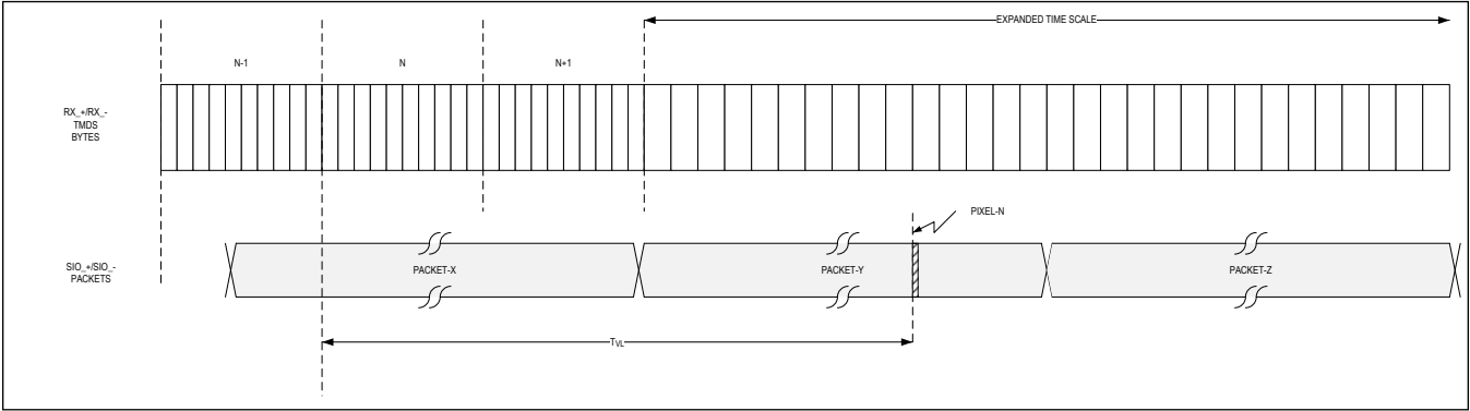
Figure 4. Video Latency
