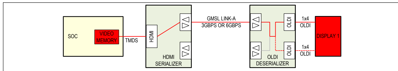
Figure 14. Single Video Stream, Single GMSL2 Link at Either 3Gbps or 6Gbps, OLDI Deserializer with Single or Dual OLDI Outputs
