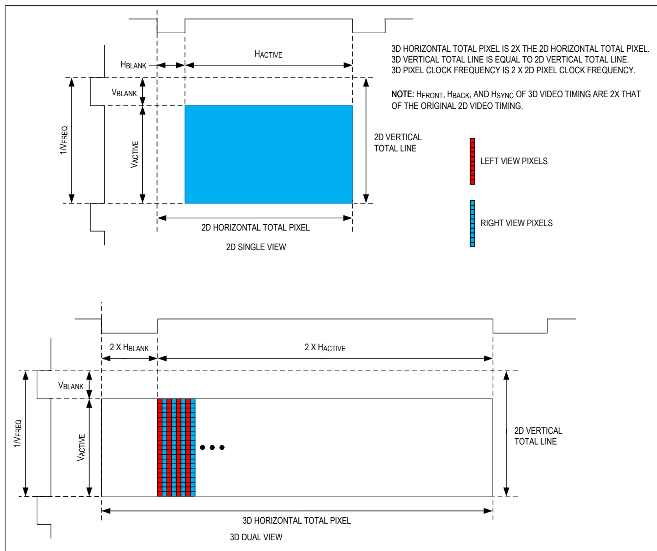
Figure 13. Dual-View Column (Pixel) Interleaved HDMI Interface Format
