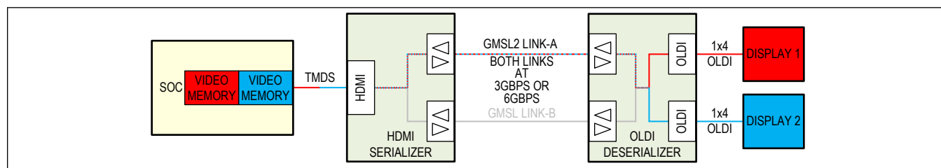
Figure 20. Serializer Dual-View Splitter Mode, Convert Dual-View to Pixel Interleave, Send Dual-Views Down Single GMSL2 Link, Dual OLDI Deserializer Splits Pixel Interleaved Dual View, Each Video Stream (View) Must Have Identical Timing, Can Also Be Done in Dual GMSL2 Link Mode
