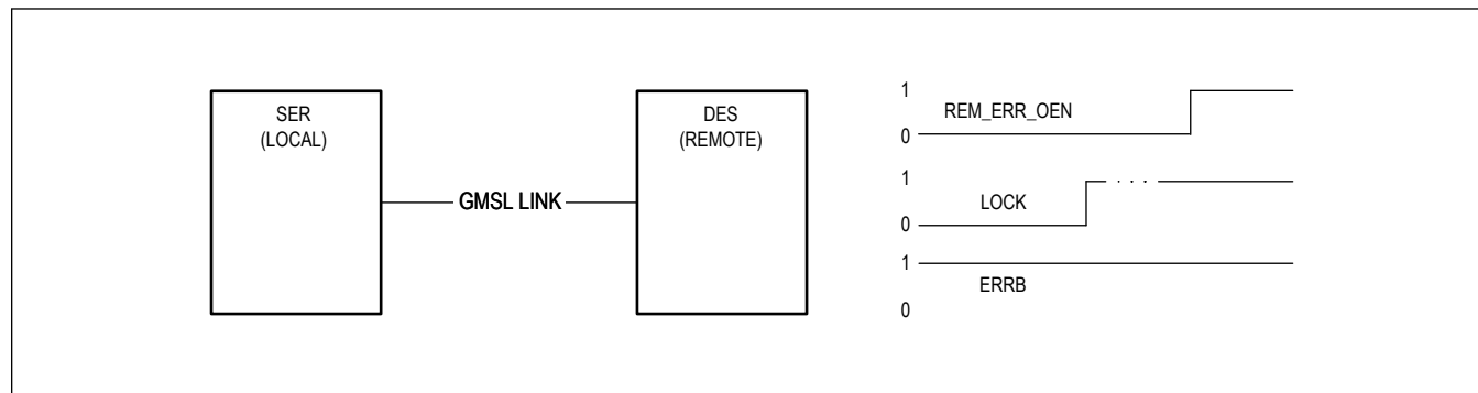
Figure 26. REM_ERR_OEN on the remote device is enabled after Link Lock
