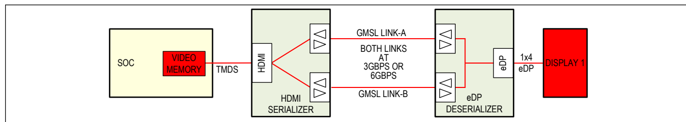
Figure 17. Single Video Stream, Dual GMSL2 Links with Both at Either 3Gbps or 6Gbps, eDP Deserializer (One, Two, or Four Lanes)
