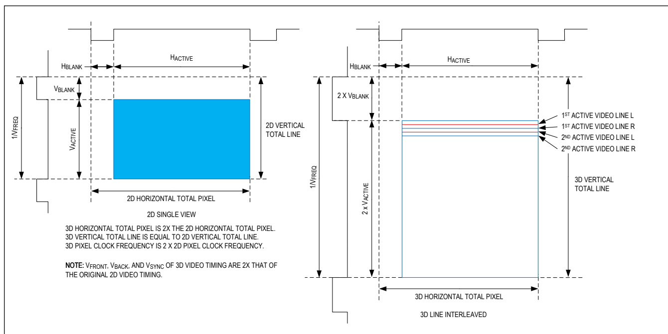
Figure 12. Dual-View Line Interleaved HDMI Interface Format
