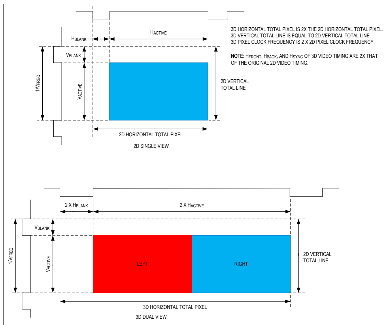
Figure 11. Dual-View Side-by-Side (Full) HDMI Interface Format
