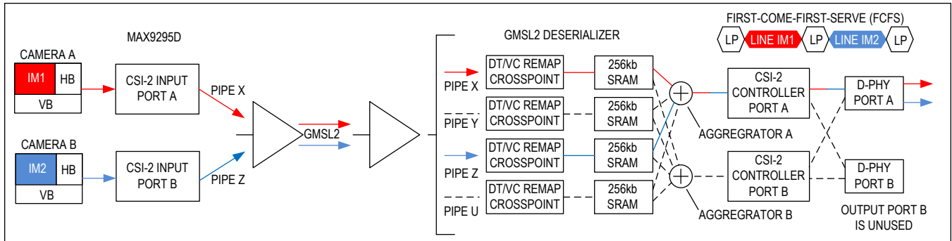
Figure 18. Deserializer Aggregation
