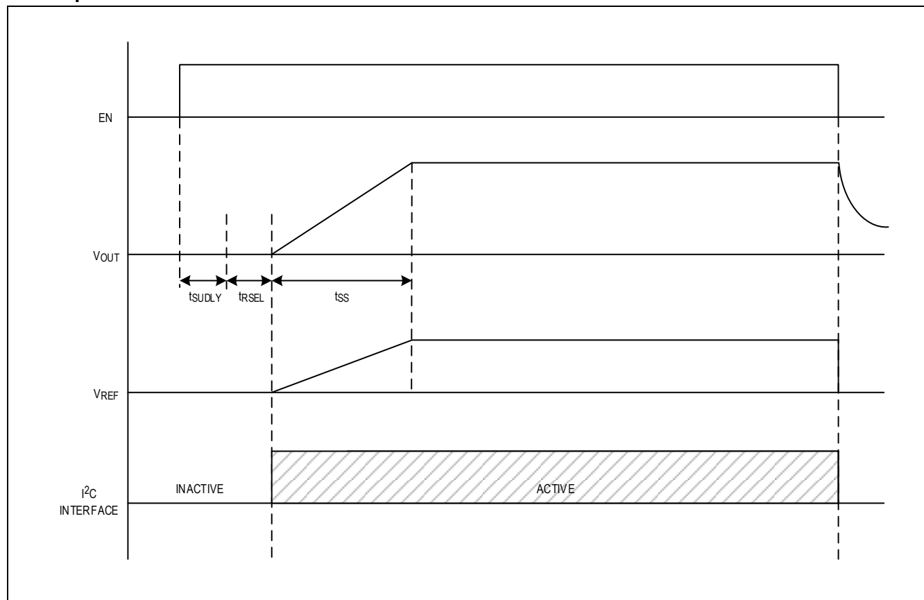
Figure 1. Start-Up Waveform
