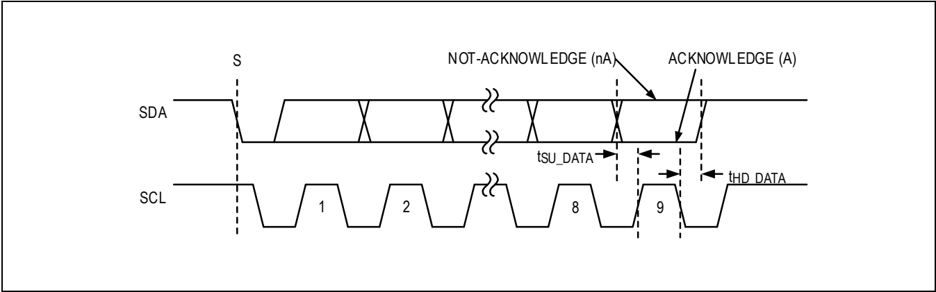
Figure 11. Acknowledge Bit
