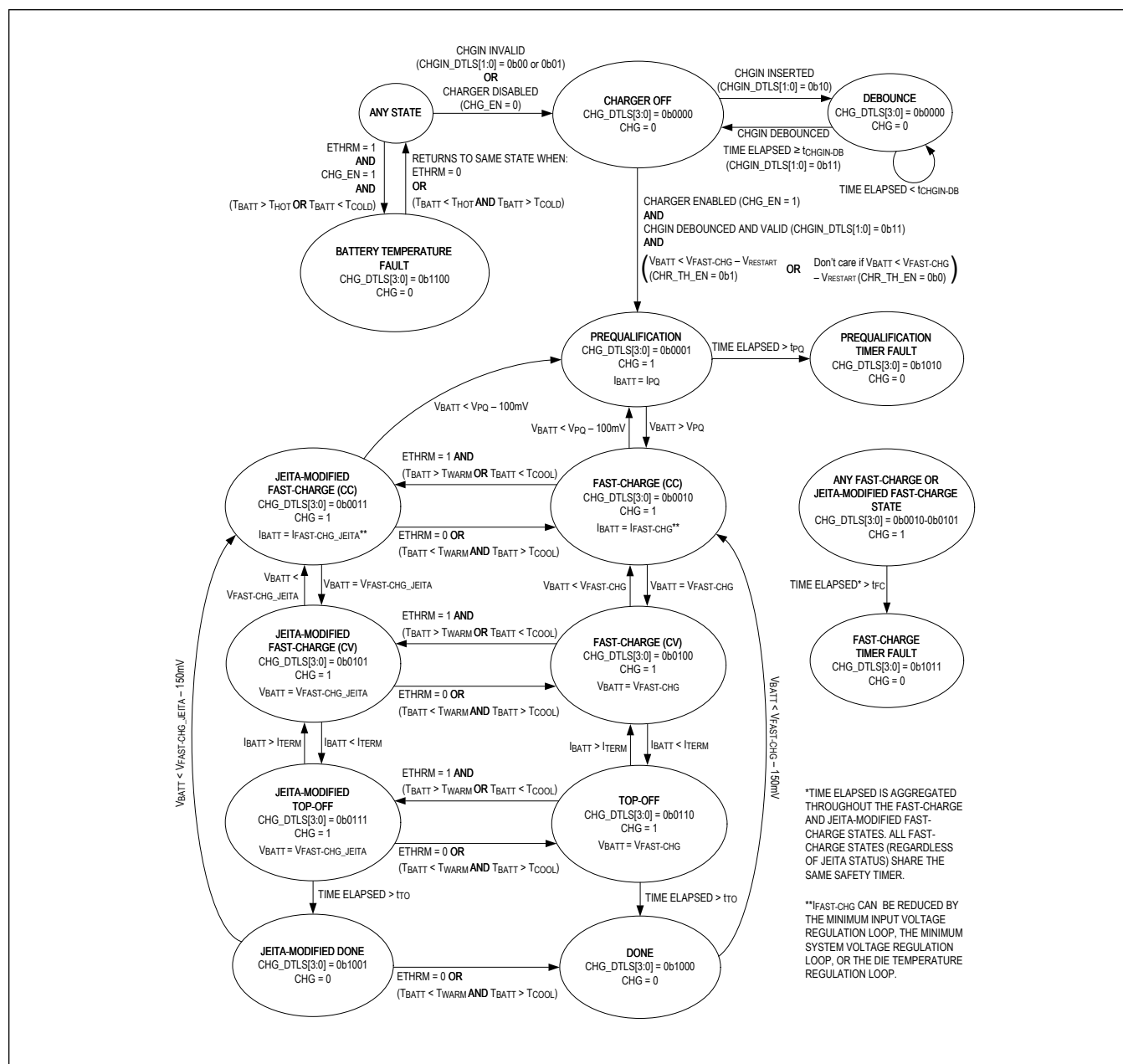
Figure 16. Charger State Machine
