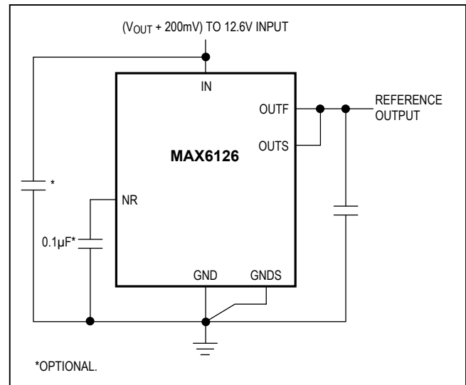
Figure 1. Noise-Reduction Capacitor
