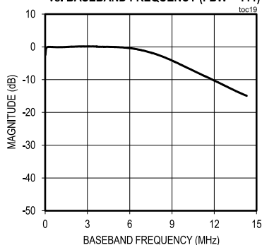
3 RD -ORDER LOWPASS FILTER RESPONSE vs. BASEBAND FREQUENCY (FBW = 111)
