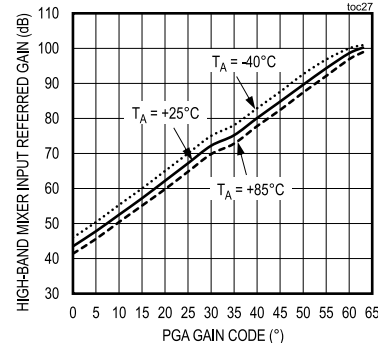
HIGH-BAND MIXER INPUT REFERRED GAIN vs. PGA GAIN CODE
