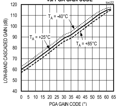
LOW-BAND CASCADED GAIN vs. PGA GAIN CODE
