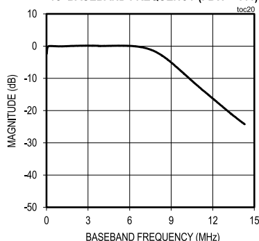
5 TH -ORDER LOWPASS FILTER RESPONSE vs. BASEBAND FREQUENCY (FBW = 111)
