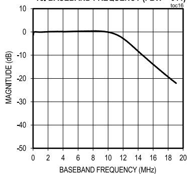
5 TH -ORDER LOWPASS FILTER RESPONSE vs. BASEBAND FREQUENCY (FBW = 011)
