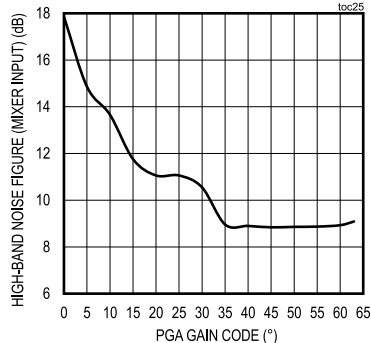
HIGH-BAND NOISE FIGURE (MIXER INPUT) vs. PGA GAIN CODE
