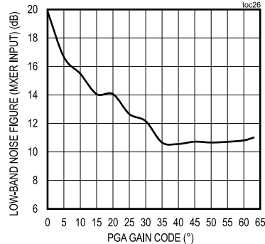
LOW-BAND NOISE FIGURE (MIXER INPUT) vs. PGA GAIN CODE
