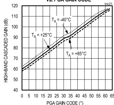
HIGH-BAND CASCADED GAIN vs. PGA GAIN CODE
