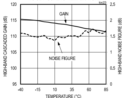
HIGH-BAND CASCADED GAIN AND NOISE FIGURE vs. TEMPERATURE
