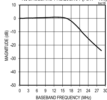
5 TH -ORDER LOWPASS FILTER RESPONSE vs. BASEBAND FREQUENCY (FBW = 100)
