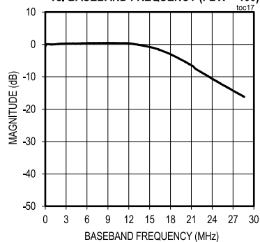
3 RD -ORDER LOWPASS FILTER RESPONSE vs. BASEBAND FREQUENCY (FBW = 100)
