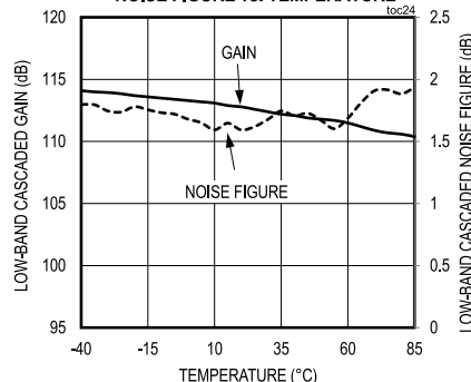
LOW-BAND CASCADED GAIN AND NOISE FIGURE vs. TEMPERATURE
