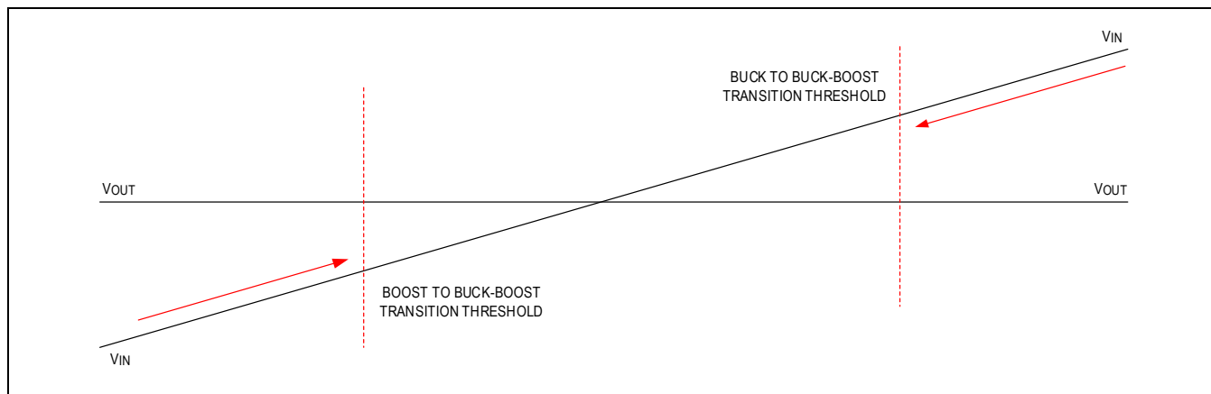
Figure 1. Input/Output Voltage at Buck-Boost Transition Boundary
