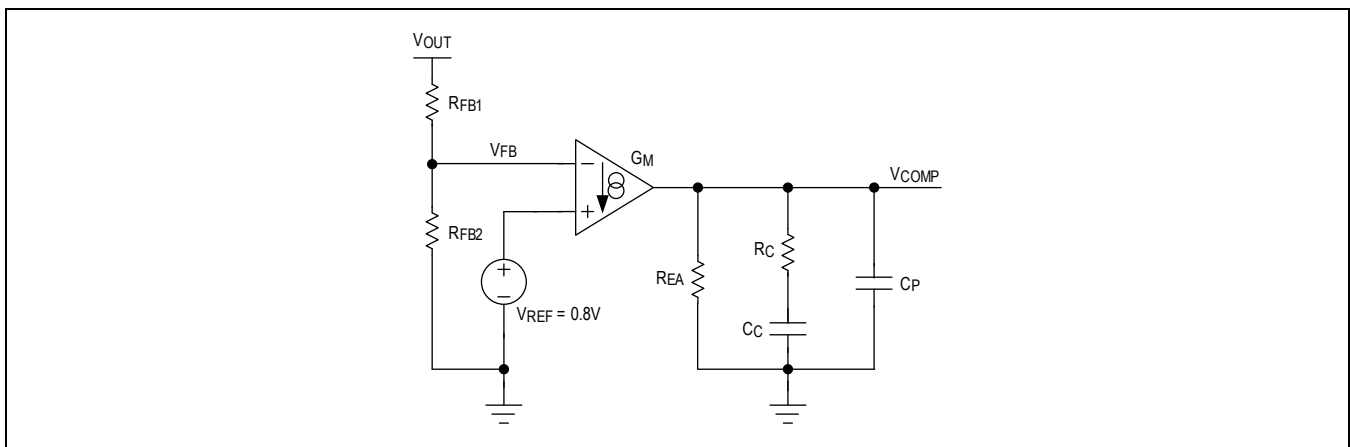
Figure 3. Compensation Network
