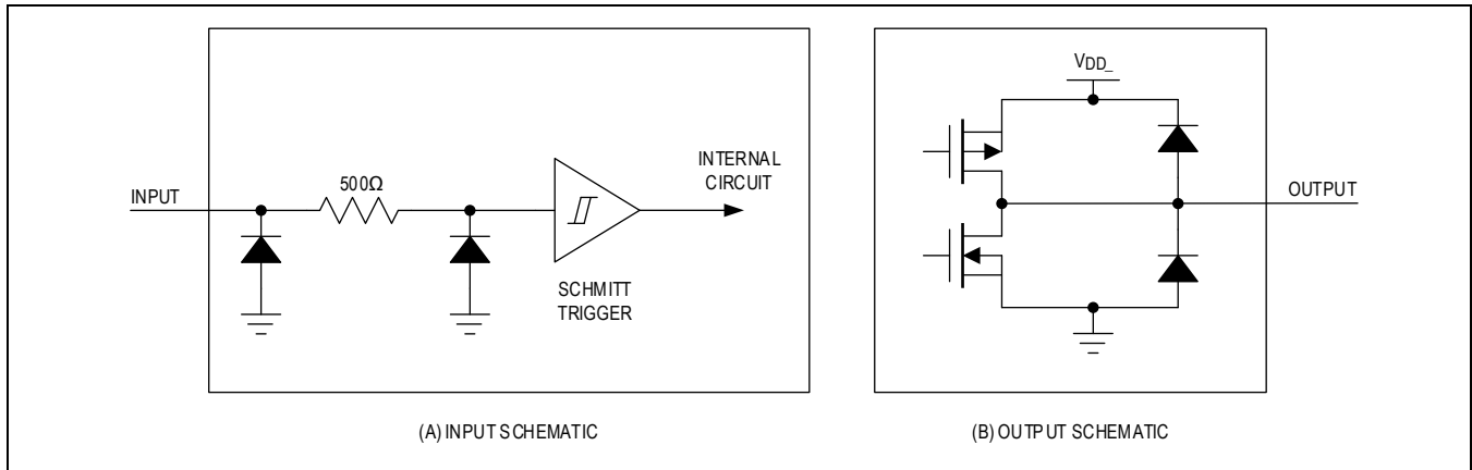
Figure 10. Device I/O Schematics
