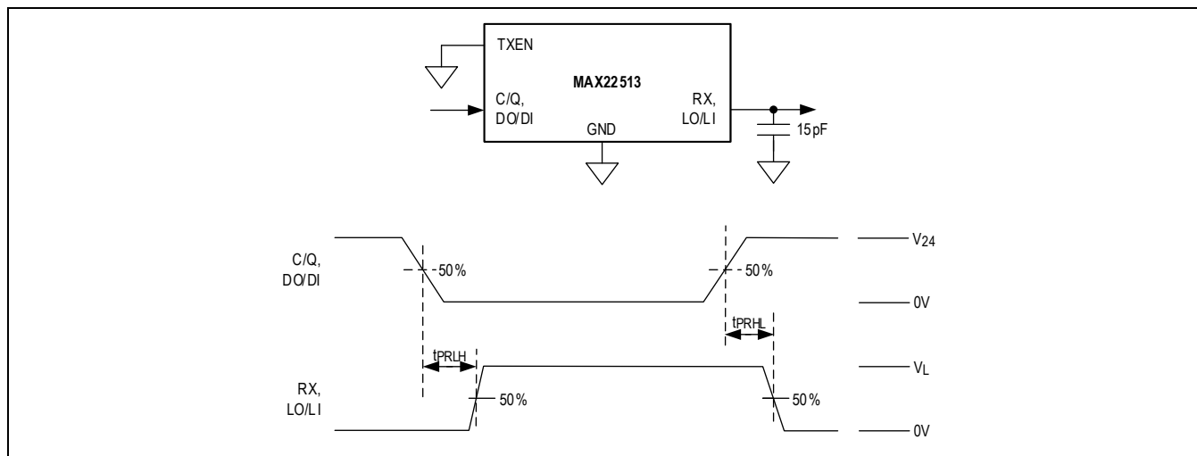
Figure 4. C/Q Receiver Timing
