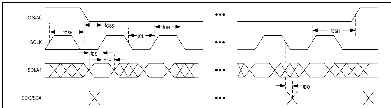
Figure 6. SPI Timing
