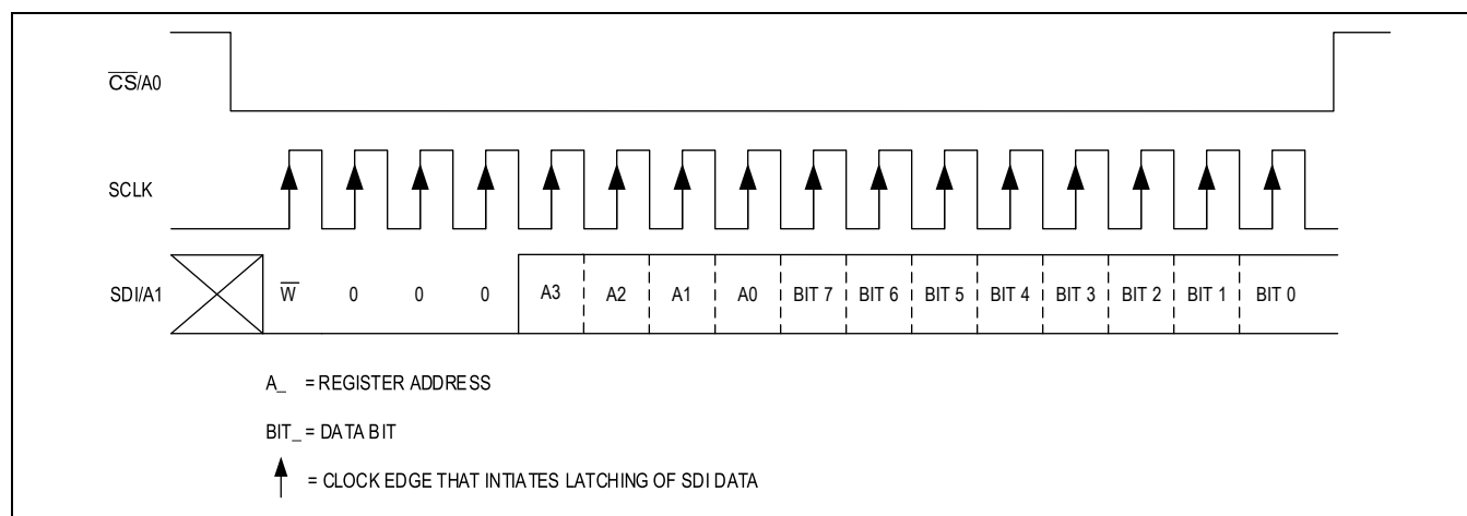
Figure 8. SPI Byte Write
