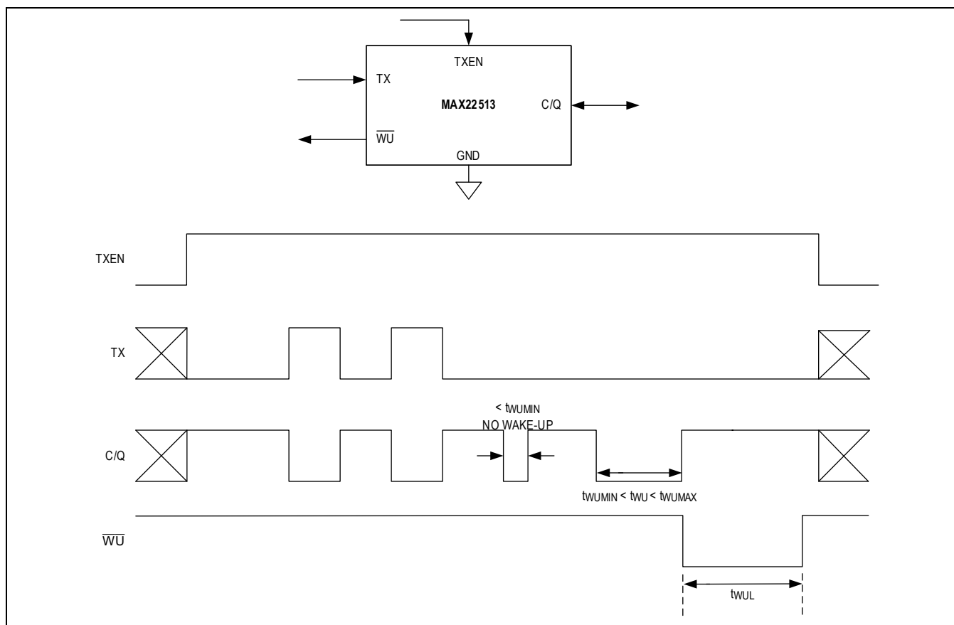
Figure 5. Wake-Up Timing
