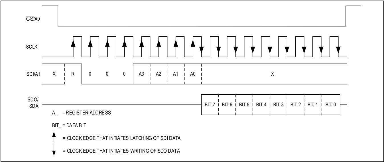
Figure 9. SPI Byte Read
