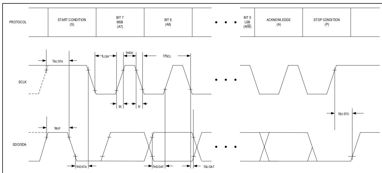
Figure 7. I²C Timing
