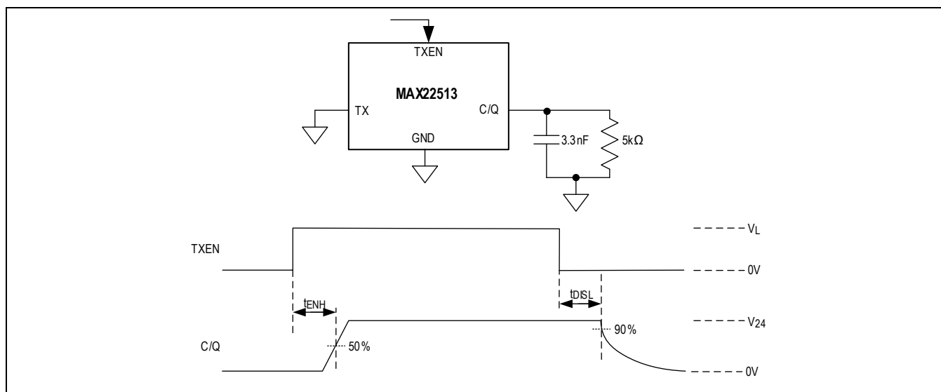
Figure 3. C/Q Driver Enable/Disable Timing
