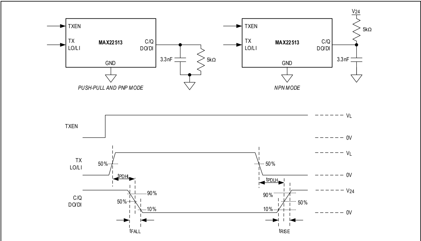
Figure 1. C/Q and DO/DI Driver Propagation Delays
