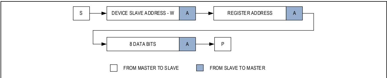
Figure 11. I 2 C Byte Write
