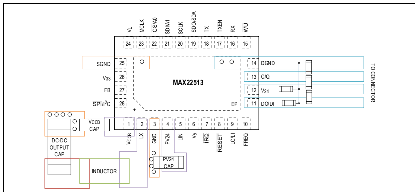
Figure 13. Sample Grounding Scheme (TQFN Package)
