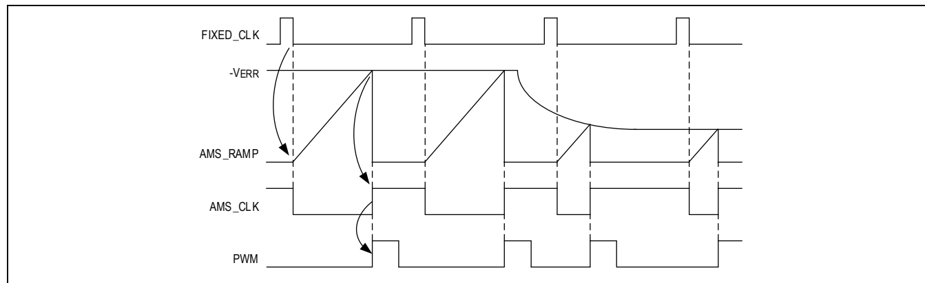
Figure 2. AMS Operation
