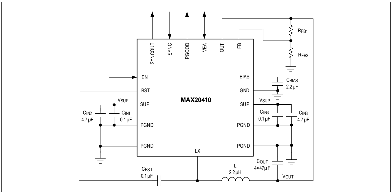
MAX20410 Configuration: 400kHz, 10A, Adjustable Output Voltage
