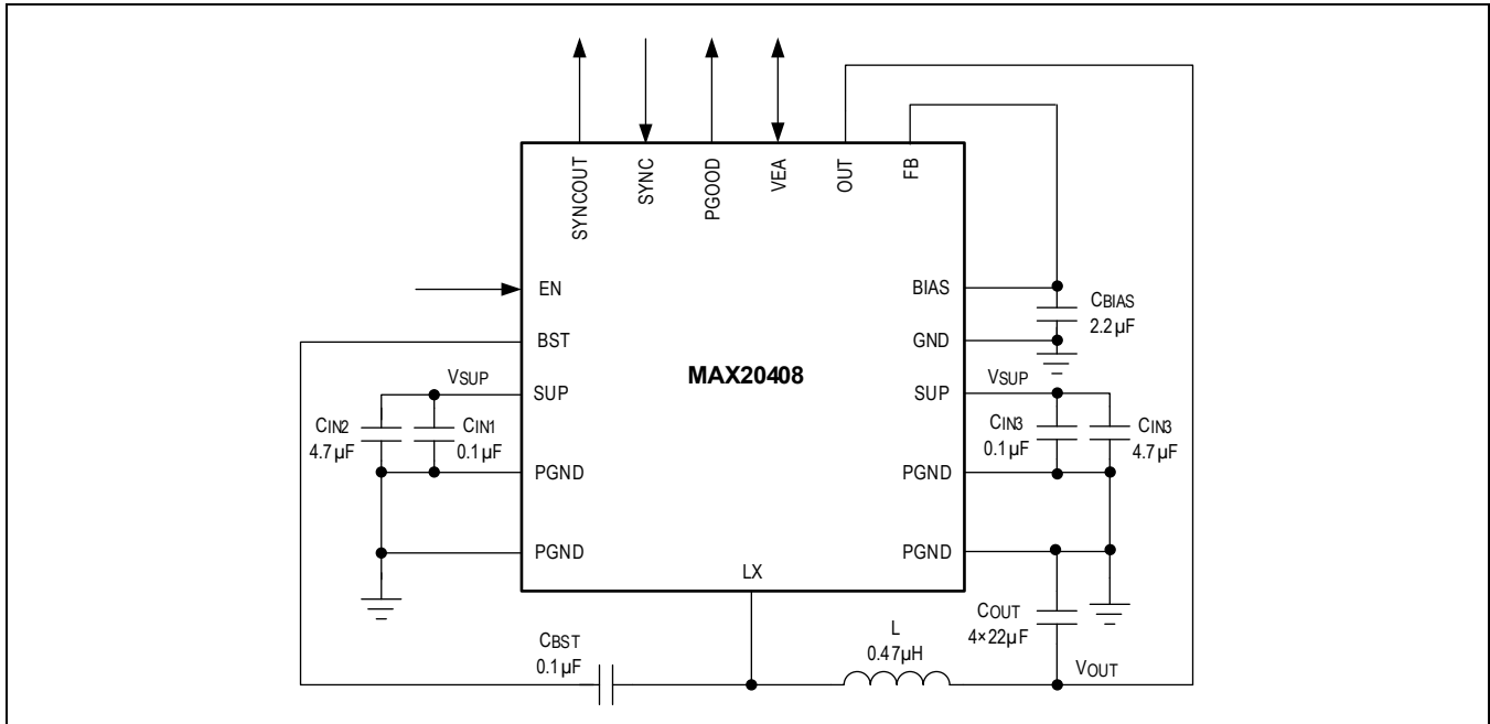
MAX20408 Configuration: 2.1MHz, 8A, Fixed Output Voltage
