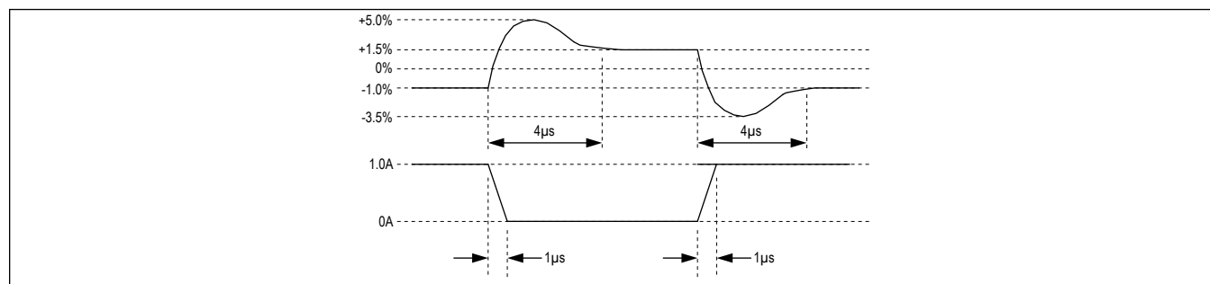
Figure 1. Load-Transient Response
