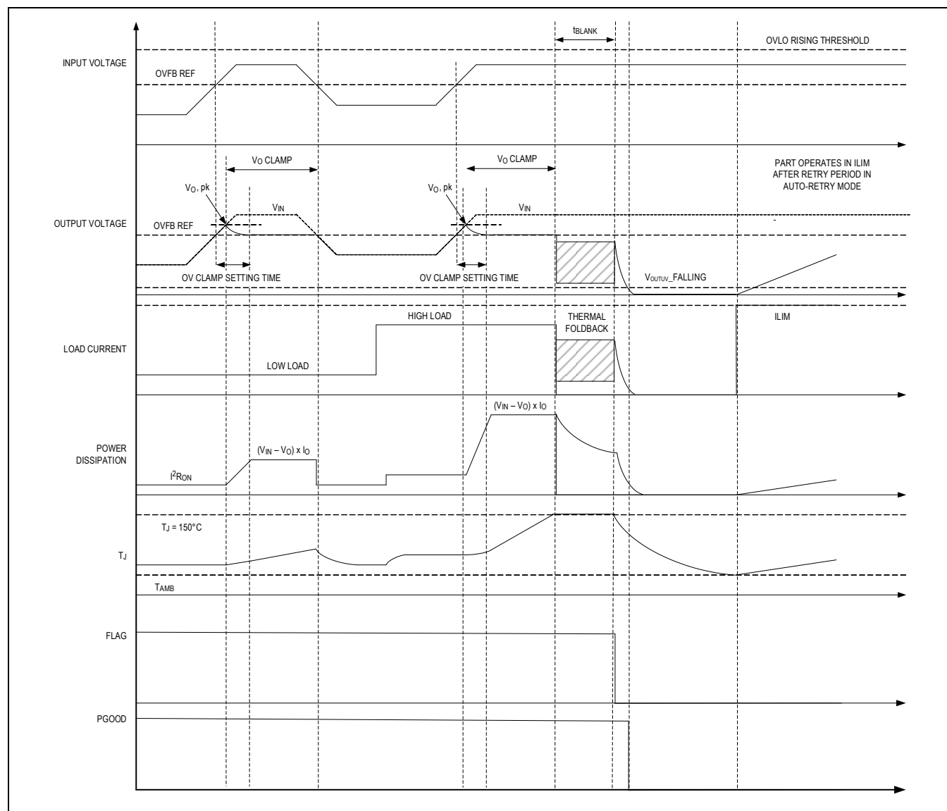
Figure 19. Overvoltage Clamp Operation and Recovery
