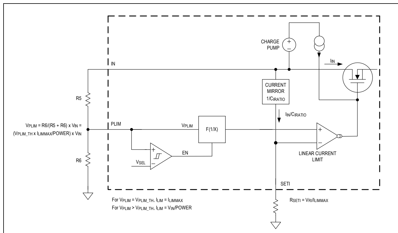
Figure 28. Power Limit Circuit
