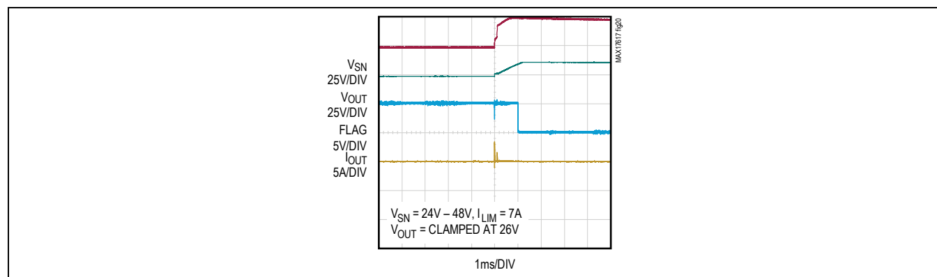
Figure 20. Overvoltage Clamp Response
