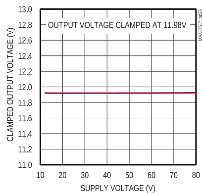
CLAMPED OUTPUT VOLTAGE vs. SUPPLY VOLTAGE
