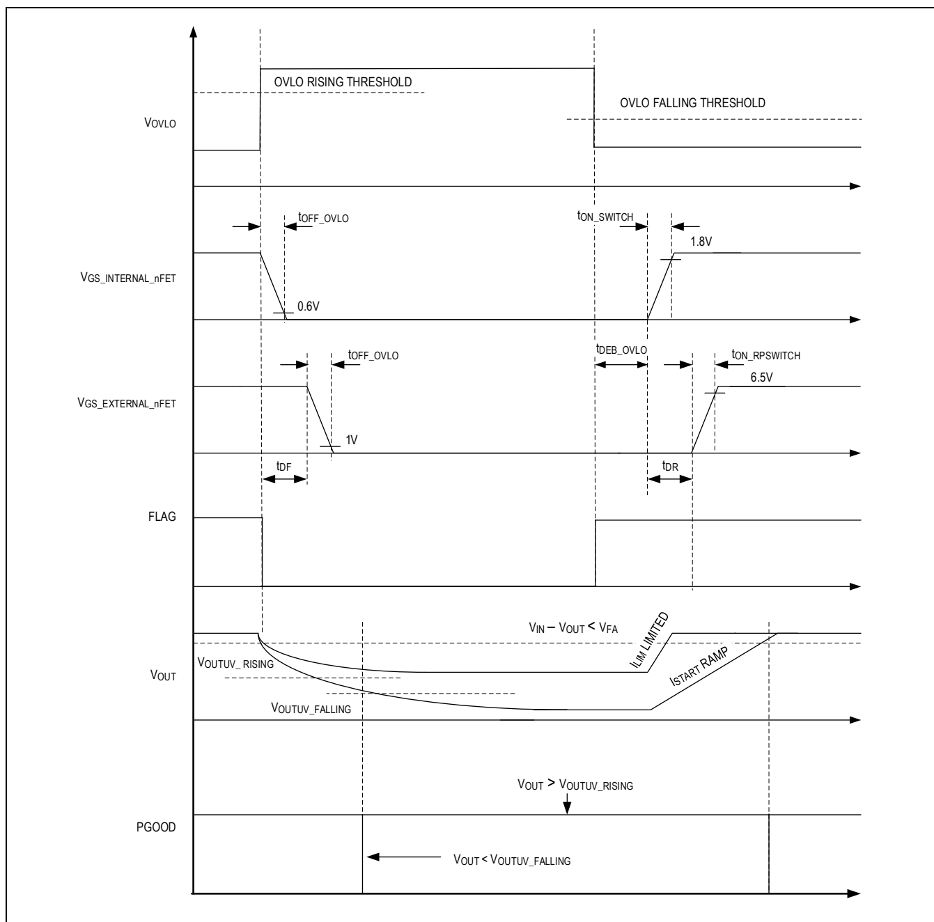
Figure 6. Input Overvoltage Fault Timing Diagram
