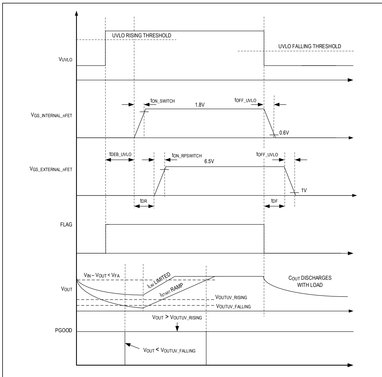
Figure 4. Input Undervoltage Fault Timing Diagram
