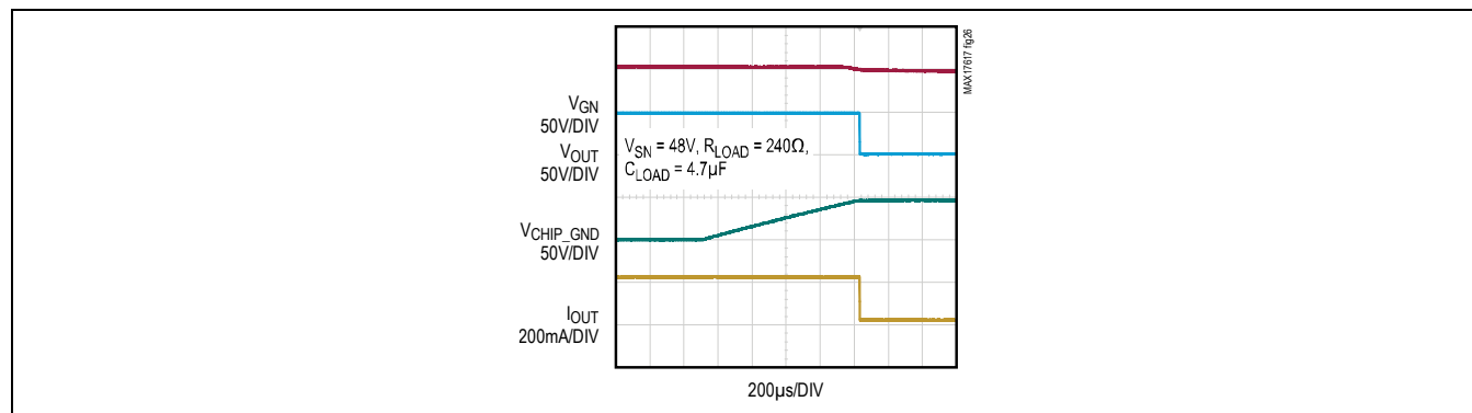
Figure 26. Load Current Interruption During a Loss of Ground Event
