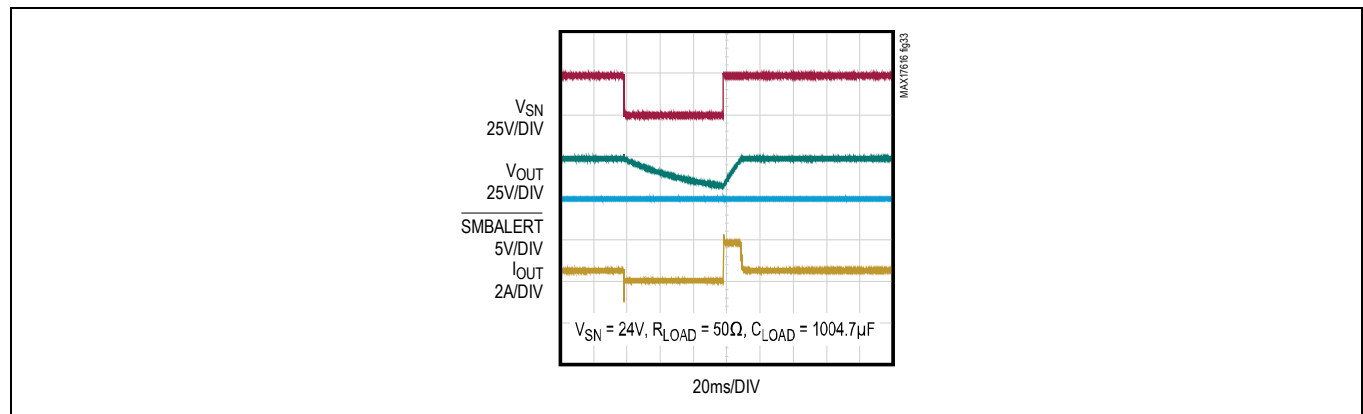
Figure 33. Voltage Interruption Response
