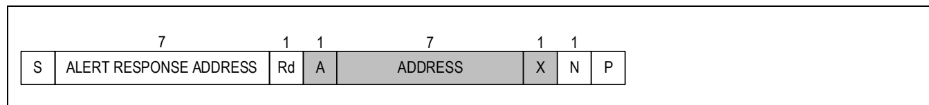
Figure 31. A 7-Bit Addressable Device Response to an ARA
