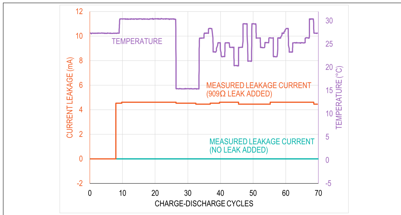
Figure 11. Example of Internal Self-Discharge with Temperature Variation
