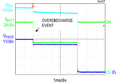
OVERDISCHARGE CURRENT PROTECTION ( I_{\text{ODCP}} = 4\text{A}/5\text{ms DELAY} )
