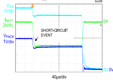
SHORT-CIRCUIT PROTECTION ( I_{\text{SCCP}} = 5\text{A}/253\mu\text{s DELAY} )
