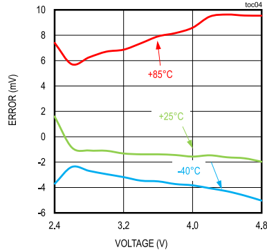
CELL VOLTAGE ADC ERROR
