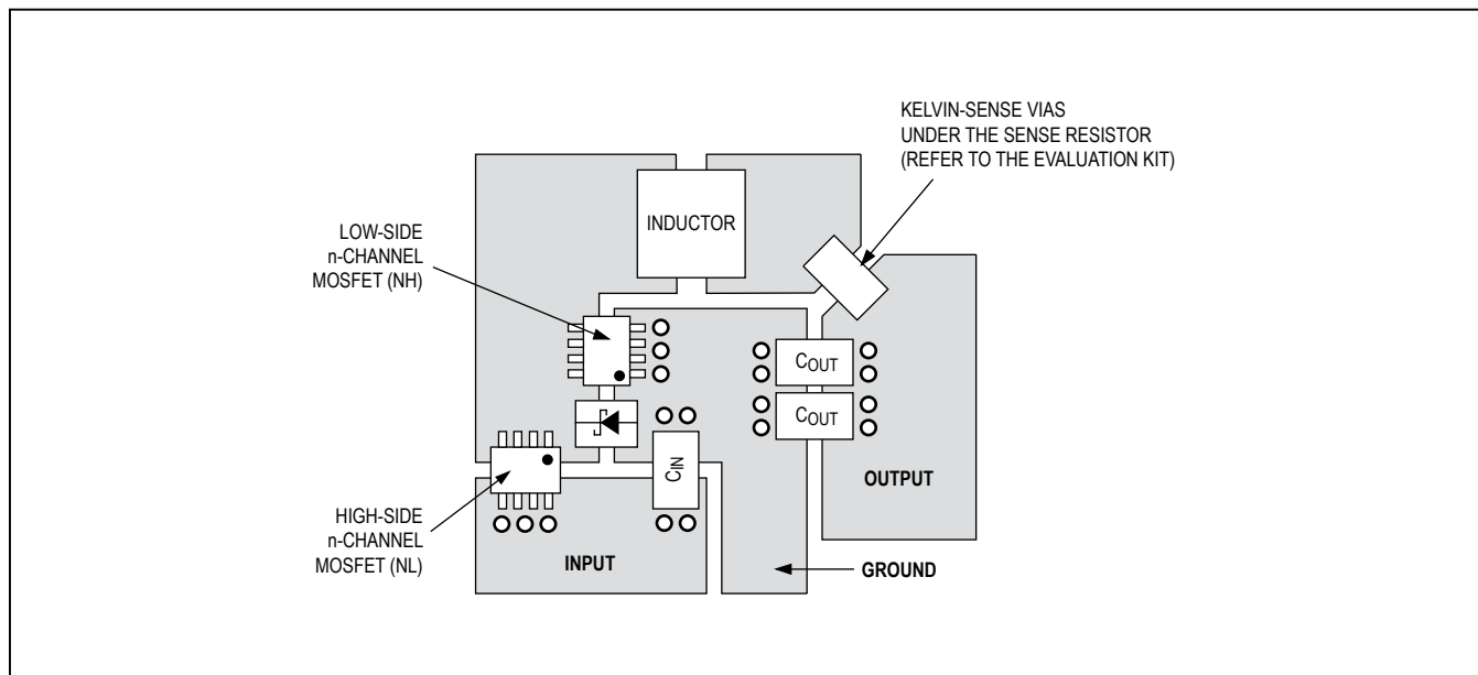
Figure 3. Layout Example
