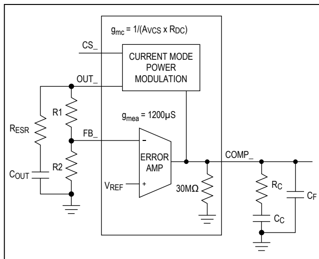
Figure 2. Compensation Network
