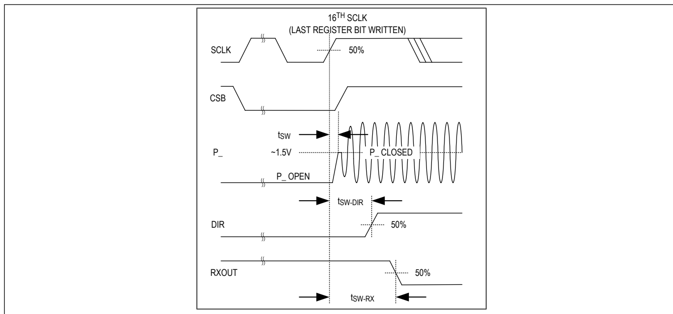
Figure 3. Switch Timing
