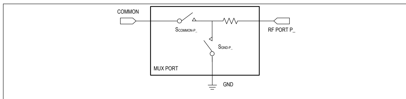
Figure 2. MUX Port Diagram
