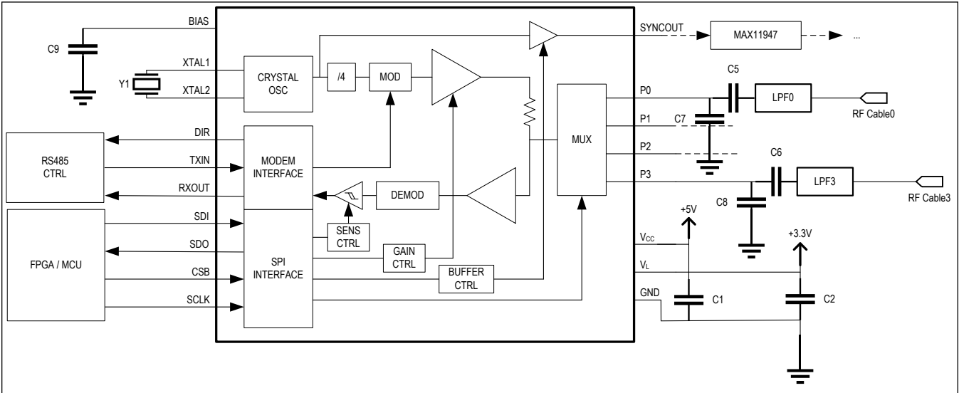
Circuit 1
