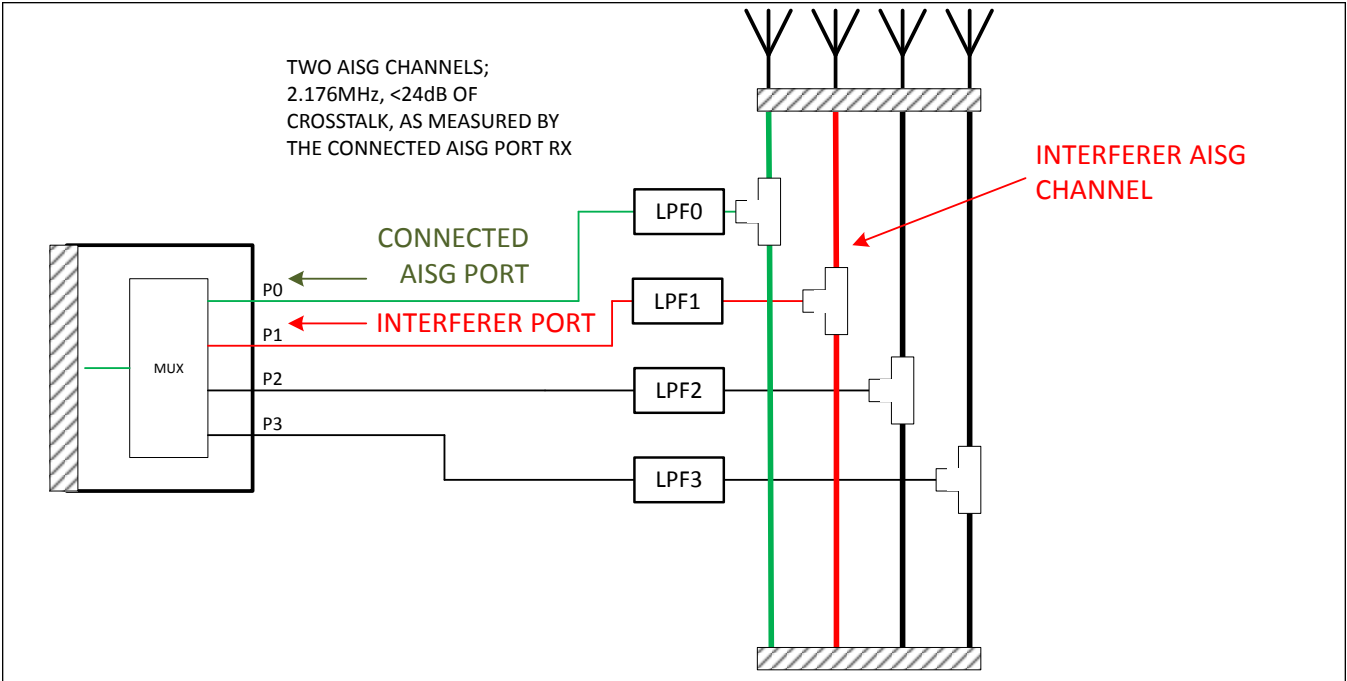
Figure 6. Modem Crosstalk
