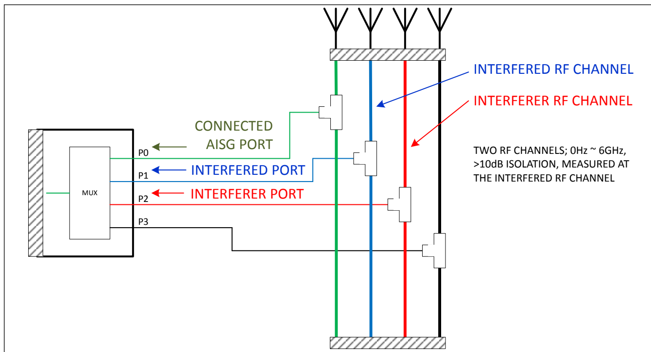
Figure 4. RF Isolation
